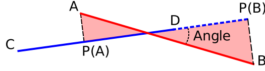
Figure 6.10: Distance between two lines segment. Here the overlap is \mathcal{R}(P(AB), CD) = \frac{|P(A)D|}{|P(B)C|} .
