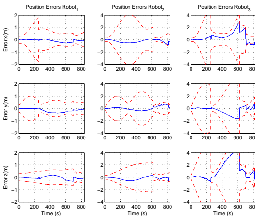
(b) Position Errors r_1 , r_2 and r_3
