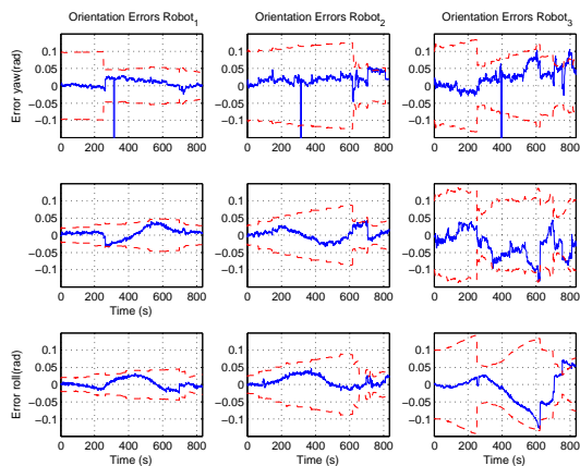
(c) Orientation Errors r_1 , r_2 and r_3
