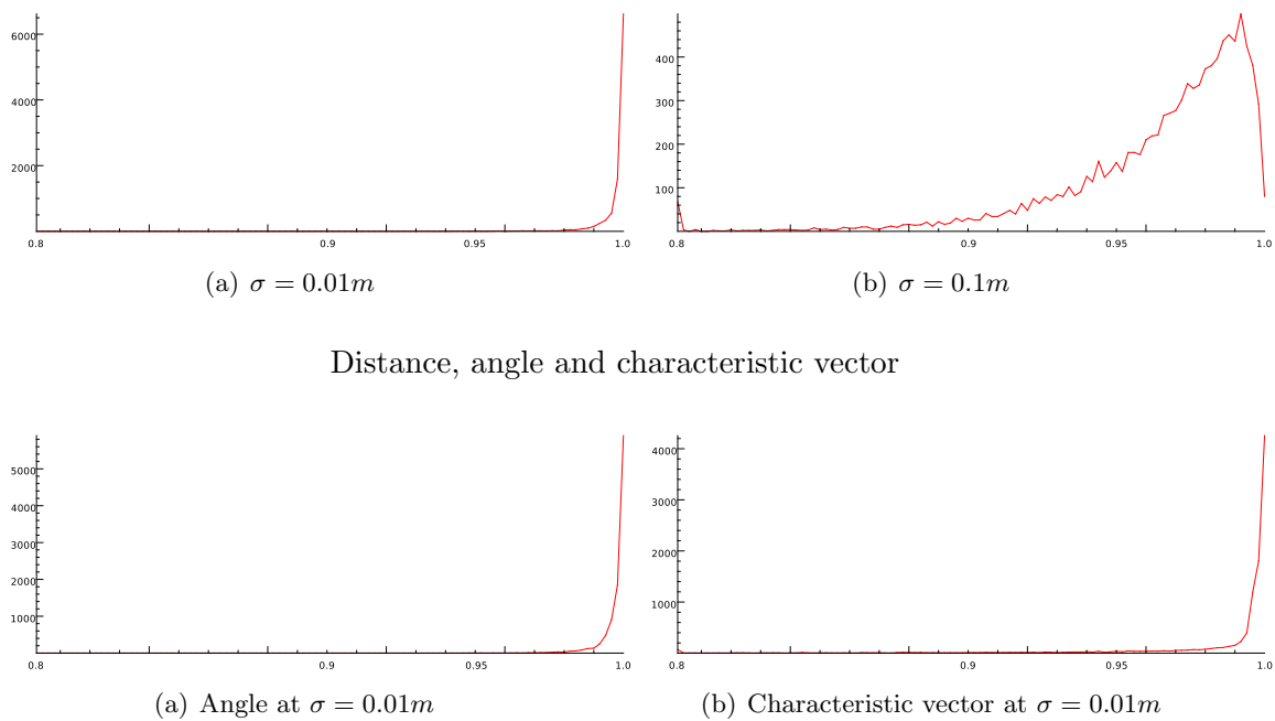
Figure 9.14: Robustness to noise, the interval for the correlation is [0.8; 1.0]
