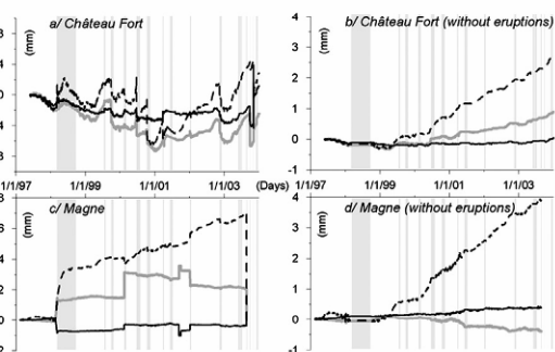
Figure 3. (a, c) Extensometer displacements recorded during 1997 to 2003 on the opening (black indents), shear (grey lines) and vertical (black lines) components. An increase of the values corresponds to an opening, a dextral movement or an uplift of the East side of the fracture, respectively. Grey areas represent periods of eruptions. (b, d) Same displacements as above without the short-term ground deformations due to dyke injections.
