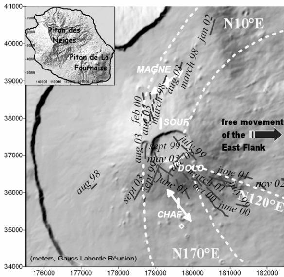
Figure 1. Structural map of Piton de la Fournaise. The rift zones are limited by dashed white lines. The solid white lines, black lines, and diamonds indicate respectively the location of the extensometers, the eruptive fissures from 1998 to 2003, and the CHAF tiltmeter station.
