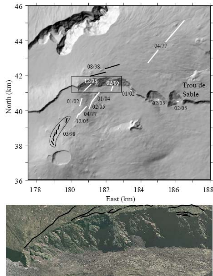
Fig. 14. Top: Location of the April 1977 and the post-1997 eruptive fissures that have propagated in Plaine des Osmondés or outside Enclos Fouqué. The white lines show the eruptive fissures that emitted olivine-rich lavas. The black lines show the eruptive fissures that emitted common aphyric basalt. The dates are month/year. All the fissures that opened in 1998 are related to the same eruption, the opening in 08/98 corresponding to a late propagation of the dyke (Bachelery, 1999). Bottom: Aerial photo of August 2003 (IGN) showing the western part of the scarp above Plaine des Osmondés. In black are the fractures visible on the photography.
