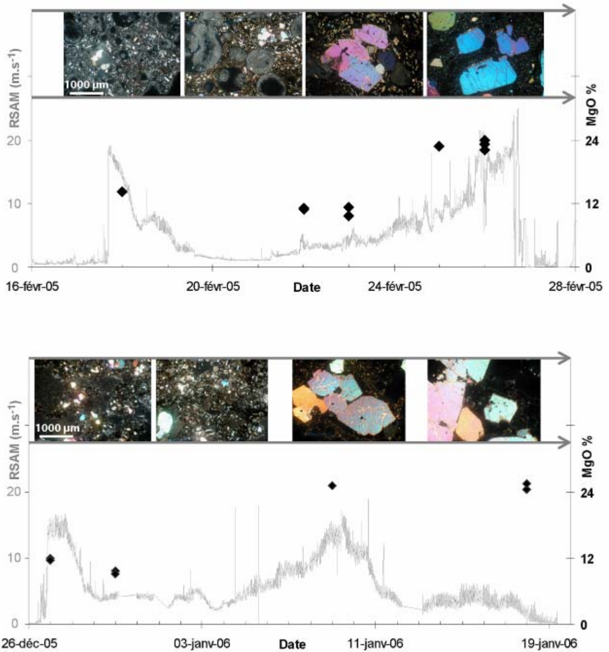
Fig. 8: Curves of the RSAM (Real-time Seismic-Amplitude Measurement) evolution at NSR seismic station during the two oceanite eruptions of February 2005 (a) and December 2005 (b) compared with the evolution of the MgO% of the lavas (black squares) and the evolution of their mineral composition (photography).
