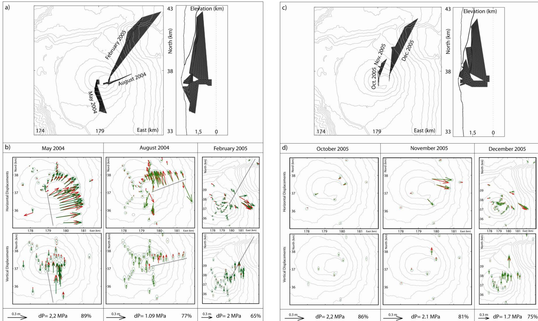
Fig. 5: (a) Geometry of the dykes modelled for the May 2004, August 2004 and February 2005 eruptions (Gauss Laborde Reunion map coordinates), and (b) comparison between observed (green) and calculated (red) ground displacements. (c) Geometry of the dykes modelled for the October 2005, November 2005 and December 2005 eruptions (Gauss Laborde Reunion map coordinates), and (d) comparison between observed (green) and calculated (red) ground displacements.
