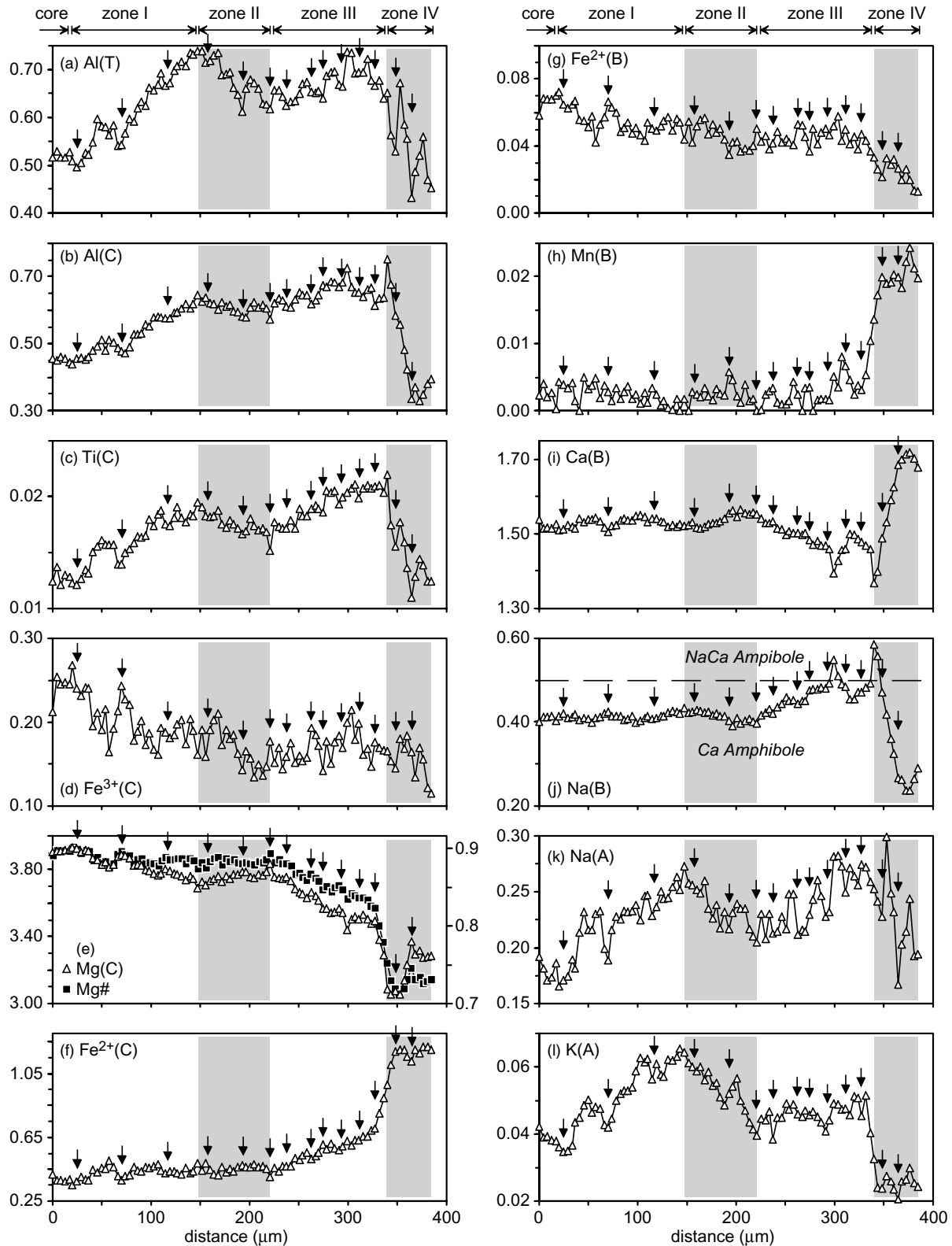
Fig. 6. Detailed core to rim profile (probe step: 4 \mu\text{m} ) of amphibole porphyroblast shown in Fig. 5. Note that zoning includes large-range (zones I-IV) and short range oscillations (arrows define decrease in Al(C) and/or Al(T)).
