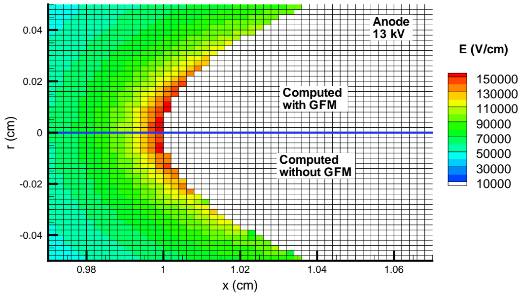
Figure IV.7: Comparison between the magnitude of the electric field computed with and without the GFM in the same point-to-plane configuration as in Figure IV.4. The white region of the color scale corresponds to the hyperboloid anode. In the case without the GFM, all the potentials V_{i,j} are set equal to V_a if the point (i,j) is inside the electrode. In the case with GFM, the nodes inside the electrode are also set to V_a , except for the points close to the interface.
