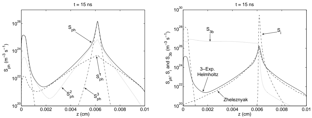
Figure III.16: Photoionization production rate S_{ph} at t = 15 ns along the symmetry axis of the computational domain. (a) S_{ph} and the three components S_{ph}^1 , S_{ph}^2 , and S_{ph}^3 of the three-exponential Helmholtz model. (b) S_{ph} calculated using the three-exponential Helmholtz and Zheleznyak models, electron impact ionization production rate S_i , and three-body electron attachment rate S_{3b} .
