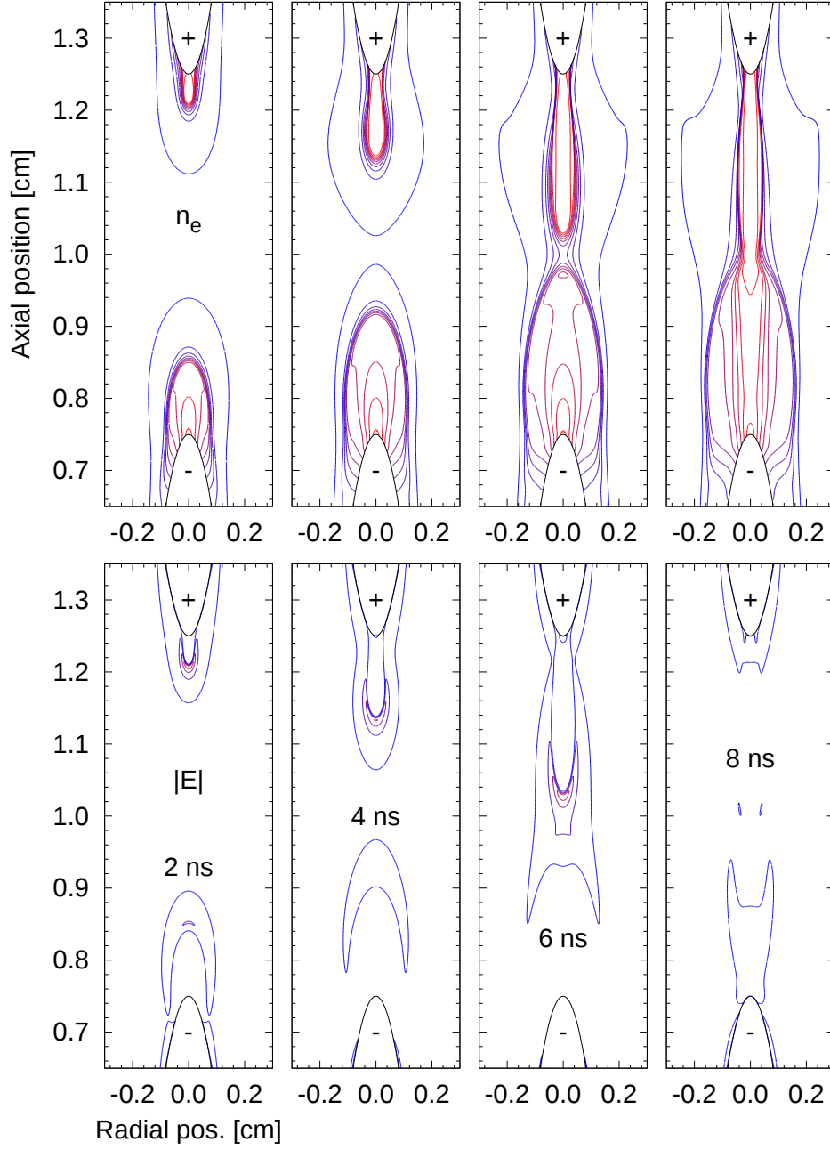
Figure IV.15: Point-to-point geometry: Two-dimensional isocontours of the electron density and the magnitude of the electric field at t = 2, 4, 6 , and 8 ns. For the electron density the isocontours vary from 10^9 to 10^{13.5} \text{ cm}^{-3} , with a multiplier step of 10^{0.5} \text{ cm}^{-3} . For the electric field the isocontours vary from 30 to 150 \text{ kV/cm} , with a step of 30 \text{ kV/cm} . In this case T = 300 \text{ K} and V_a = 13 \text{ kV} .
