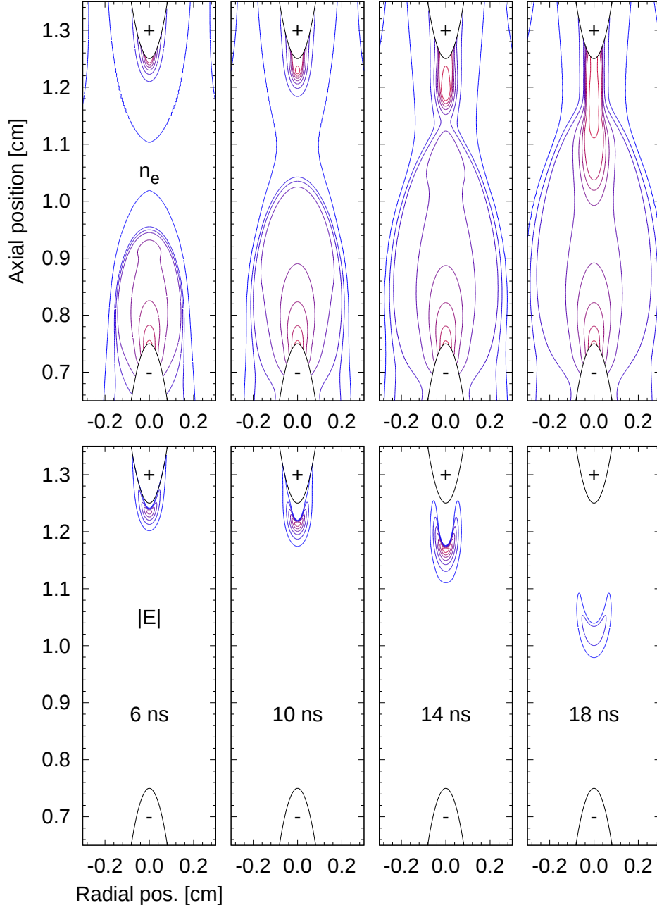
Figure IV.16: Point-to-point geometry: Two-dimensional isocontours of the electron density and the magnitude of the electric field at t = 6, 10, 14, and 18 ns. For the electron density the isocontours vary from 10^9 to 10^{13.5} \text{cm}^{-3} , with a multiplier step of 10^{0.5} \text{cm}^{-3} . For the electric field the isocontours vary from 10 to 30 kV/cm, with a step of 2.5 kV/cm. In this case T = 1800 K and V_a = 3 kV.
