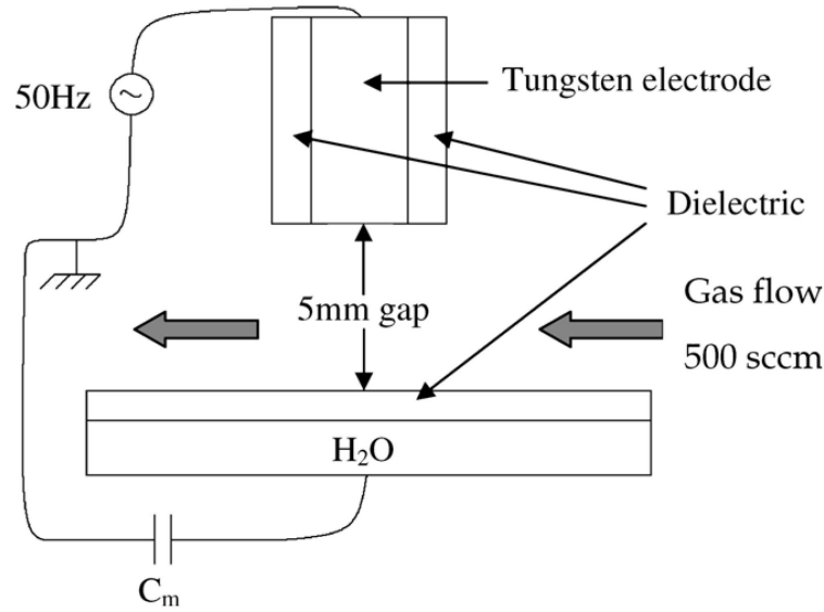
Figure V.1: Scheme of the reactor.
