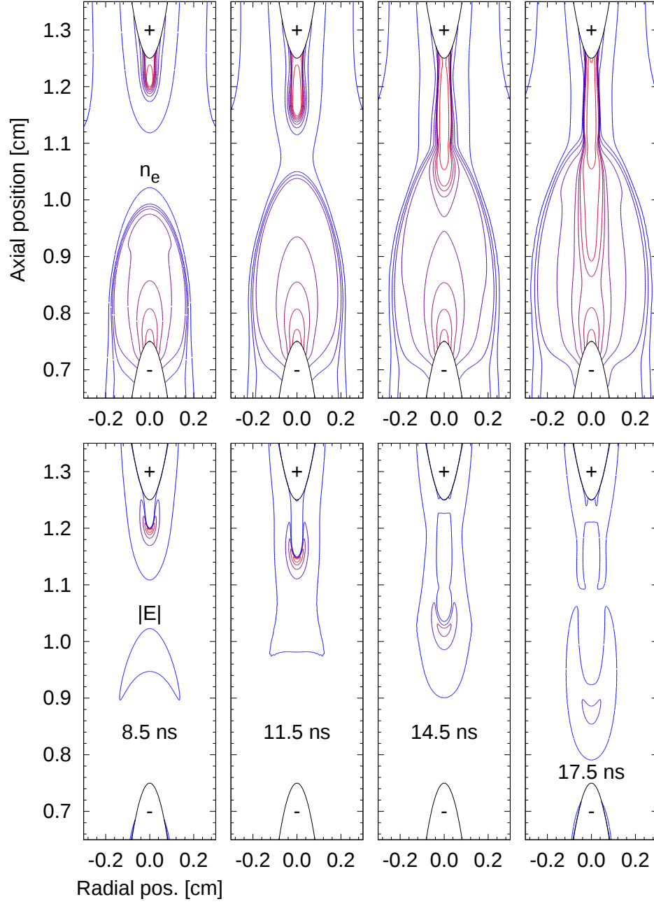
Figure IV.13: Point-to-point geometry: Two-dimensional isocontours of the electron density and the magnitude of the electric field at t = 8.5, 11.5, 14.5 , and 17.5 ns. For the electron density the isocontours vary from 10^9 to 10^{13.5} \text{ cm}^{-3} , with a multiplier step of 10^{0.5} \text{ cm}^{-3} . For the electric field, the isocontour vary from 10 to 50 kV/cm, with a step of 10 kV/cm. In this case T = 1000 \text{ K} and V_a = 5 \text{ kV} .
