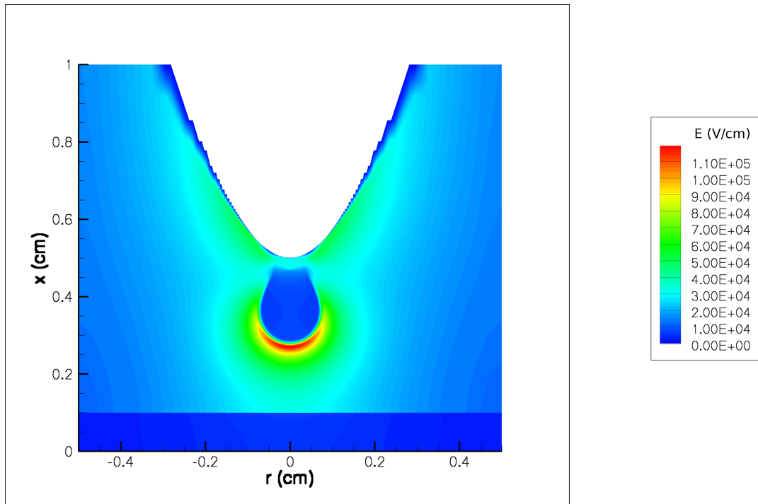
Figure VI.6: Cross-sectional view of the distribution of the magnitude of the electric field at t = 3 \text{ ns} . The white area represents the anode.
