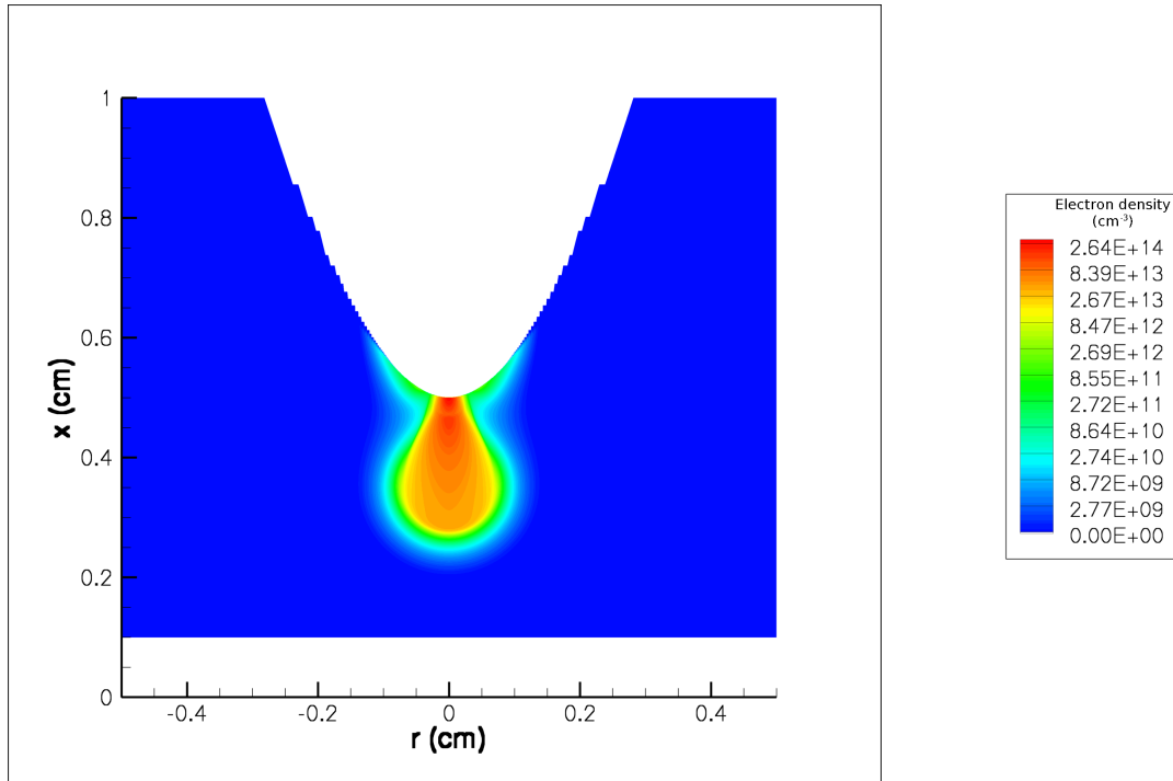
Figure VI.5: Cross-sectional view of the distribution of the electron density at t = 3 \text{ ns} . The white areas represent the anode and the dielectric material.
