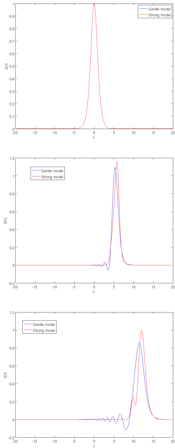
Figure 4.3.1: Solution of Camassa-Holm equation for a sinusoidal bottom, with gentle or strong model for t = 0 , t = 6.67 , t = 13.33 . ( c_1 = 0.5 \beta = 0.5 , \varepsilon = \mu = 0.1 \alpha = 0.05 )
