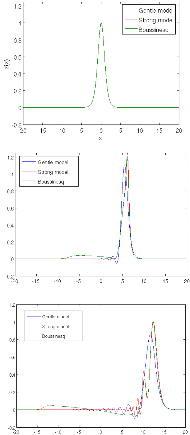
Figure 4.2.1: Solution of KdV equation for a sinusoidal bottom, with gentle, strong model and Boussinesq model, for t = 0 , t = 6.67 , t = 13.33 . ( c_1 = 0.5 \beta = 0.5 , \varepsilon = \mu = 0.1 \alpha = 0.05 )
