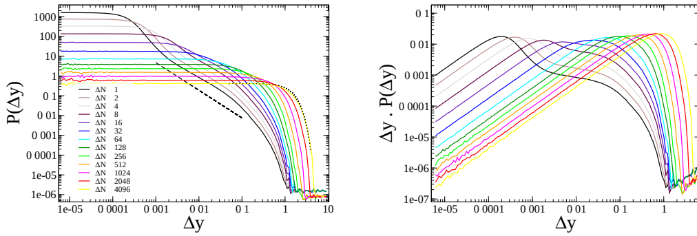
FIG. 5.15 : Left : Distribution P(\Delta y, \Delta N) of distances \Delta y after \Delta N steps of incremental strain imposed at the top rigid wall. Each step \Delta N = 1 corresponds to a elementary strain of \delta\varepsilon = 0.005\% . The dashed line correspond to the power law P(\Delta y) \propto \Delta y^{-1.4} . The dotted line correspond to a Gaussian fit. Right : Same distributions but multiplied by the distance \Delta y itself. These function correspond to the van Hove functions. The position of the peak appearing at large \Delta N evolves in a diffuse manner.
