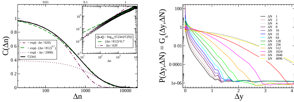
FIG. 5.12 : Left : Autocorrelation function of the shear stress computed on each particle and averaged over the whole sample, as a function of time (applied shear strain). The nature of the fits is indicated in the legend box. Inset : Logarithm of the autocorrelation function of the shear stress, in log-log scale, in order to determine the exponent of the corresponding stretched exponential. Right : Probability distribution function P(\Delta y, \Delta N) or equivalently van Hove function G_s(\Delta y, \Delta N) of the transverse displacement \Delta y for \Delta N = 1, 2, 4, 8, 16, 32, 64, \dots . The log-lin scale illustrates the deviation from the Fickian behavior and the exponential tail of the distributions. The dotted line is a Gaussian fit for large \Delta N where the Fickian behavior is recovered.
