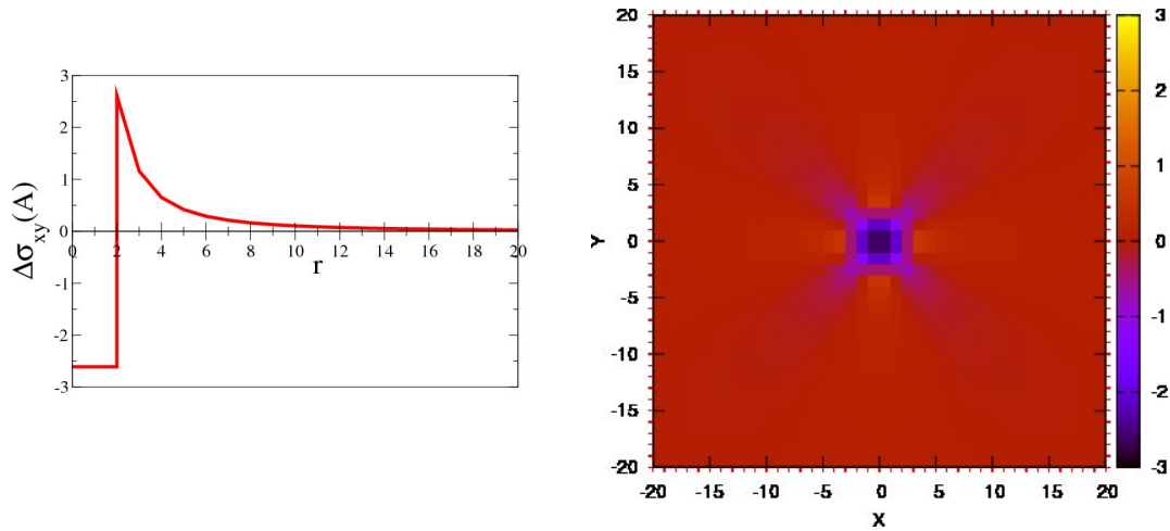
FIG. 5.8 : Typical quadrupole used in the numerical calculations, of amplitude A (here A \sim 0.25 ) diameter of the core d = 4 . Left : values of the stress drop along a line crossing the core of the quadrupole. Right : discretized values of the spatial stress redistribution.
