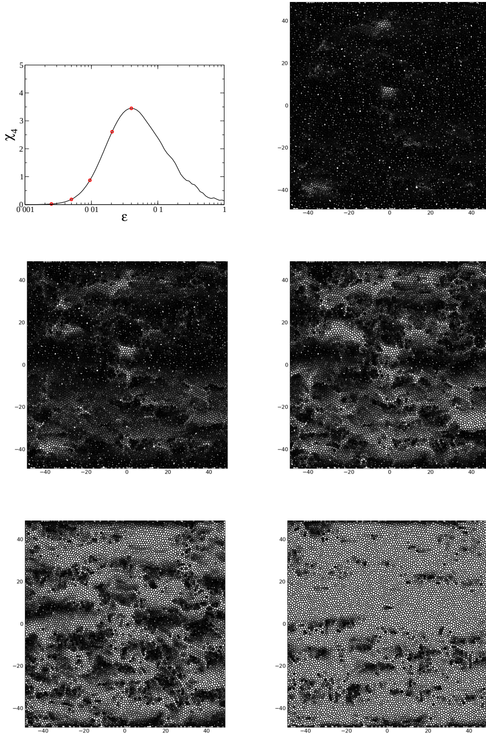
FIG. 6.14 : Top left corner : \chi_4(\varepsilon) . The red marks correspond to the strain intervals at which the five spatial maps of the self correlation function Q_s^i(\varepsilon) = \exp\left(\frac{\Delta r_i(\varepsilon)^2}{2a^2}\right) are computed. From top to bottom and from left to right, \varepsilon = 2.5 \cdot 10^{-3}, \varepsilon = 2.5 \cdot 10^{-3}, \varepsilon = 5 \cdot 10^{-3}, \varepsilon = 10^{-2}, \varepsilon = 2 \cdot 10^{-2} . All figures are obtained on a sample containing 10000 particles under RWBCs and at a shear rate of \dot{\gamma} = 5 \cdot 10^{-4} .
