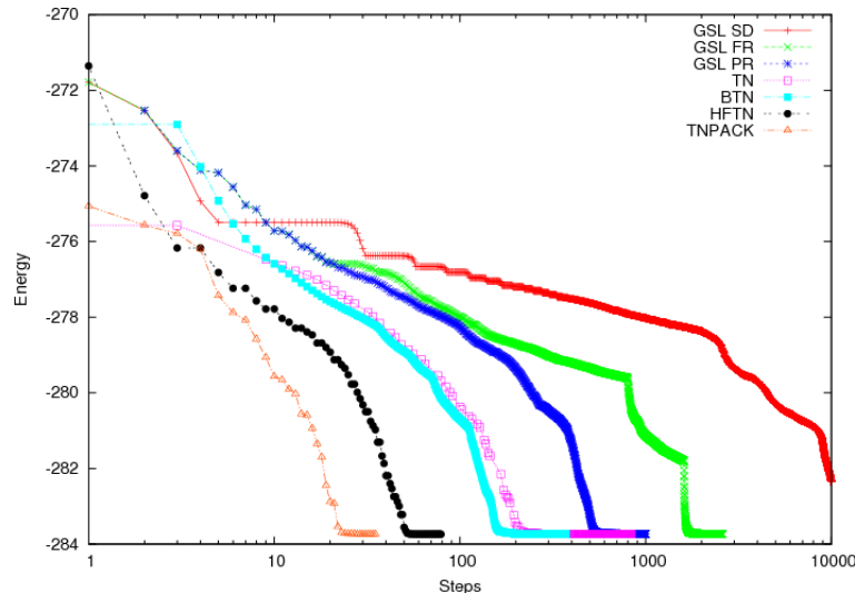
FIG. 2.2 : Evolution of the energy of a Lennard-Jones glass sample containing 100 particles during energy minimization for various algorithms. From slowest to fastest, steepest descent algorithm (GSL SD) [84], Fletcher-Reeves conjugate gradient algorithm (GSL FR) [84], Polak-Ribiere conjugate gradient algorithm (GSL PR) [84], block truncated newton (BTN) [85], truncated newton (TN) [86], hessian free truncated method (HFTN) [87], truncated newton package (TNPack) [88].
