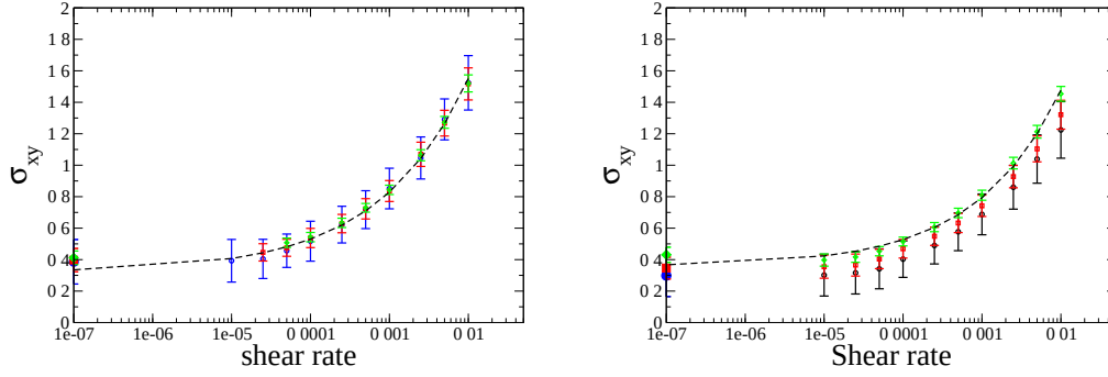
FIG. 6.2 : Flow curves associated with the different system sizes. Small open symbols correspond to finite shear rate values ranging from 10^{-5} to 10^{-2} . The larger solid points on the vertical axis correspond to the quasistatic protocol \dot{\gamma} = 0 . Left : Shear under LEBCs with fit parameter to the Herschel-Bulkley rheological law, \tau_Y \simeq 0.32 , c_1 = 7.2 and \beta = 0.38 . Right : Shear under RWBCs, with the dashed line representing a Herschel-Bulkley fit \tau = \tau_Y + c_1 \dot{\gamma}^\beta , with \tau_Y \simeq 0.36 , c_1 = 7.4 and \beta = 0.4 .
