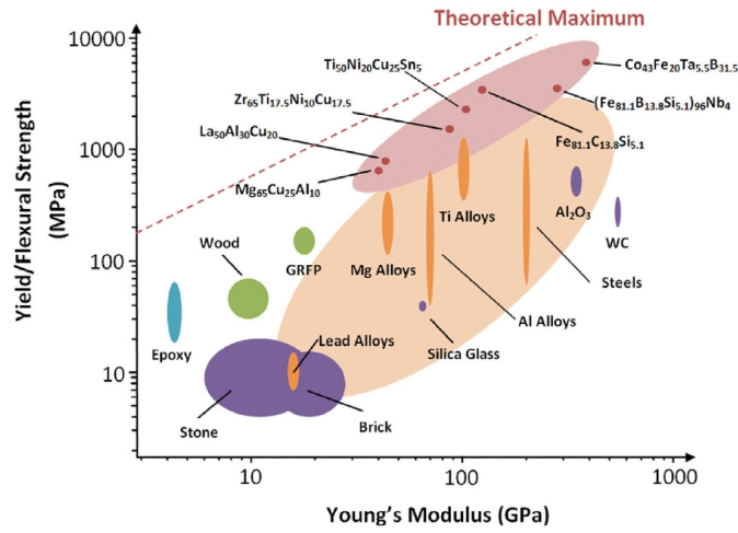
FIG. 1.3 : Schematic representation of room temperature yield (metals, composites and polymers) or flexural strength (ceramics) as a function of modulus. Note the increased strength of amorphous metals (light red) over conventional crystalline metals (light orange). [19] adapted from Greer[20].
