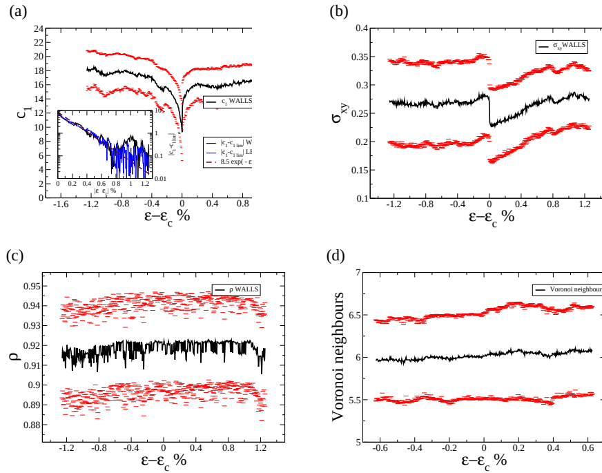
FIG. 4.18 : Evolution of different fields around a plastic event and averaged over all plastic events. (a) local shear modulus, (b) local shear stress, (c) local density and (d) number of Voronoi neighbours.
