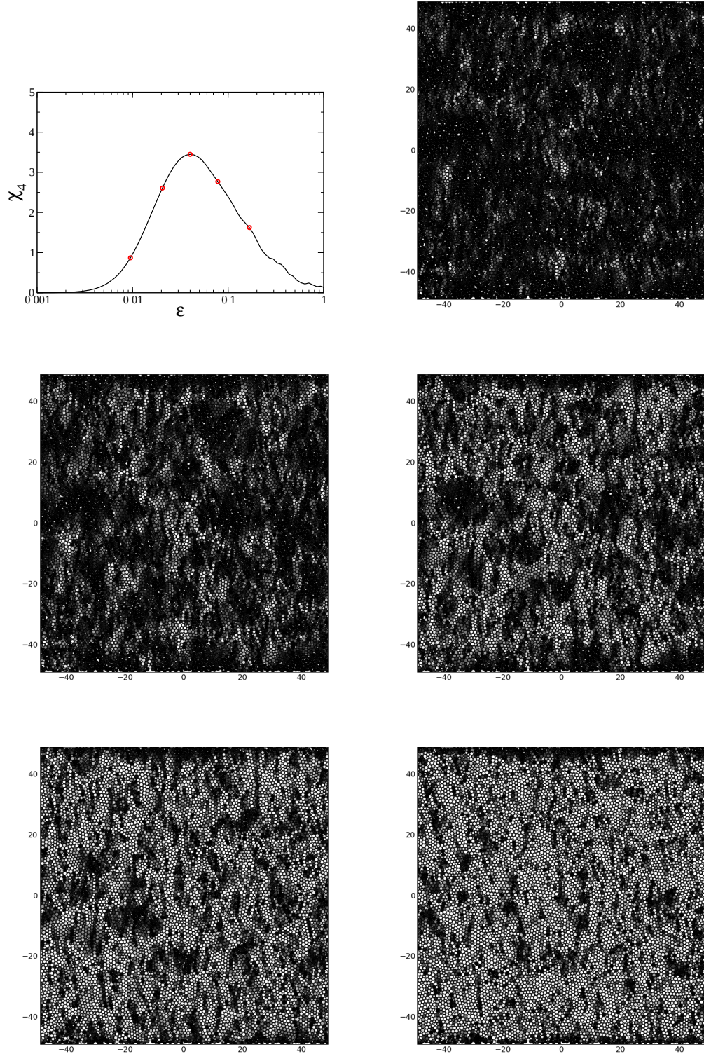
FIG. 6.13 : Top left corner : \chi_4(\varepsilon) . The red marks correspond to the strain intervals at which the five spatial maps of the self correlation function Q_s^i(\varepsilon) = \exp\left(\frac{\Delta y_i(\varepsilon)^2}{2a^2}\right) are computed. From top to bottom and from left to right, \varepsilon = 10^{-2}, \varepsilon = 2 \cdot 10^{-2}, \varepsilon = 4 \cdot 10^{-2}, \varepsilon = 8 \cdot 10^{-2}, \varepsilon = 16 \cdot 10^{-2} . All figures are obtained on a sample containing 10000 particles under RWBCs and at a shear rate of \dot{\gamma} = 5 \cdot 10^{-4} .
