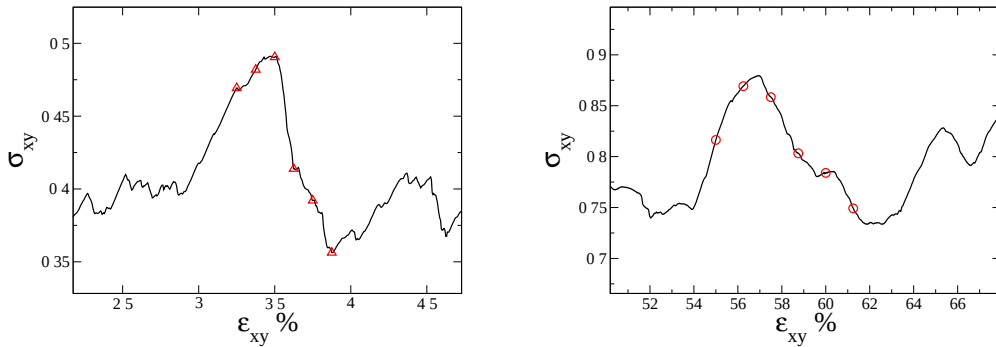
FIG. 6.3 : Portion of the mechanical stress-strain response of a Lennard-Jones glass containing 10000 particles and sheared under LEBs for two shear-rates. Left : \dot{\gamma} = 10^{-5} . Right : \dot{\gamma} = 10^{-3} .
