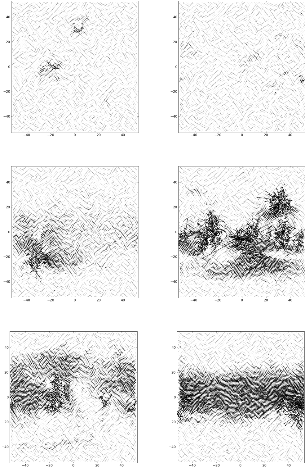
FIG. 6.4 : Snapshots of the instantaneous displacement field during 1 LJU and corresponding to the triangular symbols of figure 6.3. The shear-rate is here \dot{\gamma} = 10^{-5} .
