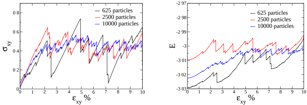
FIG. 5.1 : Left : Stress-strain response of three two-dimensional polydisperse Lennard-Jones glass under Lees-Edwards boundary conditions. Each curve corresponds to a different square cell of size 25, 50 and 100 particle diameters. Right : Energy-strain mechanical response of the same samples. Here the total energy is divided by the total number of particles to produce the average energy per particle.
