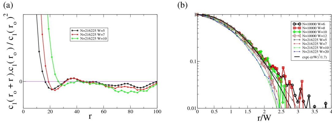
FIG. 3.10 : (a) Spatial correlation function of the local shear modulus c_1 : \langle (c_1(0) - \bar{c}_1)(c_1(r) - \bar{c}_1) \rangle . (b) Scaling of the function with the coarse-graining length W for small values of r .
