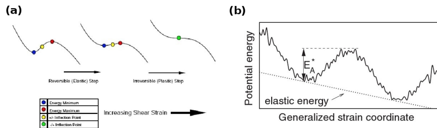
FIG. 4.8 : (a) A schematic representation of deformation induced changes of a local minimum in the potential energy landscape [205]. (b) Schematic illustration of the potential energy landscape of an individual STZ under applied shear stress. External shear strain or stress tilts the potential energy landscape and reduces the activation energy E_A^* of plastic shear events [206].
