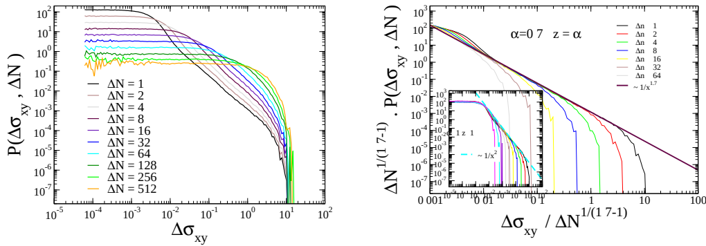
FIG. 5.17 : Left : Distribution P(\Delta\sigma_{xy}, \Delta n) of the variation of local shear stress \Delta\sigma_{xy} for different strain intervals \Delta n . The distribution has been obtained by averaging over the whole sample, and for different time origins. Right : Scaling of P(\Delta\sigma_{xy}, \Delta N) \propto \phi(\Delta\sigma_{xy}/\Delta N^{1/z}) with z = \alpha and \alpha = 0.7 . The scaling is very good in the intermediate range of the distribution, and for small \Delta N < 64 where the exponential cut-off does not play a role. Inset: the same with \alpha = 1 = z . This exponent corresponds also to the one discussed in the text.
