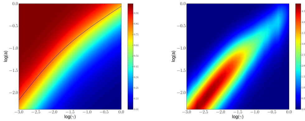
FIG. 6.10 : Dynamical correlation functions computed over the particles of a sample containing 2500 particles and sheared at \dot{\gamma} = 10^{-4} under RWBCs for a total strain \varepsilon_{tot} = 200\% . Left : Correlation function Q_s(a, \gamma) as a function of the probing length a and the strain \gamma in a log-log colormap. Right: Four-point correlation function \chi_4(a, \gamma) in a log-log colormap.
