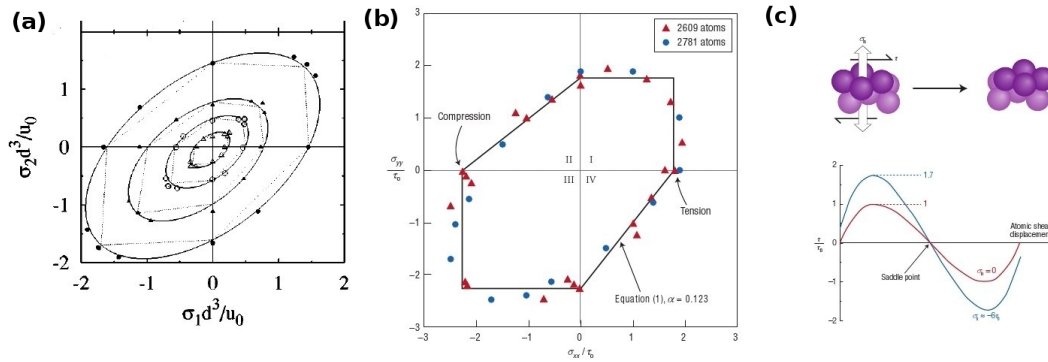
FIG. 4.5 : (a) Yield points for biaxial stress states obtained on a model polymer system [198]. The ellipses represent the pressure modified Von-Mises yield surface and the dashed lines show the pressure modified Tresca yield surface. (b) Yield surface of a model metallic glass. Normalized principle stresses \sigma_{xx} and \sigma_{yy} at yield ( \sigma_{zz} = 0 ) extracted from computational multiaxial mechanical tests. Data for two different amorphous structures are shown, composed of 2609 and 2781 atoms, respectively. The solid line is the Mohr-Coulomb yield criterion, plotted with the value of \alpha = 0.123 obtained from the elementary shear transformation zone analysis of figure (c). (c) On the top figure is represented a representation of the elementary three dimensional shear transformation zone used in [199]. The four upper (darker) atoms move as a unit with respect to the five lower atoms, and a trajectory with constant normal-stress \sigma_n is determined in the shear direction. In the bottom figure the applied shear stress \tau necessary to maintain a given atomic shear displacement, normalized by the maximum value of \tau at \sigma_n = 0, \tau_0 . The beginning and end of the curve correspond to the starting and ending structures seen in the top figure. The maximum value of \tau necessary to complete the shear displacement of the top figure increases with an applied compressive stress.
