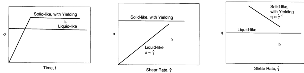
FIG. 1.1 : Left : Illustration of transient shear stress \sigma(t) for ‘liquid-like’ and ‘solid-like’ materials. Illustration of shear-rate dependent, middle : shear stress \sigma and right : shear viscosity \eta(\dot{\gamma}) \equiv \sigma/\dot{\gamma} for prototypical ‘liquid-like’ and ‘solid-like’ materials. [17]
