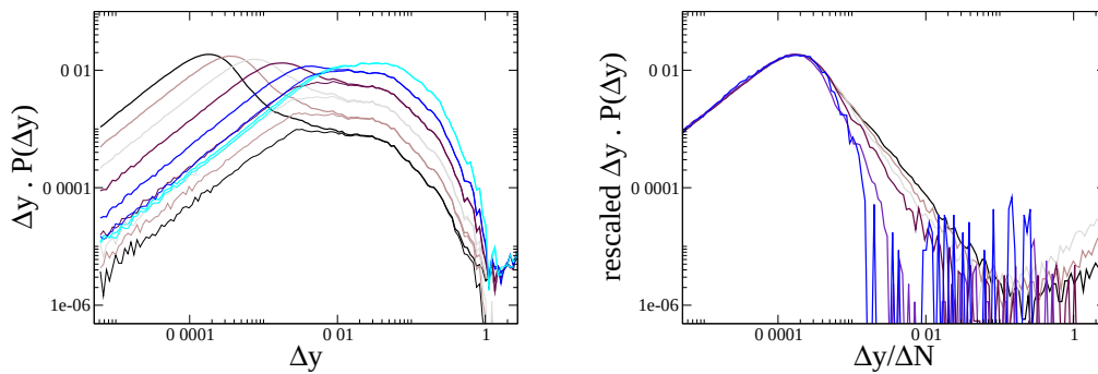
FIG. 5.16 : Left : Total distribution \Delta y \cdot P(\Delta y, \Delta N) (thick lines) and plastic contribution \Delta y \cdot P_{plastic}(\Delta y, \Delta N) (thin lines). Plastic intervals are considered when at least one macroscopic relaxation of the total stress has occurred during \Delta N . Right : Elastic contribution P_{elastic}(\Delta y, \Delta N) = P(\Delta y, \Delta N) - P_{plastic}(\Delta y, \Delta N) of the distribution of transverse displacements vs \Delta y/\Delta N , for \Delta N = 1, 2, 4, 8, 16, 32 and 64 . The function is normalized vertically at the maximum.
