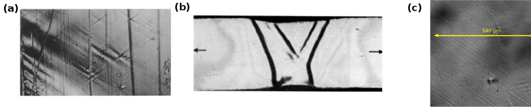
FIG. 1.6 : (a) Microscopic view of the polycarbonate specimen taken during stage II of the deformation shown on figure 1.5(b) [23]. Formation of shear bands at the beginning of necking, observed for a sample of polycarbonate. The arrows indicate the direction of the applied tensile stress. Micrograph obtained by Morbitzer [24, 25]; (c) microscopic shear bands located inside the macroscopic shear bands of (a) [26].
