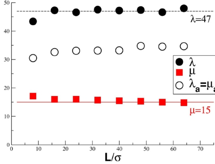
FIG. 3.1 : Lamé coefficients \lambda (spheres) and \mu (squares) vs system size L . Full symbols correspond to the direct measurement using Hooke's law; open symbols are obtained supposing affine deformations (Born term). The effect of system size is weak. The coefficients relying on a negligible nonaffine field differ by a factor as large as 2 from the true ones. Clearly, a calculation taking into account the nonaffine character of the displacement is necessary for disordered systems. Figure taken from [118].
