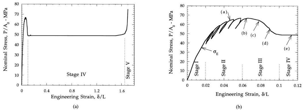
FIG. 1.5 : Nominal stress vs nominal extension of a polycarbonate specimen indicating the different stages in the deformation. (a) shows the full range and (b) shows an expanded view at small strain levels [23].
