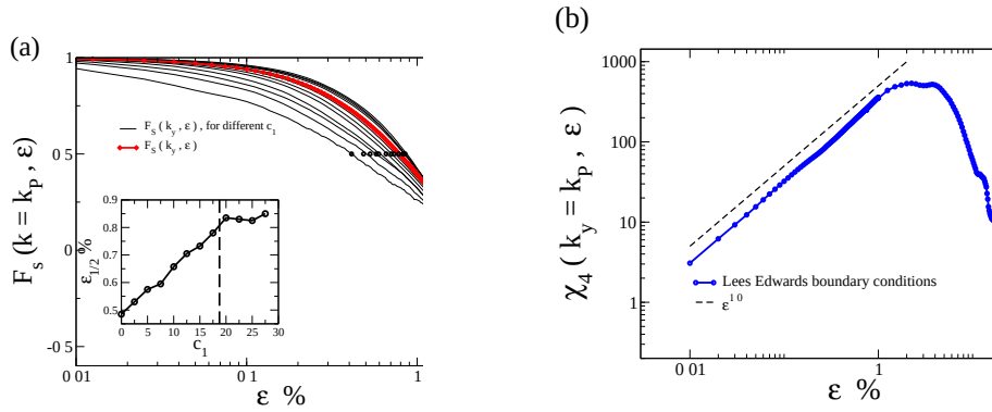
FIG. 4.16 : (a) Intermediate scattering function (SISF) F_s(\mathbf{k}, \varepsilon) plotted for \mathbf{k} = k_y = k_p (diamonds) and for regions of different softness c_1 (thin lines, from bottom to top the rigidity c_1 is increased). Inset in (a): the relaxation strain is shown as a function of the softness at the origin. (b) 4 point correlation function represented for Lees-Edwards boundary conditions (circles). For small strain increments the linear behavior is highlighted (dotted line).
