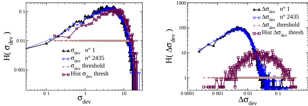
FIG. 4.6 : (a) Distribution of the deviatoric stress in a configuration of 10 000 particles for 2 different strains in the beginning and in the end of the plastic flow plateau (triangles). Comparison with the distribution of the deviatoric stress in the center of the future quadrupole just before the quadrupolar event takes place (squares), computed on the 2500 plastic events of the plastic flow regime. The 3 curves are very similar. (b) Same as in (a), but for the incremental deviatoric stress. In this case, the distribution obtained on the center of the quadrupoles indicates a more pronounced correspondence with the highest incremental stresses inside the sample.
