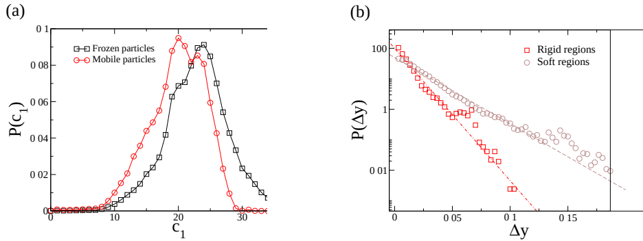
FIG. 4.15 : (a) Distribution of the local shear modulus for mobile and immobile particles. (b) Distribution of the nonaffine field during a total strain of 1% for rigid and soft regions.
