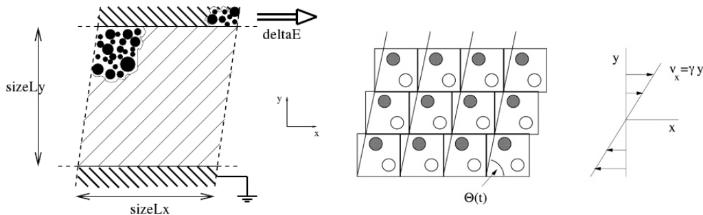
FIG. 2.4 : Left : Schematic representation [117] of the quasistatic shearing protocol in two dimensions and under RWBCs. The bottom and top walls contain here frozen LJ particles, while the x direction remains periodic. Right : Schematic representation of the LEBs.
