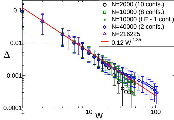
FIG. 3.3 : Deviation \Delta from linear elasticity as a function of the coarse-graining parameter W . For W \geq 5 Hooke's law is satisfied locally with more than 1% accuracy.
