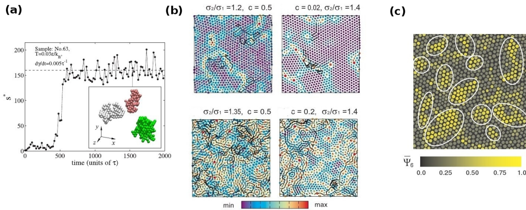
FIG. 4.4 : (a) Main: size of the largest cluster versus time in a sheared monodisperse Lennard-Jones glass. Broken line corresponds to the value 160. The study sample is still the same as for the previous figures. Inset: Three largest clusters at the moment indicated by arrow. The sizes of the clusters are N1 = 177 , N2 = 130 and N3 = 126 particles. [195] (b) Disorder variable D (opposite of hexatic order parameter) at T = 0.2\varepsilon/k_B and \phi = 0.9 for a bidisperse Lennard-Jones glass. The arrows represent the particle displacement over a time of the order of the relaxation time of the different glasses \tau_\alpha [196]. (c) Snapshot of a polydisperse colloidal system of \phi = 0.631 for polydispersity \Delta = 9\% [197].
