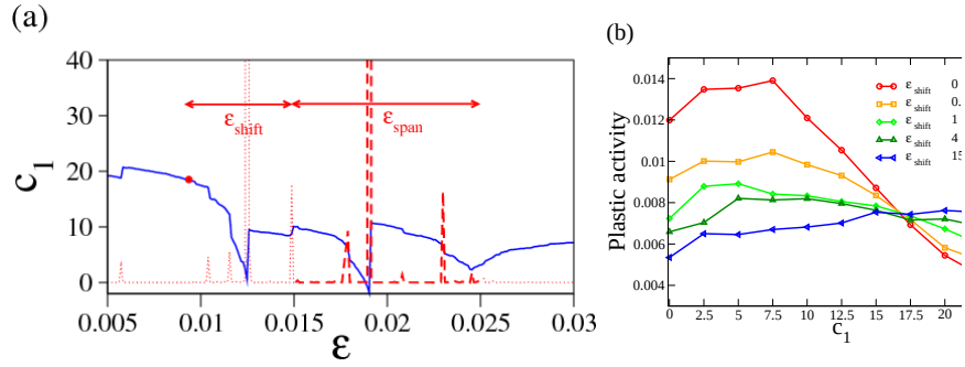
FIG. 4.17 : (a): Evolution of c_1 of a particle in a plastic zone. The dotted line represents the parameter D_{BF} that marks the local deviation from affinity. \varepsilon_{shift} and \varepsilon_{span} are defined for the point marked in red. (b): cumulative plastic activity for \varepsilon_{span} \sim 0.5\% and for different values of \varepsilon_{shift} .
