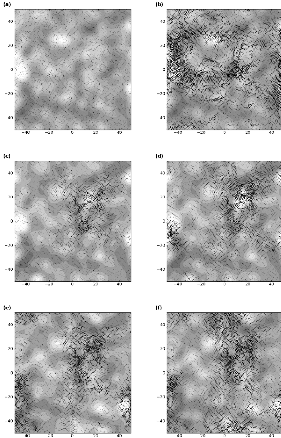
FIG. 4.14 : We represent the local map of the shear modulus at the same macroscopic strain values as in figure 13. These values correspond to the onset of plastic rearrangement of the material. These maps are superimposed with the non-affine displacement accumulated from figure (a). Figures (a) to (f) correspond to a macroscopic strain of (a)2.5%, (b)2.55%, (c)2.65%,(d)2.7%,(e)3.25% and (f)3.4%. Note that the non-affine field is multiplied by a factor 300 on figure (b) to illustrate the very strong correlation of the elastic non-affine field with the elasticity map for small incremental strain intervals (here 0.05%).
