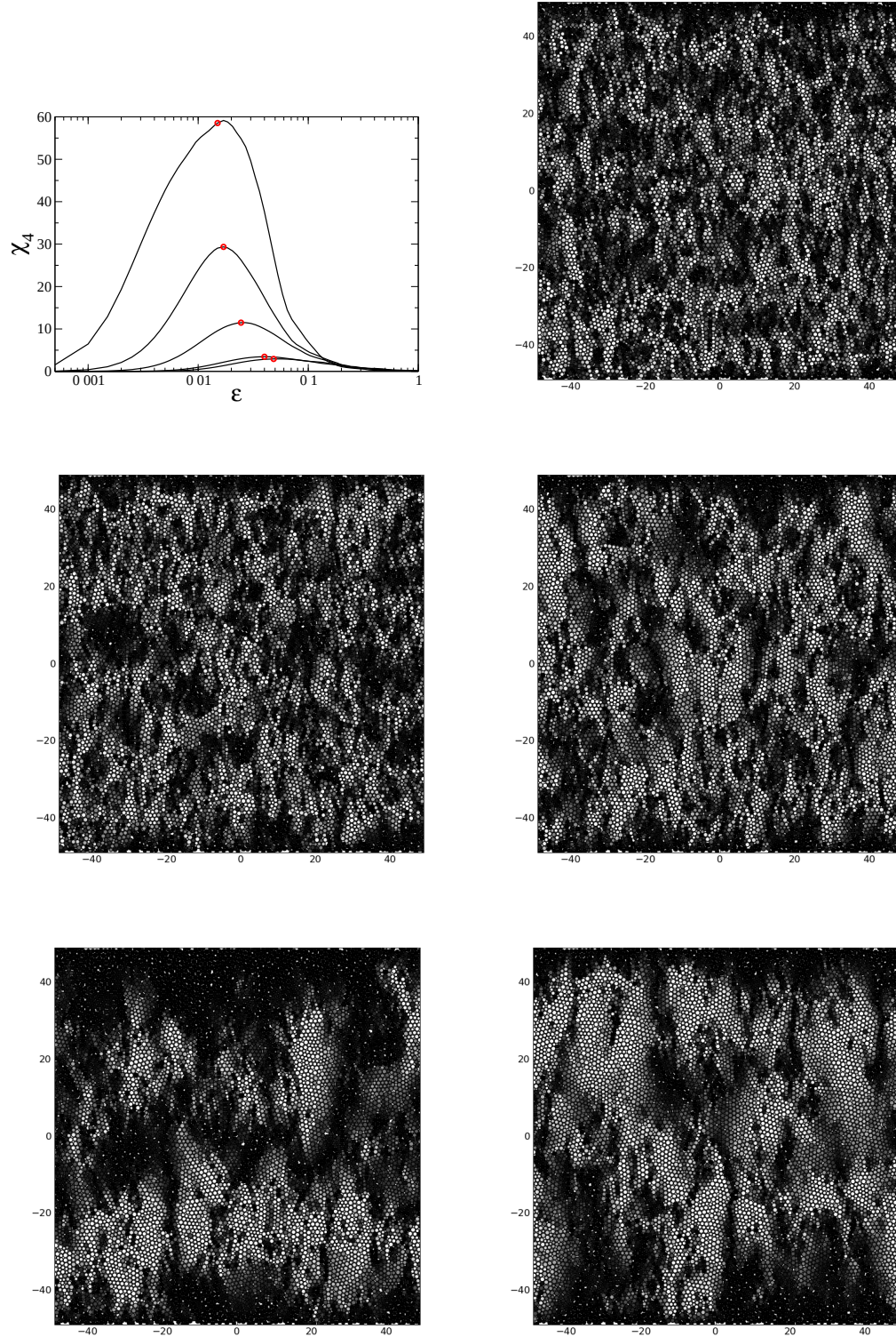
FIG. 6.15 : Top left corner : \chi_4(\varepsilon) . The red marks correspond to the strain intervals at which the five spatial maps of the self correlation function Q_s^i(\varepsilon) = \exp\left(\frac{\Delta y_i(\varepsilon)^2}{2a^2}\right) are computed. From top to bottom and from left to right, \dot{\gamma} = 10^{-3}, \dot{\gamma} = 5 \cdot 10^{-4}, \dot{\gamma} = 10^{-4}, \dot{\gamma} = 5 \cdot 10^{-5}, \dot{\gamma} = 10^{-5} . All figures are obtained on a sample containing 10000 particles and for RWBCs.
