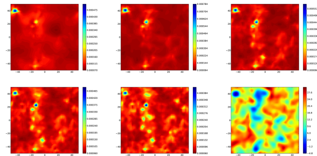
FIG. 4.22 : Map of the average participation fraction on the same configuration as in figure 4.21 for the 10, 30, 50, 75 and 100 lowest eigenmodes. Comparison with the local elasticity map of figure 4.21.
