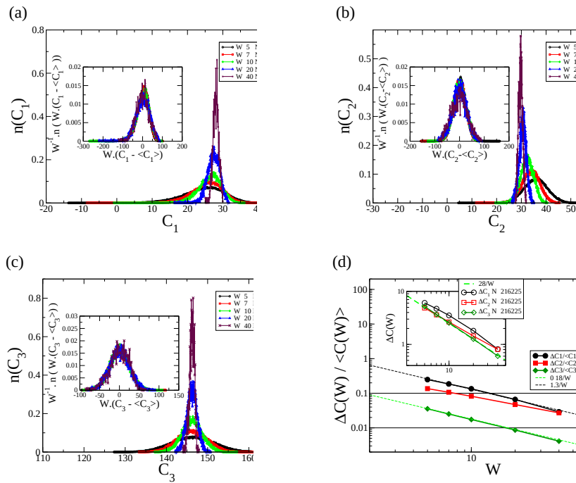
FIG. 3.7 : The figures (a), (b) and (c) show, respectively, the distributions of the three lowest eigenvalues c_1 , c_2 and c_3 for different coarse-graining lengths W . The inset of each figure show the distributions rescaled by W . Figure (d) shows that the distributions get narrower as W increases to converge to the macroscopic values of the elastic constants. The variances of the distributions is plotted as a function of W . The variances normalized by the average values of the distributions are also plotted. Both curves show a power law evolution with W .
