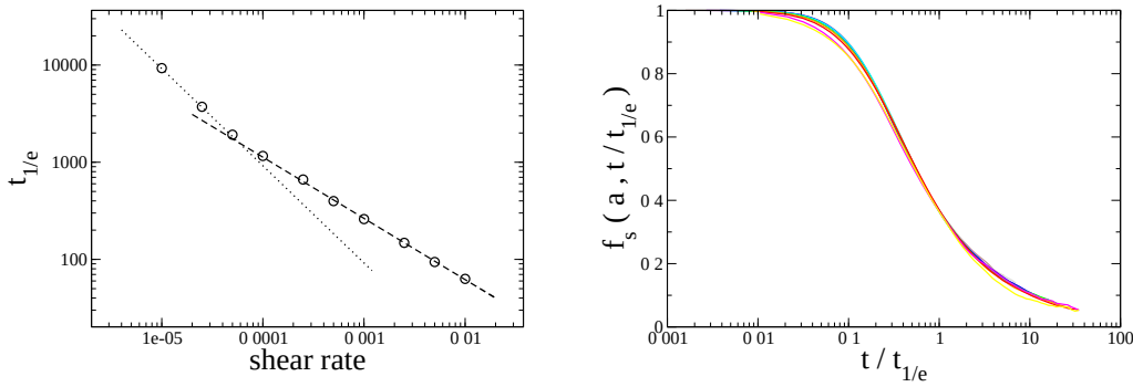
FIG. 6.7 : Left : Relaxation time t_{1/e} vs shear rate \dot{\gamma} for the system of figure 6.6. Dotted line t_{1/e} \propto \dot{\gamma}^{-1} , dashed line t_{1/e} \propto \dot{\gamma}^{-0.63} . Right: Rescaled self correlation function Q_s(a, t) of figure 6.6 when time is rescaled by the structural relaxation time t_{1/e} . All curves superimpose rather well on a master curve f_s(a, t/t_{1/e}) .
