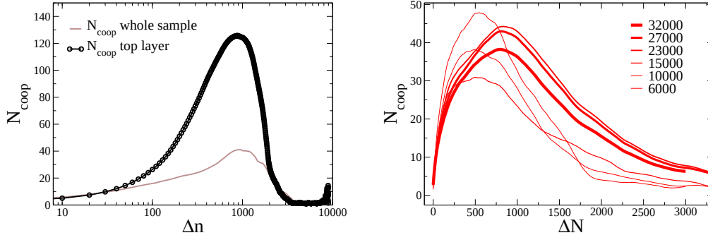
FIG. 5.13 : Left : Cooperativity number of the local shear stress at the borders, in comparison with cooperativity number in the center of the sample. Right : Cooperativity number obtained over different strain intervals. Increasing thickness of the curves reflects increasing averaging strain interval.
