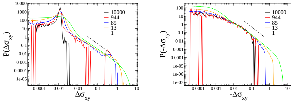
FIG. 5.5 : Log-log representation of the PDF of the stress drops where the stress are calculated over cells of different diameters ranging from the total sample of size 104 \times 104 (macroscopic stress) to the site stress (stress calculated on a single particle) and going through cells of diameter d = 104/3, 104/10 and 104/26 . The averages are calculated in the plastic flow for a total strain 5\% < \varepsilon < 10\% . Left : Positive stress jumps. Right : Negative stress jumps. The dashed line represent a guide to the eyes for a power law \propto \Delta\sigma_{xy}^{-1.7} .
