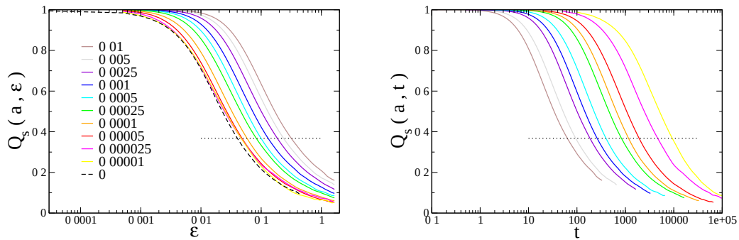
FIG. 6.6 : Left : 2-point correlation function Q_s(a, \varepsilon) = \sum_i \exp\left(-\frac{(y_i(\varepsilon) - y_i(0))^2}{2a^2}\right) against strain \varepsilon for a system with LEBC. Thin lines (color on pdf version) : from top to bottom shear rate values are 0.01, 0.005, 0.0025, 0.001, 0.0005, 0.00025, 0.0001, 0.00005 and 0.000025. Dashed line : Q_s(a, \varepsilon) vs \varepsilon for quasistatic shear. Dotted line corresponds to the value 1/e for which we calculate the 1/e -relaxation strains and times. Right: Q_s(a, t) against time t . In both figures the parameter a is chosen equal to 0.1.
