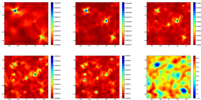
FIG. 4.20 : Map of the average participation fraction on the same configuration as in figure 4.19 for the 10, 30, 50, 75 and 100 lowest eigenmodes. Comparison with the local elasticity map of figure 4.19.
