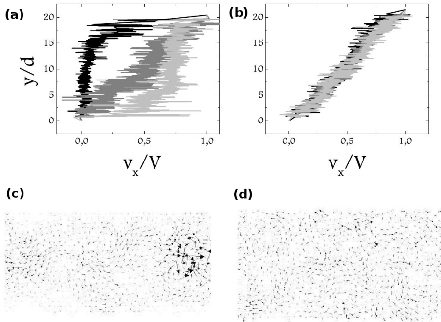
FIG. 1.11 : Instantaneous velocity profiles in simulation of dry granular material [49] for two different inertial numbers, in two dimensions defined as I = \dot{\gamma} \sqrt{\frac{m}{P}} , (a) I = 10^{-3} , (b) I = 10^{-1} . Non-affine velocity fluctuations in the quasistatic regime I = 10^{-3} (c) and in the dynamic regime I = 10^{-1} (d).
