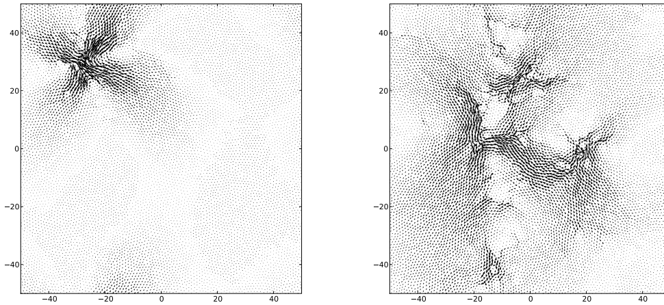
FIG. 5.2 : Left : Displacement field during a local rearrangement. Right : Displacement field ( \times 20 ) associated with a more complex spatial structural rearrangement involving many vortices.
