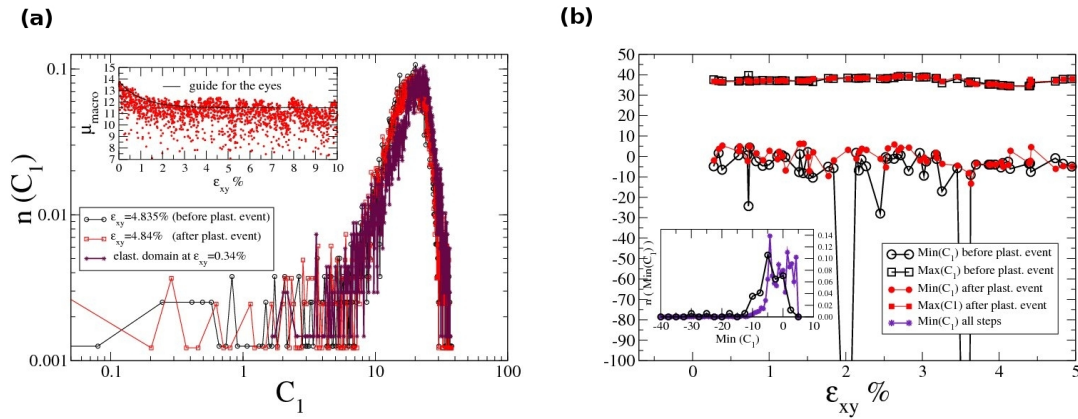
FIG. 3.8 : (a) Distributions of the local shear modulus c_1 averaged over the elastic regime and for two configurations in the plastic regime, just before and just after a rearrangement. Inset: Evolution with the macroscopic strain of the instantaneous macroscopic shear modulus defined as \Delta\sigma_{xy,macro} = \mu_{macro}\Delta\epsilon_{xy,macro} . (b) Evolution with the strain of the maximal and minimal values of c_1 . Inset: Distribution of the maximal and minimal values of the local elastic modulus c_1 over the entire plastic regime for all configurations, and for configurations just before the occurrence of a plastic event.
