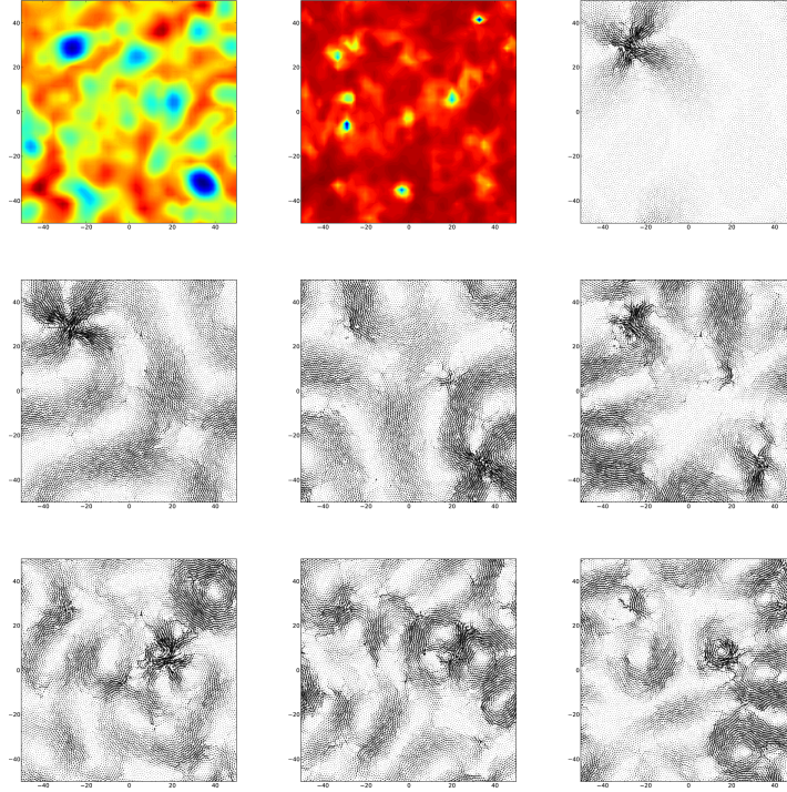
FIG. 4.19 : Analysis of the elasticity map and soft modes of a configuration at a macroscopic strain \varepsilon = 0.2725\% just prior to a localized quadrupolar rearrangement. From top to bottom and from left to right : Local elasticity map of the shear modulus C1 for a coarse-graining W = 5 , map of the average participation fraction |\mathbf{e}_\omega(\mathbf{x})|^2 over the 30 lowest eigenmodes, actual non-affine displacement during the plastic rearrangement between \varepsilon = 0.2725\% and \varepsilon = 0.275\% , first six eigenmodes with a participation ratio below 0.4 (see figure 4.23), i.e. the eigenmodes 10, 11, 26, 28, 29 and 34.
