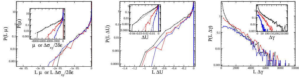
FIG. 5.4 : Raw PDFs in the insets and rescaled PDF in the main panels. Left : Stress drops. Middle : Energy drops. Right : Strain increments.
