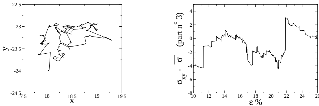
FIG. 5.14 : Left : Trajectory (non-affine part) of a single particle for a cumulative shear strain of 15%. The cell dimension is in this case L = 104 and the mean radius of the particles is a = 1 . Right : Evolution of the shear stress on a given particle in the center of the sample, as a function of the applied shear strain. For each value the average over the sample has been subtracted.
