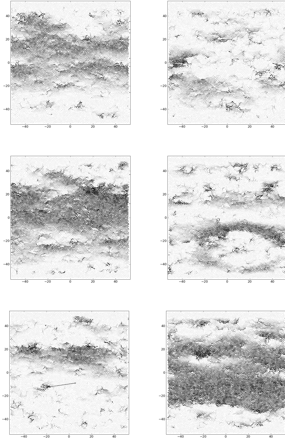
FIG. 6.5 : Snapshots of the instantaneous displacement field during 1 LJU and corresponding to the circular symbols of figure 6.3. The shear-rate is here \dot{\gamma} = 10^{-3} .
