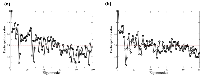
FIG. 4.23 : Participation ratio of the 100 lowest eigenmodes of (a) the configuration of figure 4.19 at \varepsilon = 0.2725\% , (b) the configuration of figure 4.21 at \varepsilon = 5.8625\% . The dashed lines at P(\omega) = 0.4 are arbitrarily chosen to determine a localization criterion.
