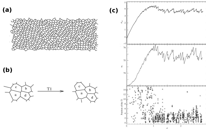
FIG. 1.9 : (a) Snapshot of a simulated foam with 16 \times 48 bubbles. The polydispersity is 6%. The foam has periodic boundary conditions along the x direction. Films laying at upper and lower edges are fixed; shearing is obtained by moving the lower edge along the x direction. (b) Example of a topological change (T1 process) occurring inside the foam upon shearing. (c) Evolutions from top to bottom of the shear stress, the free energy and the positions of the T1 events within the gap as a function of the applied strain [11].
