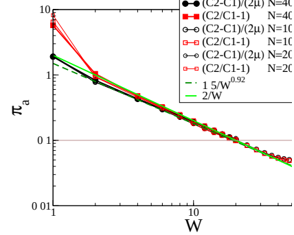
FIG. 3.4 : (a) The three eigenvalues of the elasticity tensor averaged spatially as a function of the coarse-grain length W . (b) log-log plot of the convergence of the three eigenvalues to the limit values obtained by a coarse graining on the whole system size. (c) Anisotropy parameter \pi_a as a function of the coarse-graining scale W .
