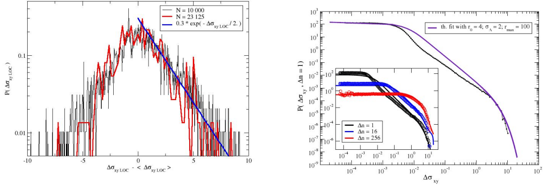
FIG. 5.10 : Left : Distribution of shear stress releases in the center of the quadrupoles, during a plastic event. The fit is exponential with a characteristic \Delta\sigma = 2 . Right : Comparison of the distribution P(\Delta\sigma_{xy}, \Delta n = 1) with the theoretical fit discussed in the text. The parameters of the fit are indicated in the legend box. Inset: evolution of the distribution with \Delta n . The symbols are the numerical results. The lines are obtained by a simple convolution of the theoretical curve obtained for \Delta n = 1 . It assumes no temporal correlation between successive events.
