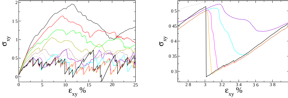
FIG. 6.1 : Left : stress strain mechanical response of a glass sample containing 625 particles sheared under RWBCs at shear rates ranging from \dot{\gamma} = 10^{-2} to \dot{\gamma} = 10^{-5} (thin colored lines from top to bottom, \dot{\gamma} = 10^{-2} (black), \dot{\gamma} = 5 \cdot 10^{-3} (red), \dot{\gamma} = 2.5 \cdot 10^{-3} (green), \dot{\gamma} = 10^{-3} (dark green), \dot{\gamma} = 5 \cdot 10^{-4} (brown), \dot{\gamma} = 2.5 \cdot 10^{-4} (gray), \dot{\gamma} = 10^{-4} (violet), \dot{\gamma} = 5 \cdot 10^{-5} (cyan), \dot{\gamma} = 2.5 \cdot 10^{-5} (magenta) and \dot{\gamma} = 10^{-5} (orange)). The thick black line corresponds to the quasistatic shear protocol. Right : Zoom in a portion of the total mechanical response, illustrating the typical relaxation time associated to a plastic rearrangement in the glass signaled in the quasistatic protocol by an abrupt stress drop.
