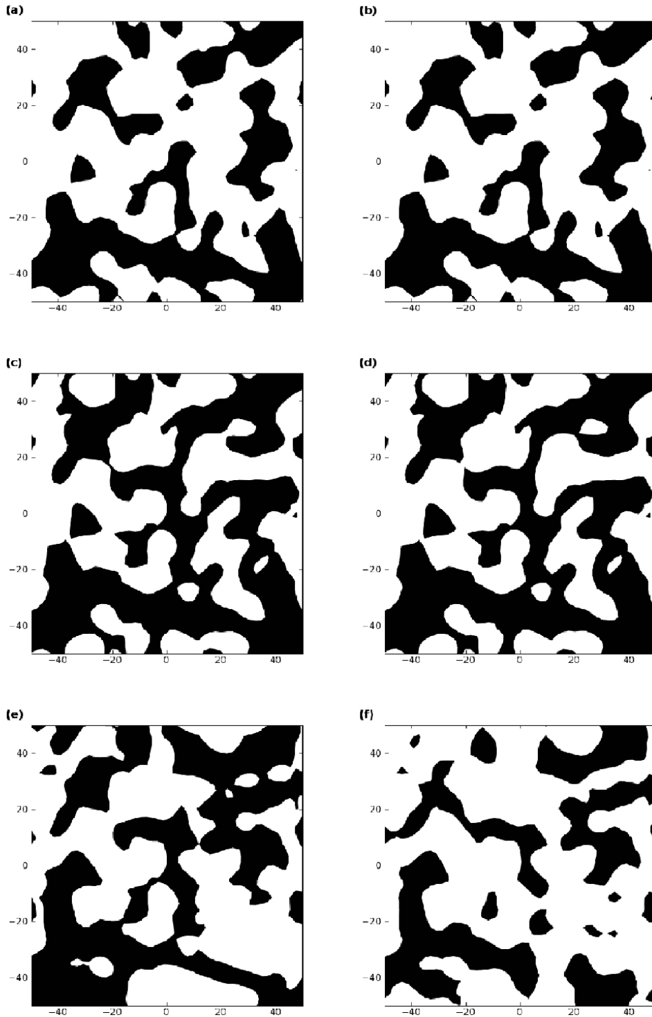
FIG. 4.13 : Shear modulus divided in rigid ( c_1 \geq \bar{c}_1 , black) and soft zones ( c_1 \leq \bar{c}_1 , white) for different macroscopic strains. Figures (a) to (f) correspond to a macroscopic strain of (a)2.5%, (b)2.55%, (c)2.65%,(d)2.7%,(e)3.25% and (f)3.4%.
