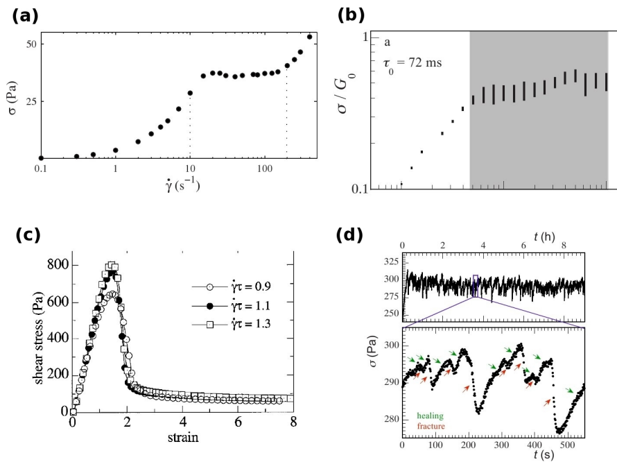
FIG. 1.8 : (a) Engineering flow curve (in the concentrated wormlike micellar system CTAB at 20% wt. in D_2O ) \sigma(\dot{\gamma}) at T = 41^\circ C under controlled shear rate obtained by averaging the shear stress over the last 100 s of each step [41]. (b) Dimensionless shear stress \sigma/G_0 versus dimensionless \dot{\gamma}\tau_0 ( G_0 = 500\text{Pa} , \tau_0 = 72\text{ms} ) for a transient polymer network at 25 g/L at T = 5^\circ C . The vertical bars indicate the range of stress fluctuations for a given shear rate. The grey region indicates where shear banding and fluctuating stresses are found [42, 43]. (c) Transient stress measurements obtained from start-up experiments at various shear rates. (telechelich polymer network analysed in [39]) (d) Typical transient stress response in the banded regime, at a steady shear rate of \dot{\gamma} = 1 , measured at T = 10^\circ C ( \tau_0 = 36\text{ms} ). Note that at short time scales ( \simeq \tau_0 ), at the start-up of the shear flow, the stress shows an overshoot, which is not visible here due to the longer sampling interval of 1\text{s} \approx 30\tau_0 [42, 43].
