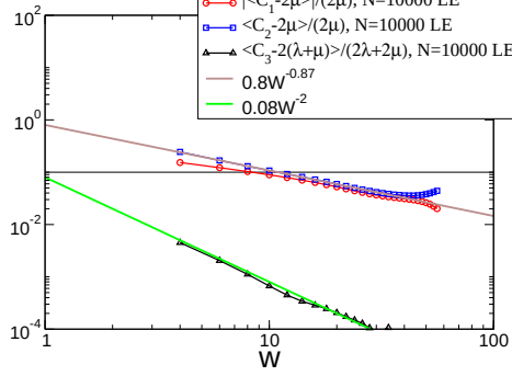
FIG. 3.4 : (a) The three eigenvalues of the elasticity tensor averaged spatially as a function of the coarse-grain length W . (b) log-log plot of the convergence of the three eigenvalues to the limit values obtained by a coarse graining on the whole system size. (c) Anisotropy parameter \pi_a as a function of the coarse-graining scale W .
