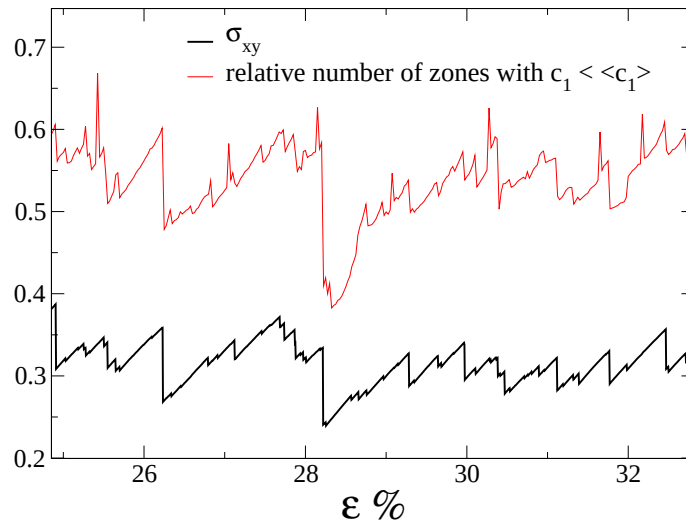
FIG. 4.11 : Evolution of the total shear stress (thick line) and the relative number of soft zones (relative number of points \mathbf{r} where c_1(\mathbf{r}) < \bar{c}_1 ) as a function of the applied shear strain, in the plastic flow regime.
