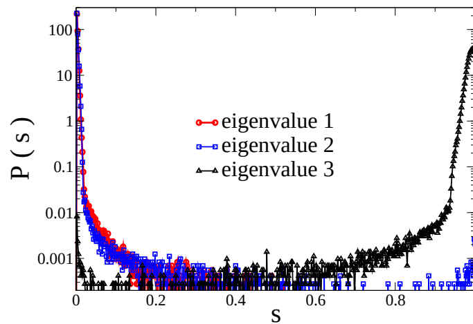
FIG. 3.6 : Distribution for each eigenvalue E_i of the local elasticity tensor of the quantity S_i = (tr(E_i))^2 / 2tr(E_i^2) . The distribution is obtained over the entire plastic flow regime.
