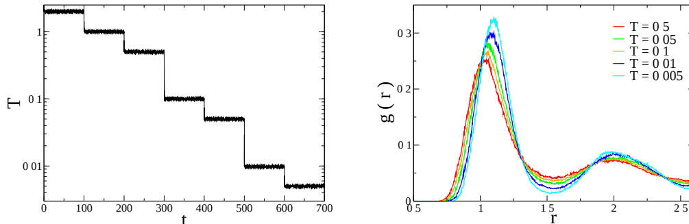
FIG. 2.3 : Left : Temperature evolution during the quench protocol used to produce the Lennard-Jones glass samples. Time and temperature are expressed in LJ units. Right : Evolution during quench of the radial distribution function.
