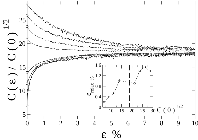
FIG. 4.10 : Autocorrelation function C(\Delta\varepsilon) = \overline{\langle c_1(\mathbf{r}, \varepsilon + \Delta\varepsilon)c_1(\mathbf{r}, \varepsilon) \rangle} of the order parameter conditioned by the value of c_1(\mathbf{r}, \varepsilon) at the origin. The curves correspond from bottom to top to increasing values of c_1(\mathbf{r}, \varepsilon) at the origin taken in the ranges [5-7,5],[7.5,10],[10,12.5],[12.5,15],[20-22.5],[22.5,25],[25,27.5], and [27.5,30] as marked by the circles. The dashed line corresponds to \overline{c_1} . Inset: the typical relaxation strain \varepsilon_{relax} associated with each rigidity c_1 \sim C(0)^{1/2} defined as the strain for which the rescaled autocorrelation function has decayed by half.
