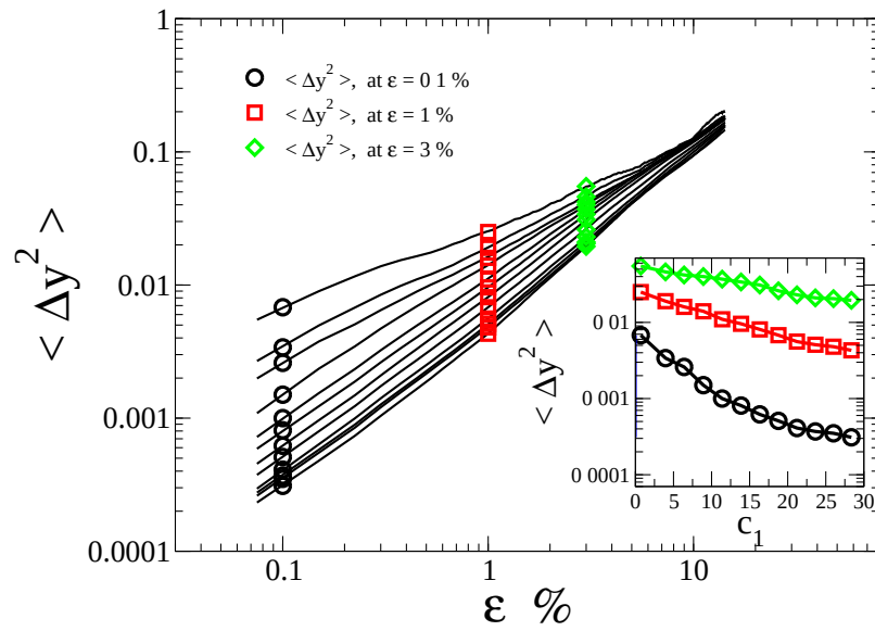
FIG. 4.12 : Mean-square displacement \langle \Delta y^2 \rangle for different values of the original local shear modulus c_1 . From top to bottom the curves correspond to c_1 taken in the ranges [0-2.5] , [2.5,5] , [5-7.5] , [7.5,10] , [10,12.5] , [12.5,15] , [20-22.5] , [22.5,25] , [25,27.5] , and [27.5,30] . Inset: \langle \Delta y^2 \rangle is shown as a function of c_1 for different relaxation strains.
