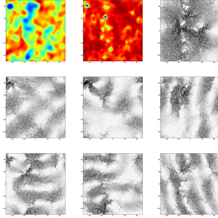
FIG. 4.21 : Analysis of the elasticity map and soft modes of a configuration at a macroscopic strain \varepsilon = 5.8625\% just prior to a large shear band. From top to bottom and from left to right : Local elasticity map of the shear modulus C1 for a coarse-graining W = 5 , map of the average participation fraction |\mathbf{e}_\omega(\mathbf{x})|^2 over the 30 lowest eigenmodes, actual non-affine displacement during the plastic rearrangement between \varepsilon = 5.8625\% and \varepsilon = 5.875\% , first six eigenmodes with a participation ratio below 0.4 (see figure 4.23), i.e. the eigenmodes 9, 10, 11, 12, 15 and 16.
