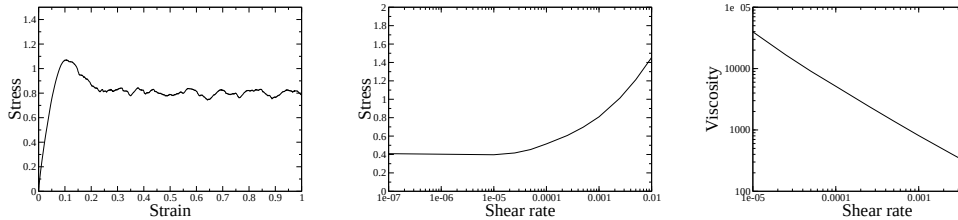
FIG. 1.2 : Parallel to figure 1.1 for the model Lennard-Jones glass system studied in this thesis. Left : Transient shear stress \sigma(\gamma) at a shear rate of \dot{\gamma} = 10^{-3} for a sample containing 10000 particles. Illustration of shear-rate dependent, middle : shear stress \sigma and right : shear viscosity \eta(\dot{\gamma}) \equiv \sigma/\dot{\gamma} for the same Lennard-Jones glass at various shear rates ranging from 0 to 10^{-2} . For more details see chapters 5 and 6.
