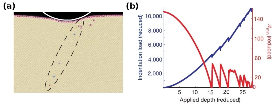
FIG. 4.7 : (a) MD simulation after several dipole nucleation events illustrating the formation of a shear band (dashed lines) after the dissociation of dislocation pairs to the free surface and crystalline interior. (b) Applied displacement load response (blue) of MD simulated bubble raft, showing correlation of load drops with a sequence of observed homogeneous dislocation dipole nucleation events. The elastic instability criterion \Lambda_{min} (red) tends to zero for the first several nucleation events. All nucleation events occur subsurface [161, 204].
