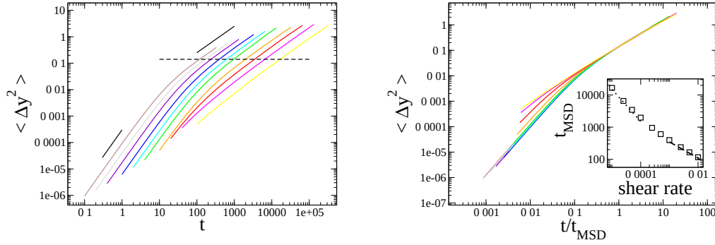
FIG. 6.8 : Left : Transverse mean square displacement (MSD) \langle \Delta y^2 \rangle versus time for different shear rates \dot{\gamma} (same color code as in previous figures). The dashed line marks the arbitrarily chosen distance criterion verifying a^2 = 0.14 corresponding to a ‘Lindemann’ criterion for the transverse MSD of the particles. The intersection of this line with the colored curves marks the times t_{\text{MSD}} . The two thick black lines correspond to the power laws t^2 and t^1 , i.e. respectively to the ballistic and diffusive regime. Right: same figure where time is rescaled by the times t_{\text{MSD}} . These plots are obtained in configurations with RWBCs and the average are computed in a central region of the samples therefore avoiding direct influence of the walls.
