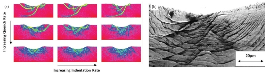
FIG. 1.4 : Sub-surface shear band morphologies resultant to indentation. (a) As simulated by the calculated local deviatoric strain field for a binary metallic glass (red is 0% strain and yellow 40%) [21] (b) As cast Zr_{52.5}Al_{10}Ti_5Cu_{17.9}Ni_{14.6} using the clamped interface technique [22]
