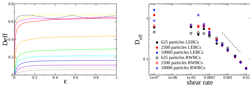
FIG. 6.9 : Left : Effective diffusion coefficients defined as De_{\text{eff}}(\Delta\gamma) = \langle \Delta y^2 \rangle / 2\Delta\gamma for different shear rates ranging from bottom to top from \dot{\gamma} = 10^{-5} to 10^{-5} (same color code as previous figures) and for the quasistatic shear protocol (black dashed line). De_{\text{eff}} is computed here for samples containing 2500 particles under RWBCs. The spatial averaging is performed sufficiently far from the rigid walls to avoid boundary effects. Right: The asymptotic values De_{\text{eff}} are plotted for various shear rates, system sizes and boundary conditions. The dashed line marks the power law De_{\text{eff}} \propto \dot{\gamma}^{-0.5} as a guide to the eyes.
