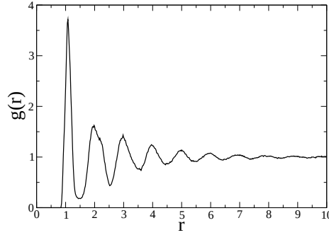
FIG. 5.11 : Radial distribution function calculated on a 104 \times 104 sample with Lees Edwards boundary conditions.
