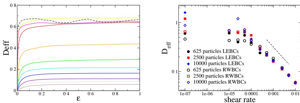
FIG. 6.9 : Left : Effective diffusion coefficients defined as D_{\text{eff}}(\Delta\gamma) = \langle \Delta y^2 \rangle / 2\Delta\gamma for different shear rates ranging from bottom to top from \dot{\gamma} = 10^{-5} to 10^{-5} (same color code as previous figures) and for the quasistatic shear protocol (black dashed line). D_{\text{eff}} is computed here for samples containing 2500 particles under RWBCs. The spatial averaging is performed sufficiently far from the rigid walls to avoid boundary effects. Right: The asymptotic values D_{\text{eff}} are plotted for various shear rates, system sizes and boundary conditions. The dashed line marks the power law D_{\text{eff}} \propto \dot{\gamma}^{-0.5} as a guide to the eyes.
