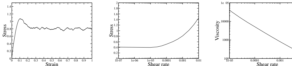
FIG. 1.2 : Parallel to figure 1.1 for the model Lennard-Jones glass system studied in this thesis. Left : Transient shear stress \sigma(\gamma) at a shear rate of \dot{\gamma} = 10^{-3} for a sample containing 10000 particles. Illustration of shear-rate dependent, middle : shear stress \sigma and right : shear viscosity \eta(\dot{\gamma}) \equiv \sigma/\dot{\gamma} for the same Lennard-Jones glass at various shear rates ranging from 0 to 10^{-2} . For more details see chapters 5 and 6.
