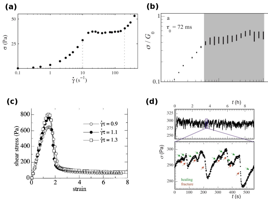
FIG. 1.8 : (a) Engineering flow curve (in the concentrated wormlike micellar system CTAB at 20% wt. in D 2 O) \sigma(\dot{\gamma}) at T = 41°C under controlled shear rate \dot{\gamma} obtained by averaging the shear stress over the last 100 s of each step [41]. (b) Dimensionless shear stress \sigma/G_0 versus dimensionless shear rate \dot{\gamma}\tau_0 ( G_0 = 500 Pa, \tau_0 = 72 ms) for a transient polymer network at 25 g/L at T = 5°C. The vertical bars indicate the range of stress fluctuations for a given shear rate. The grey region indicates where shear banding and fluctuating stresses are found [42, 43]. (c) Transient stress measurements obtained from start-up experiments at various shear rates. (telechelich polymer network analysed in [39]) (d) Typical transient stress response in the banded regime, at a steady shear rate of \dot{\gamma} = 1 , measured at T = 10°C ( \tau_0 = 36 ms). Note that at short time scales ( \approx \tau_0 ), at the start-up of the shear flow, the stress shows an overshoot, which is not visible here due to the longer sampling interval of 1\text{ s} \approx 30\tau_0 [42, 43].
