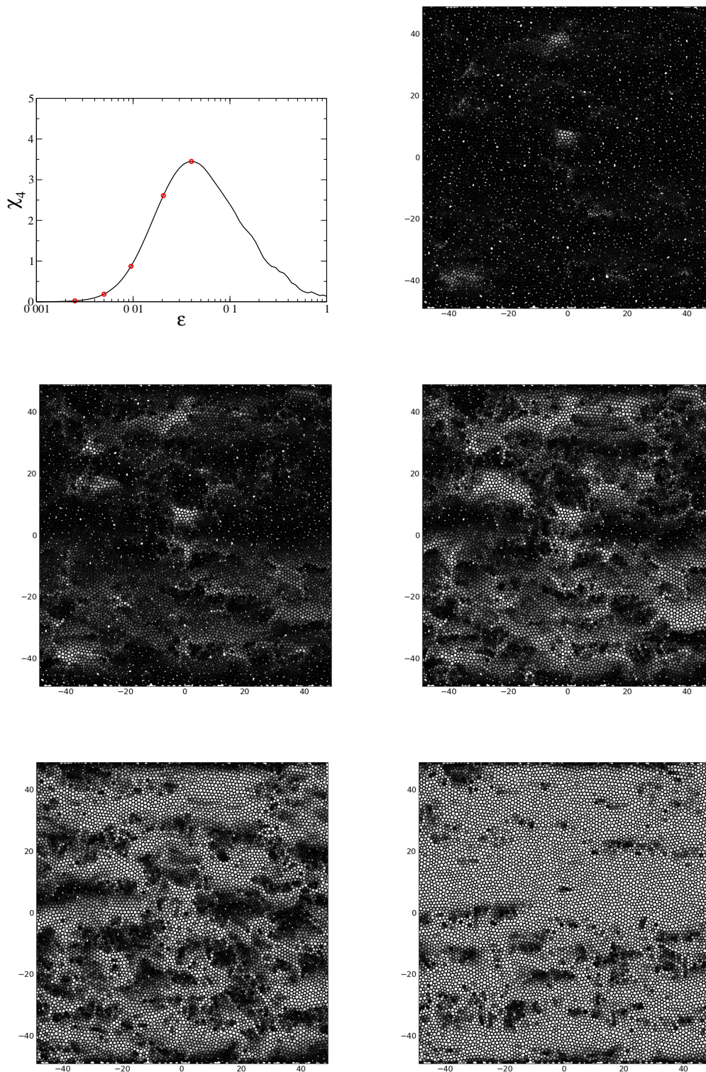
FIG. 6.14 : Top left corner : \chi_4(\epsilon) . The red marks correspond to the strain intervals at which the five spatial maps of the self correlation function Q_s^i(\epsilon) = \exp\left(\frac{\Delta r_i(\epsilon)^2}{2a^2}\right) are computed. From top to bottom and from left to right, \epsilon = 2.5 \cdot 10^{-3}, \epsilon = 2.5 \cdot 10^{-3}, \epsilon = 5 \cdot 10^{-3}, \epsilon = 10^{-2}, \epsilon = 2 \cdot 10^{-2} . All figures are obtained on a sample containing 10000 particles under RWBCs and at a shear rate of \dot{\gamma} = 5 \cdot 10^{-4} .
