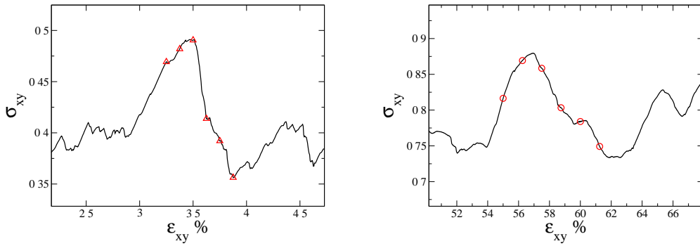
FIG. 6.3 : Portion of the mechanical stress-strain response of a Lennard-Jones glass containing 10000 particles and sheared under LEBCs for two shear-rates. Left : \dot{\gamma} = 10^{-5} . Right : \dot{\gamma} = 10^{-3} .
