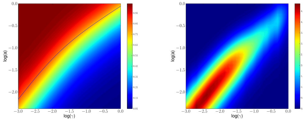
FIG. 6.10 : Dynamical correlation functions computed over the particles of a sample containing 2500 particles and sheared at \dot{\gamma} = 10^{-4} under RWBCs for a total strain \varepsilon_{tot} = 200\% . Left : Correlation function Q_s(a, \gamma) as a function of the probing length a and the strain \gamma in a log-log colormap. Right : Four-point correlation function \chi_4(a, \gamma) in a log-log colormap.
