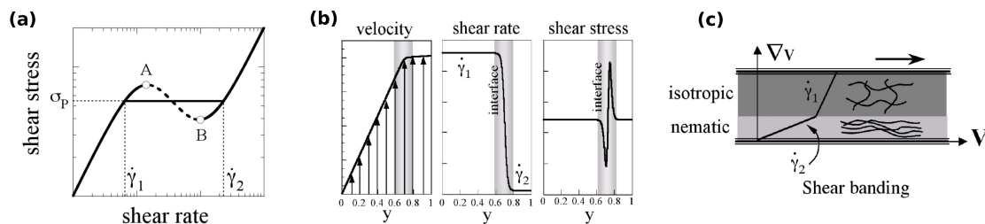
FIG. 1.7 : (a) Non monotonic constitutive equation assumed for wormlike micelles. The two stable branches at low and high shear rates are separated by an unstable portion [AB]. In the plateau region, the micellar solution demixes in bands of shear rate \dot{\gamma}_1 and \dot{\gamma}_2 (b) Velocity, shear rate and shear stress profiles calculated under the assumptions of shear banding and of non monotonic flow curve. (c) Schematic representation of the shear banding for system undergoing a shear induced isotropic-to-nematic transition.
