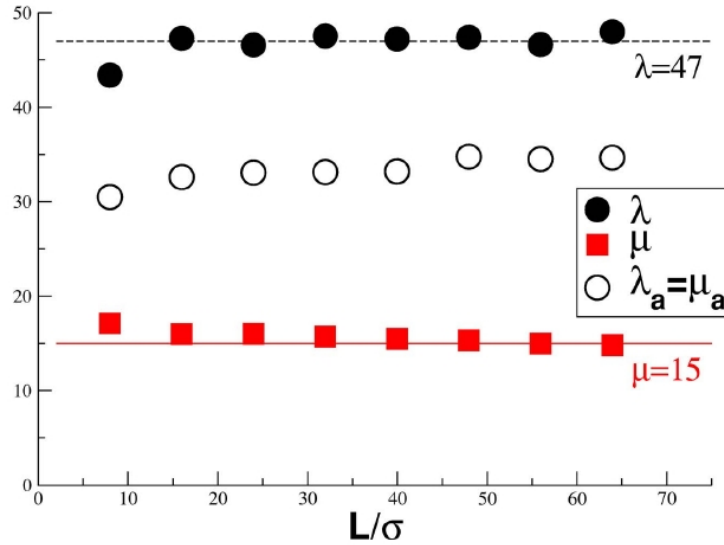
FIG. 3.1 : Lamé coefficients \lambda (spheres) and \mu (squares) vs system size L . Full symbols correspond to the direct measurement using Hooke's law; open symbols are obtained supposing affine deformations (Born term). The effect of system size is weak. The coefficients relying on a negligible nonaffine field differ by a factor as large as 2 from the true ones. Clearly, a calculation taking into account the nonaffine character of the displacement is necessary for disordered systems. Figure taken from [118].
