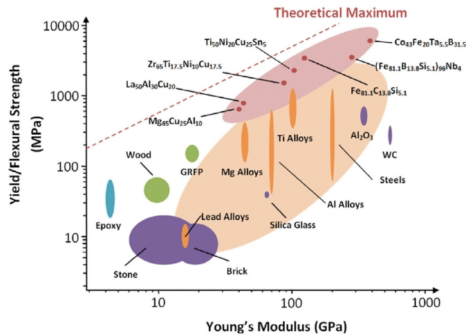
FIG. 1.3 : Schematic representation of room temperature yield (metals, composites and polymers) or flexural strength (ceramics) as a function of modulus. Note the increased strength of amorphous metals (light red) over conventional crystalline metals (light orange). [19] adapted from Greer[20].
