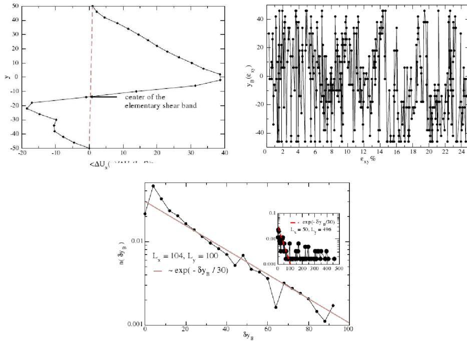
FIG. 5.7: Top left: Averaged horizontal displacement associated to a single but large event. The y-position, where the non-affine displacement field is equal to zero, allows to determine the center of the elementary shear band. Distances are expressed in units of the average particle diameter a . Top right: Position y_B of the centers of elementary shear bands (determined as described previously), here for the 5000 first steps. No localization appears, even for very large deformation (170%, not shown here). Bottom: Distribution of the distances \delta y_B between successive elementary shear bands for L_x = 104, L_y = 100 . The characteristic distance of the exponential fit is \xi \sim 30a . Inset: same distribution for the largest system size L_y = 496 . The characteristic distance is the same, \xi .
