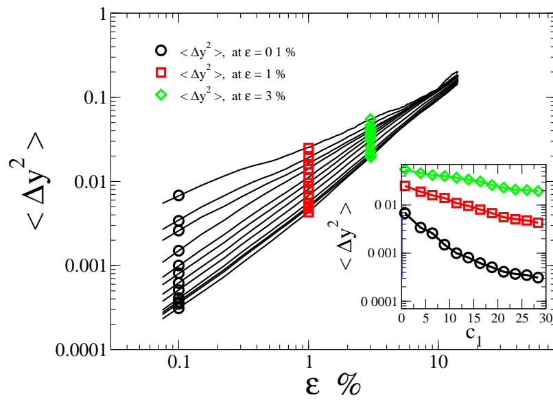
FIG. 4.12 : Mean-square displacement \langle \Delta y^2 \rangle for different values of the original local shear modulus c_1 . From top to bottom the curves correspond to c_1 taken in the ranges [0-2.5] , [2.5,5] , [5-7.5] , [7.5,10] , [10,12.5] , [12.5,15] , [20-22.5] , [22.5,25] , [25,27.5] , and [27.5,30] . Inset: \langle \Delta y^2 \rangle is shown as a function of c_1 for different relaxation strains.
