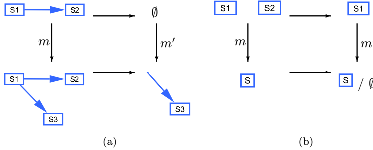
Figure 9.5: Problematic rules
