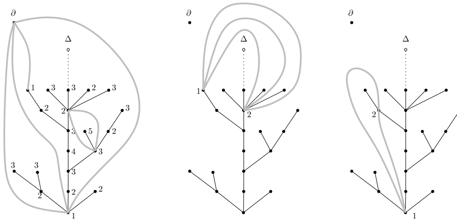
Figure 3.3: Construction of a few edges in Schaeffer's correspondence.
