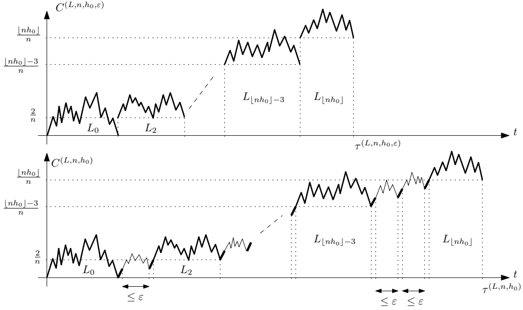
Figure 3.5: The processes C^{(L,n,h_0)} and C^{(L,n,h_0,\varepsilon)} .
