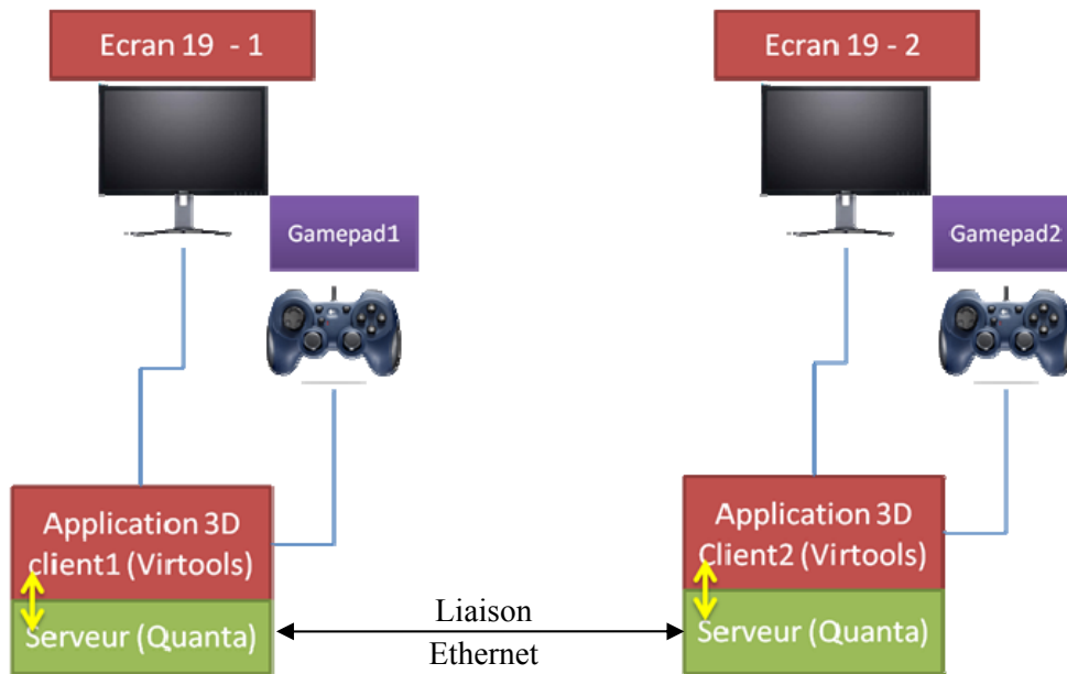
Figure 28 : Architecture logicielle
