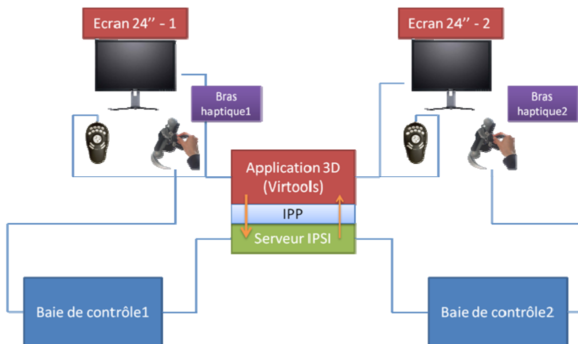
Figure 53 : Architecture logicielle
