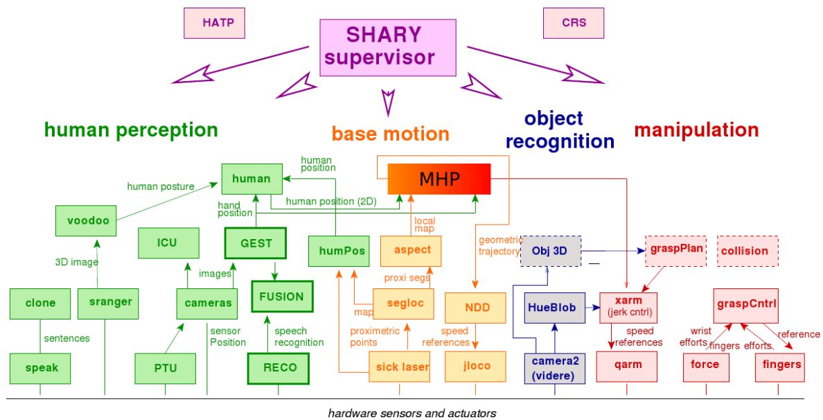
Figure 4.1: The whole architecture. Modules in the superior part (SHARY, HATP, CRS) belong to the decisional layer. In the lower part are shown all the modules of the functional layer (categorized on task types).
