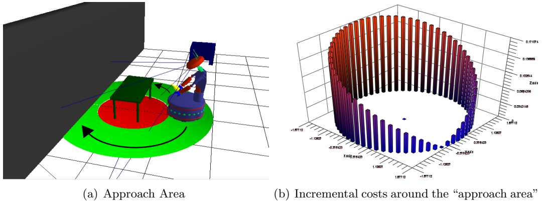
Figure 3.24: For objects the area of interaction is called approach area, and is defined illustrated as the green band that turns the object all around. The costs will depend on the robot current position.
