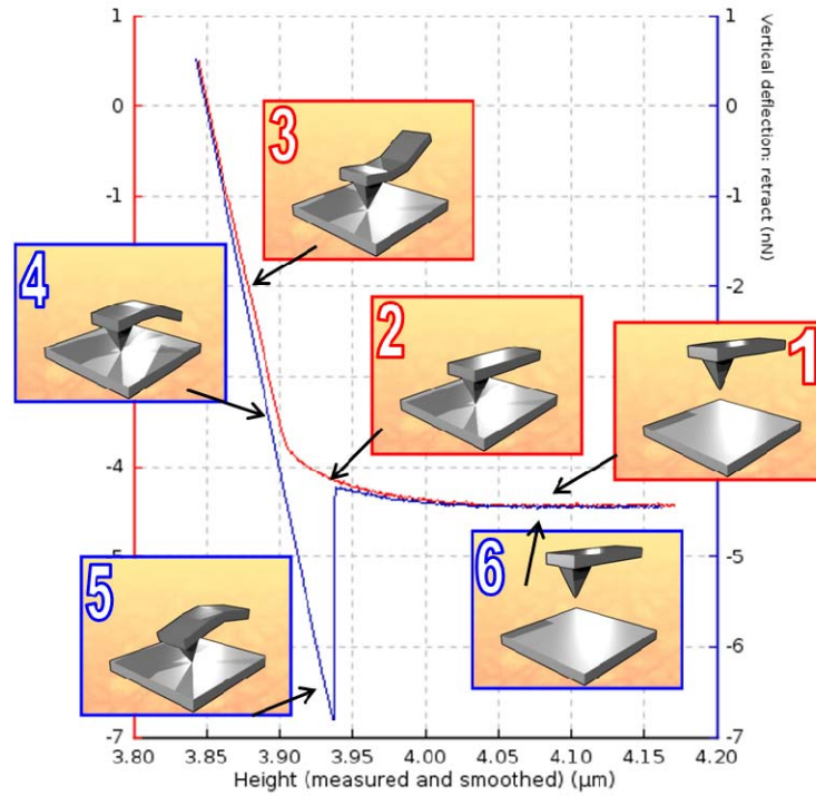
Figure 13A: Force spectroscopy principle. The AFM system records the vertical deflection of the AFM probe during a cycle of approach and retraction of the tip. These measurements can be divided into 6 steps. 1/ the AFM probe approach the surface but ‘feels’ no attractive or repulsive force. 2/ the probe ‘contacts’ the surface...3/..and starts to bend due to the resistivity of the material, generally glass slide, mica or silica. The vertical deflection increased proportionally to the force applied on the probe. 4/ the probe start to retract from the surface and the cantilever bends due to the adhesion force between the surface and the probe. 5/ the cantilever bends until it pulls out from the surface...6/..And comes back to a position where no interactions are felt by the AFM probe.
