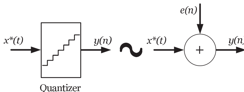
Figure 2.3: Quantizer linear model.
