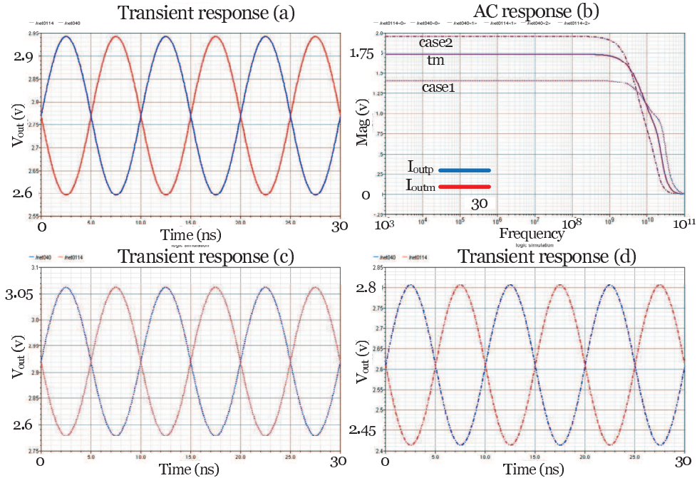
Figure 6.27: Transient response of the output voltage for the typical mean values (a), the first worst case (c) and the second worst case (d) and the AC response for the same cases for the unloaded CTOV.
