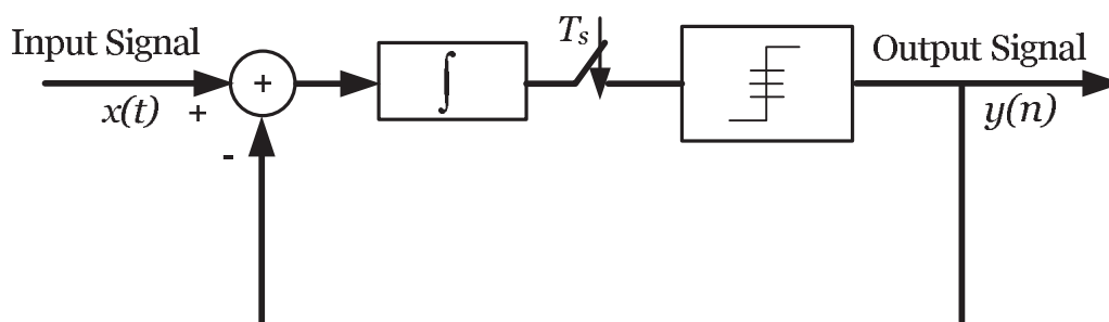
Figure 2.9: \Sigma\Delta modulation.
