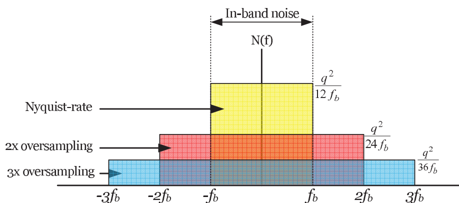
Figure 2.7: Comparison the in-band noise of Nyquist-rate ADCs and that of oversampling ADCs.
