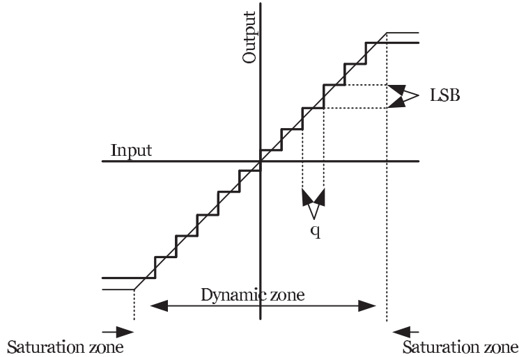
Figure 2.2: Quantization principle.
