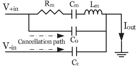
Figure 4.11: Principle of anti-resonance cancellation.
