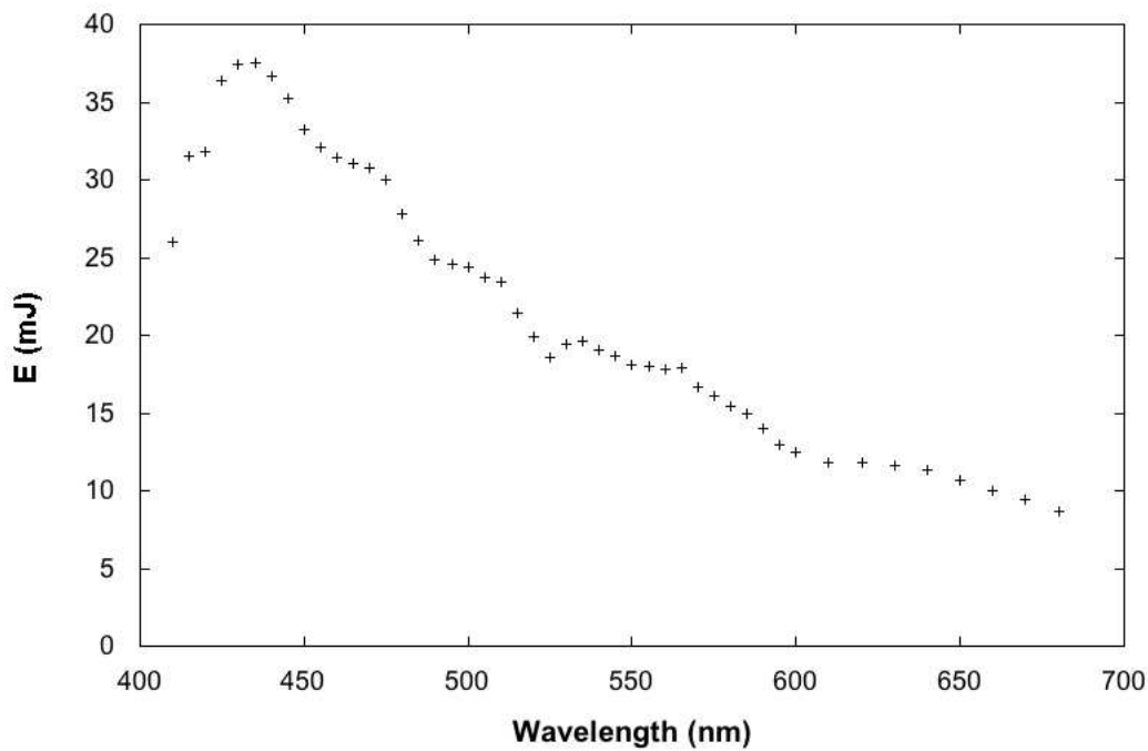
Figure 2.15: Panther EX OPO output mean energy per pulse measured in the visible range as a function of wavelength.
