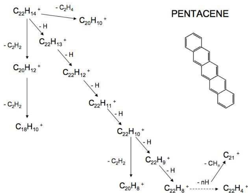
Figure 3.7: Top: FT-ICR mass spectrum of the pentacene cation after 1 minute of irradiation with the Xe arc lamp. The zoom on the spectrum evidences the presence of two separate peaks at slightly different m/z values: m/z = 252.00 ( C_{21}^+ ) and m/z = 252.09 ( C_{20}H_{12}^+ ). Bottom: identified pentacene photodissociation paths.
