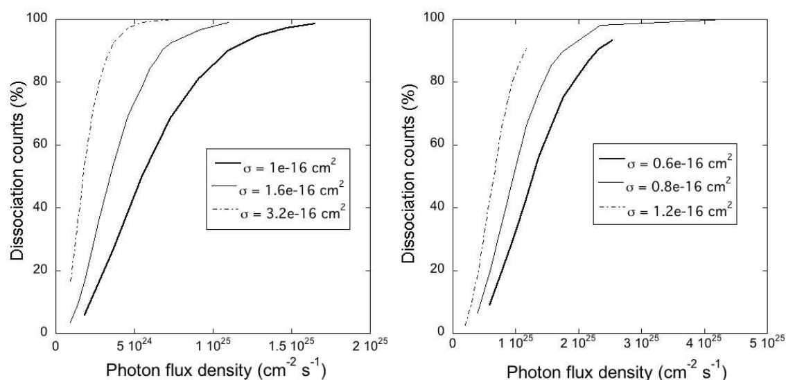
Figure 4.13: Relative dissociation counts as a function of the photon flux density obtained from the model considering different values for the absorption cross-sections, for pyrene cation (left panel) and coronene cation (right panel).
