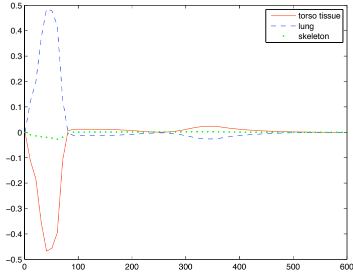
Figure 7.1: The normalized parameter derivatives of the electrocardiogram: \sigma_t \partial_{\sigma_t} ECG (red, continuous line) for the tissue derivative, \sigma_l \partial_{\sigma_l} ECG (blue dashed line) for the lung derivative and \sigma_b \partial_{\sigma_b} ECG (green, dotted line) for bones (skeleton)
