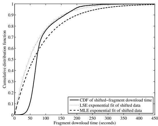
(c) Exponential fit of the shifted fragment download time distribution
