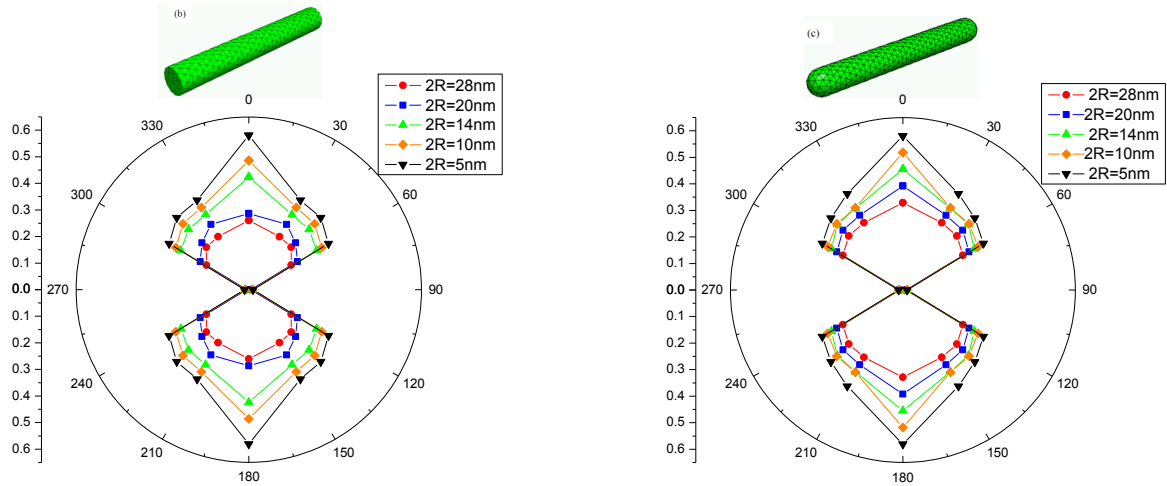
Figure 4.11: Evolution of the coercivity \mu_0 H_C as a function of the angle between the applied field and the easy axis for nanowires (object of type b) and capped nanowires (object of type c). The results from the simulations are compared for various values of diameter.
