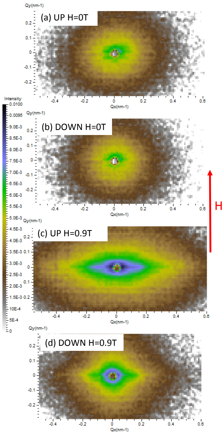
Figure 8.7: Scattering 2D spectra for : (a) neutrons polarized |+\rangle (UP) for H = 0T (b) neutrons polarized |-\rangle (DOWN) for H = 0T (c) neutrons polarized |+\rangle (UP) for H = 0.9T (d) neutrons polarized |-\rangle (DOWN) for H = 0.9T .
