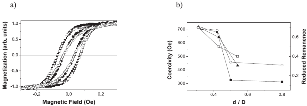
Figure 1.21: (a) Hysteresis loops as a function of the nanowire diameter for Ni nanowires separated 105 nm having diameters of 35 nm (■), 44 nm (□), 53 nm (●) and 83 nm (○). (b) Dependence of coercivity [membranes prepared in oxalic (■) and sulphuric (▲) acids] and reduced remanence [oxalic (○) and sulfuric membranes (□)] as a function of the ratio diameter to interwires distance d/D . From [Vaz2004].
