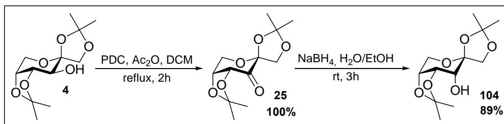
Scheme 65
