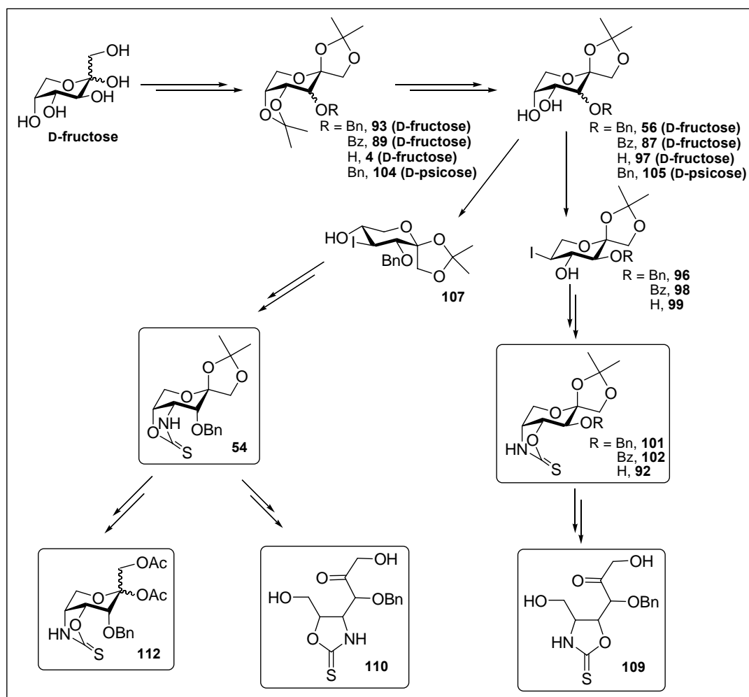
Scheme 83
