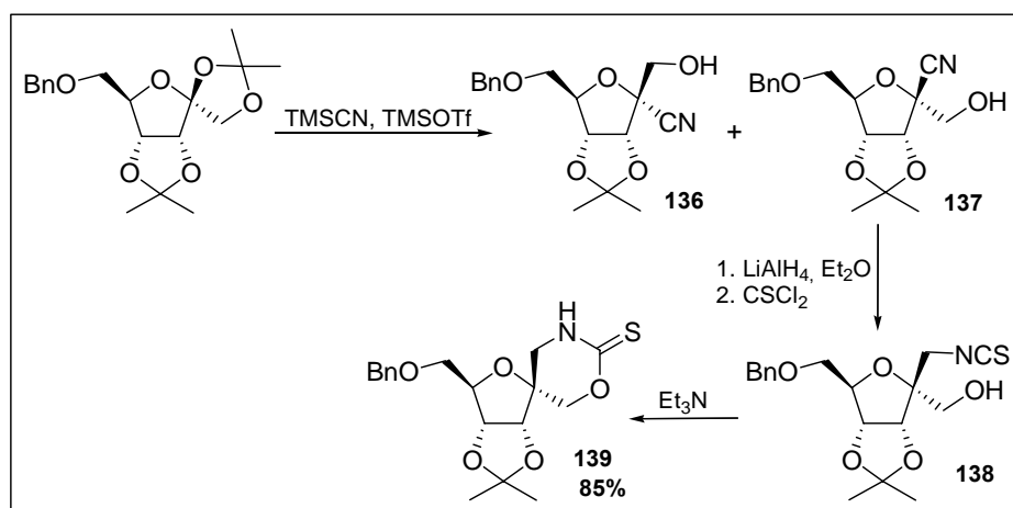
Scheme 92
