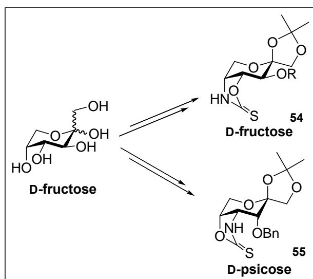
Scheme 45
