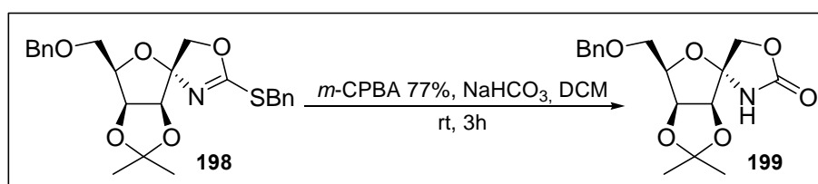
Scheme 122
