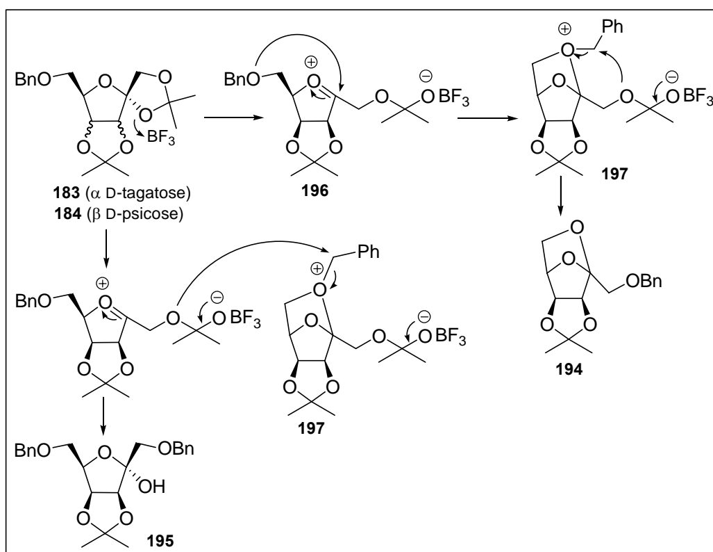
Scheme 120
