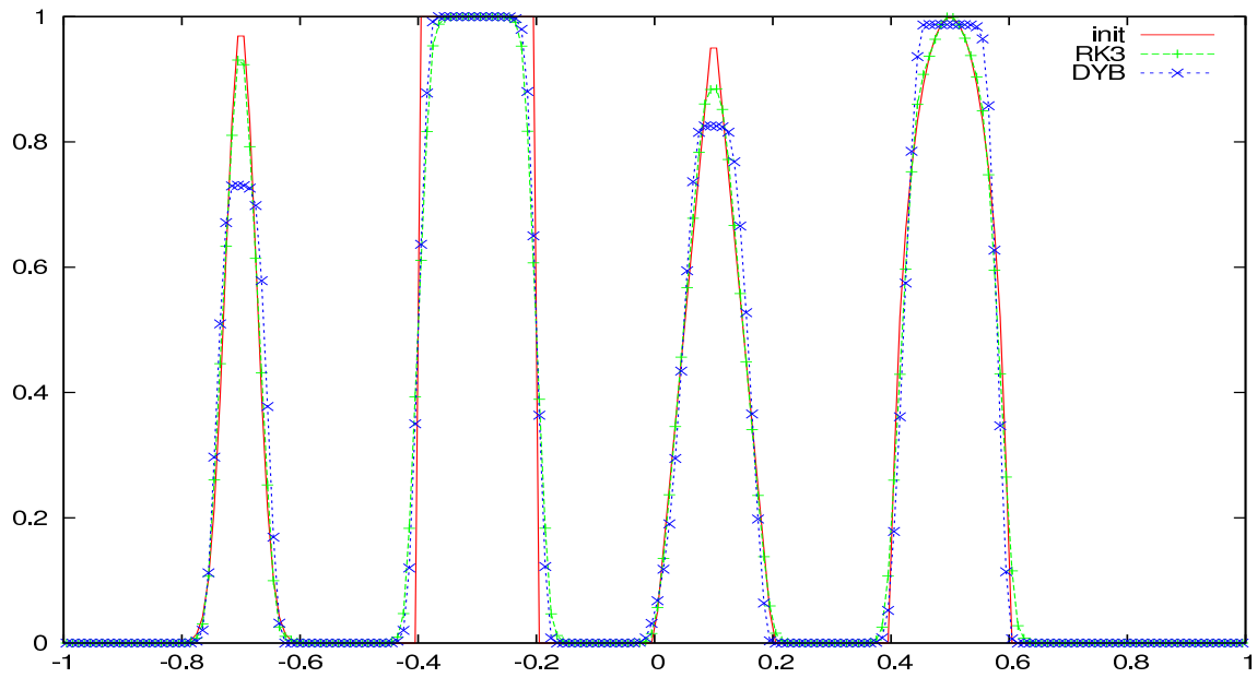
Figure 3.8: Comparison of free transport between the formal fourth order scheme issued from Daigugi, Yamamoto, and Berthon (DYB, blue), an exact third order Discontinuous Galerkin scheme from P.-H. Maire [18], with suitable slope limiters (RK3, green). The initial solution is the bold red curve. 200 grid points discretize the [-1,1] computational domain. The CFL condition is 1/5 , with 400 time steps until the final time t_{end} = 8 , when the solution of the transport equation (with velocity v = 1 ) is represented with green and blue curves.
