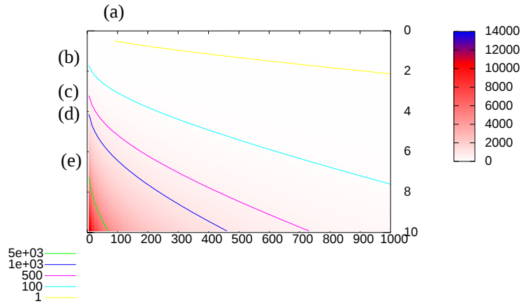
Figure 8.1: Production rate (\nu_{io}n_b)^{-1}dn_b/dt of secondary electrons by a beam electrons propagating in a 5 keV Maxwellian thermal plasma as a function of the beam energy and the energy cut-off parameter. Isolines 1, 100, 500, 1000, 5000 for the production rates are labelled with respective letters (a)-(e).
