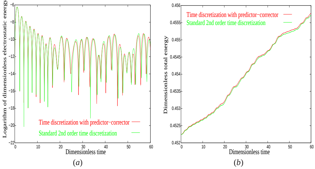
Figure 3.6: Nonlinear relativistic Landau damping for a 64 \times 64 grid resolution. The evolution of the logarithm of the discrete, dimensionless total electrostatic energy (a) and discrete, dimensionless total energy (b) is shown against time.
