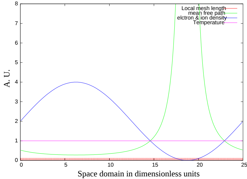
Figure 6.6: Initial profiles for electron and ion densities, electron temperature. The discretization is uniform in space and velocity. The discretization in space resolves the mean free path. For this particular configuration, \frac{n_{ref}}{n_c} = 2 , Z = 1 , n_x = 200 , n_{v_x} = n_{v_y} = n_{v_z} = 32 , v_{max} = 6 , L = 25
