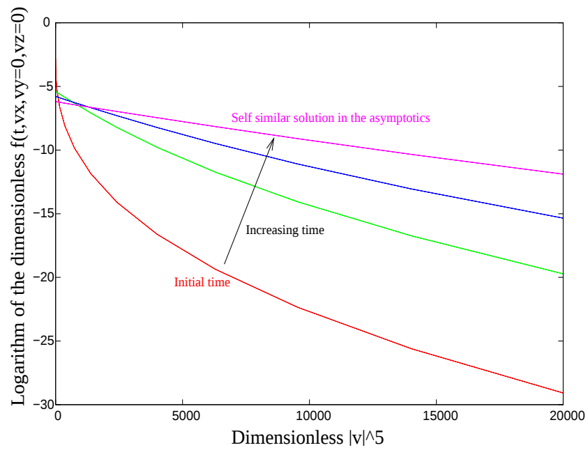
Figure 6.2: Dimensionless f(t, v_x, v_y = 0, v_z = 0) at different times. The final straight line denotes a super-gaussian dependance on the velocity dimension. Negative and positive velocities are surimposed, which shows the perfect conservation of the isotropic geometry at any time.
