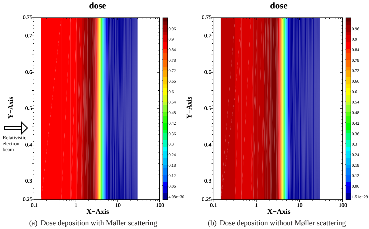
Figure 7.10: The role of the relativistic electron inelastic collisions on dose deposition in water phantom
