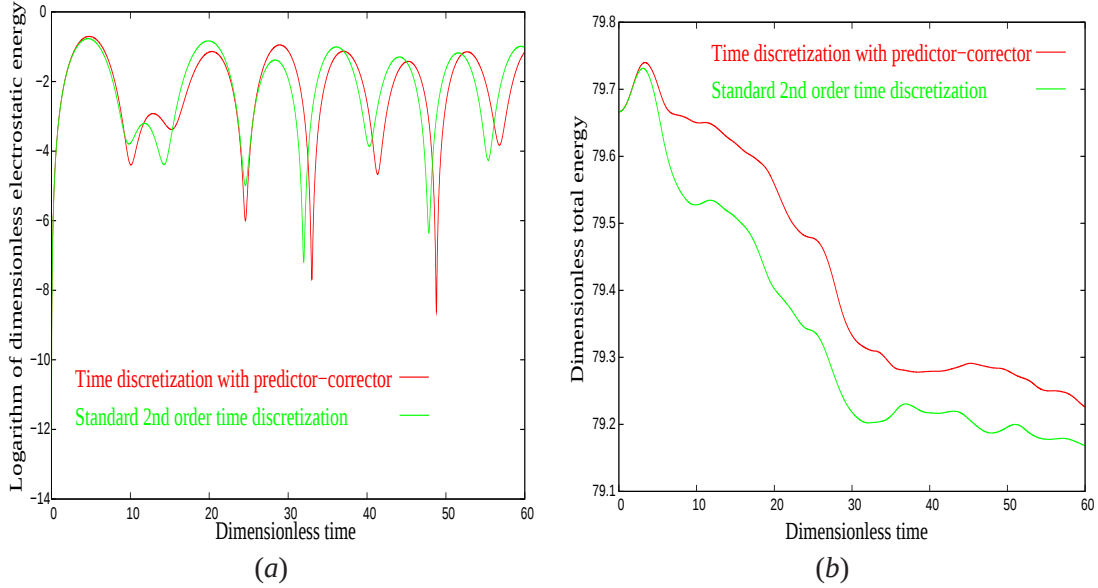
Figure 3.7: Nonlinear relativistic two-stream instability for a 32 \times 32 grid resolution. The evolution of the logarithm of the discrete, dimensionless total electrostatic energy (a) and discrete, dimensionless total energy (b) is shown against time.
