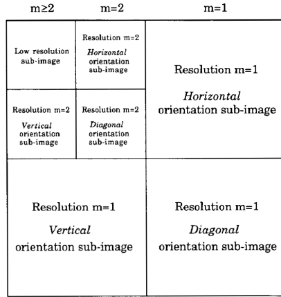
Fig. 6. Image decomposition.
