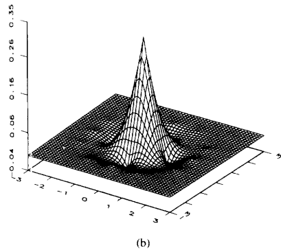
Fig. 4. (a) Scaling function associated with monodimensional nine taps filters; (b) seven taps filters.
