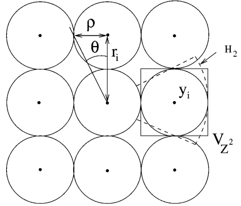
Fig. 3. \mathbb{Z}^2 lattice with packing radius \rho . The approximation consists in integrating over the domain H_2 (dashed lines) instead of the squared Voronoi V_{\mathbb{Z}^2} .
