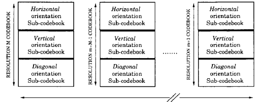
Fig. 12. Multiresolution codebook.
