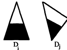
Fig. 2. Histogram-based classification.
