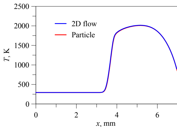
Figure IV.31 Gas and particle temperature distributions along the axis.
