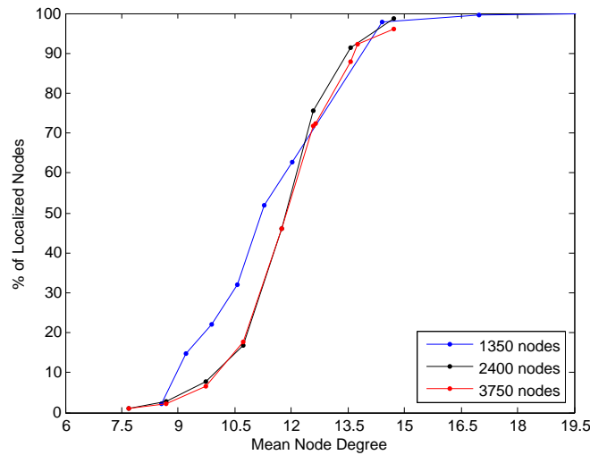
Figure 5.3: OBP: Critical Node Degree for Large Networks
