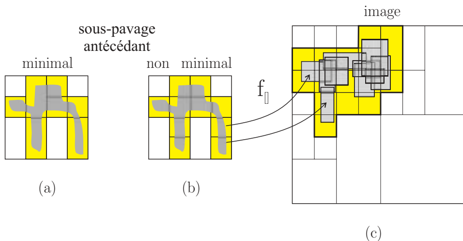
Figure 5-7: Comportement d' ImageSp .
