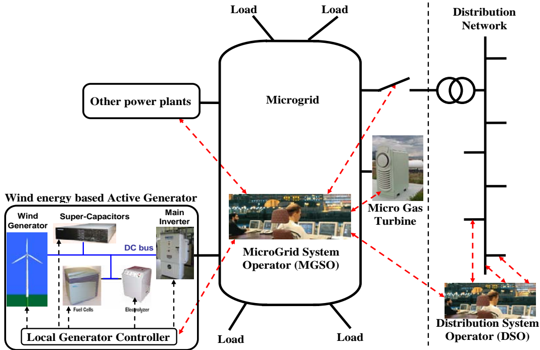
Figure V-21: Studied microgrid
