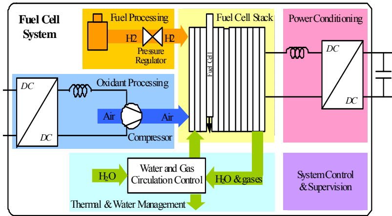
(b) Operation principles of the studied fuel cell system
