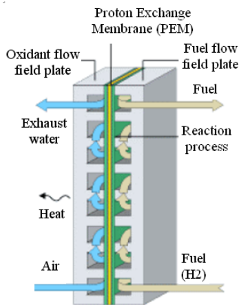
(a) Operation of a fuel cell [Pri 02]
