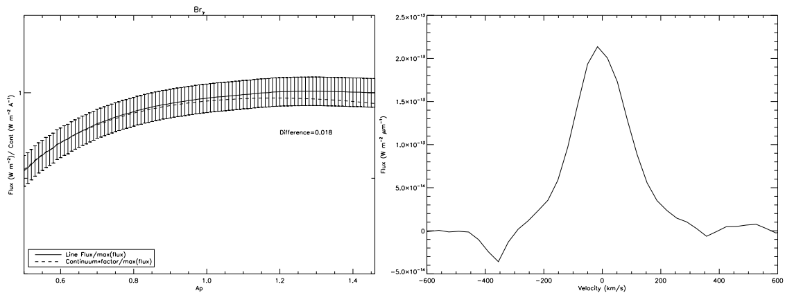
Figure 6.25: Left: Br γ flux integrated in different aperture radius (solid line), compared to its local continuum (dashed line). Both curves are normalized to the maximum emission in Br γ and the continuum curve is normalized to Br γ one at small apertures. Right: Br γ profile integrated in an aperture of 1.46". This profile is integrated to derive the line luminosity.
