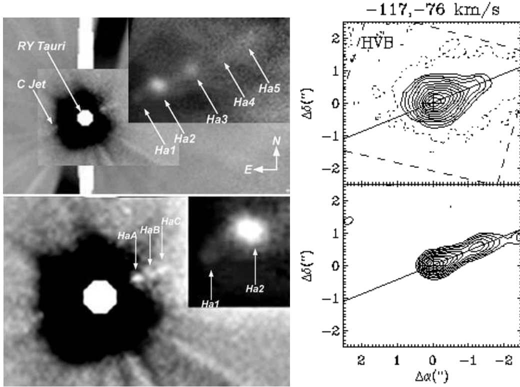
Figure 5.1: Left: Figure adapted from St-Onge & Bastien (2008) showing the RY Tau jet detected in H_{\alpha} emission, out to several arcminutes. Right: The detected high velocity blue component detected in [OI] (this work) at spatial scales of several arcsecs for comparison.
