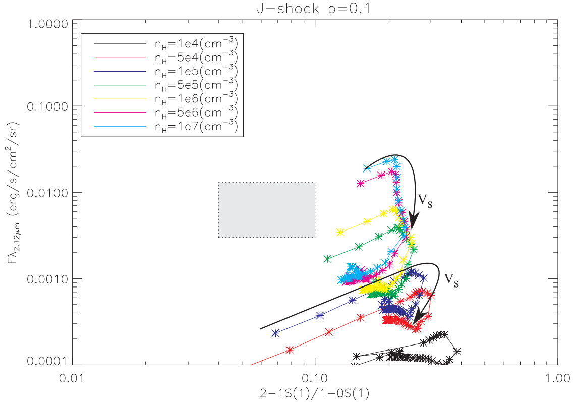
Figure 6.34: Computed H_2 brightness in the 1-0 S(1) ( \lambda=2.12\mu\text{m} ) line against the computed 2-1 S(1)/1-0 S(1) ratio by Kristensen et al. (2008) for J-shocks. The direction of increasing v_s is shown. The gray cube shows the observed measurements indicating that J-shocks are not valid in this case.
