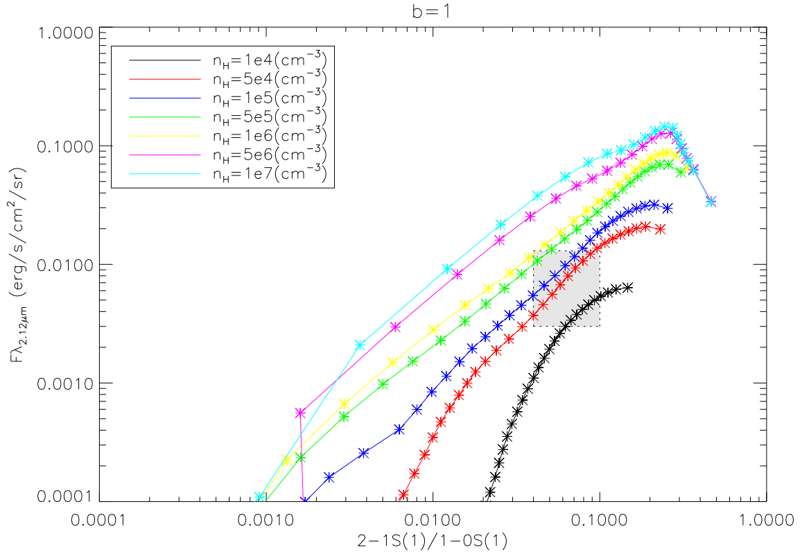
Figure 6.36: Same as Fig. 6.35 but for a C-shock with b=1.0 .
