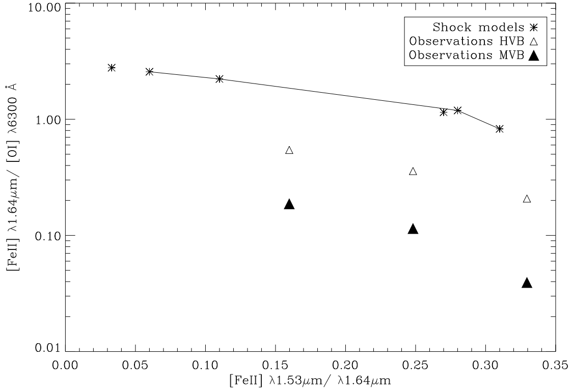
Figure 6.29: [\text{FeII}]\lambda 1.64\mu\text{m}/[\text{OI}]\lambda 6300\text{\AA} ratio against the [\text{FeII}]\lambda 1.53\mu\text{m}/[\text{FeII}]\lambda 1.64\mu\text{m} ratio indicative of the electron density. [OI] observational points are obtained from Lavalley-Fouquet et al. (2000) and shocks models are those of Hartigan et al. (2004). Models with the same n_H=10^4 are connected.
