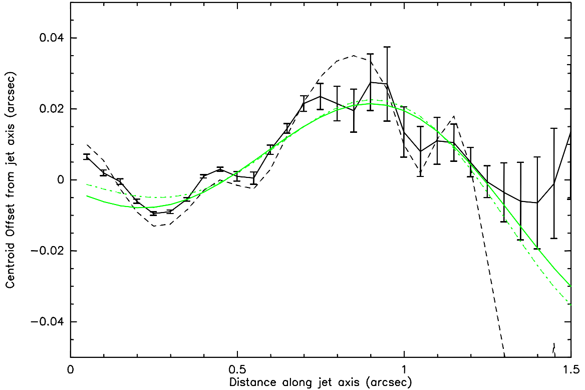
Figure 6.28: Observed wiggling in black, fit to an orbital motion in solid green line and to a jet axis precession in dot-dashed green line.
