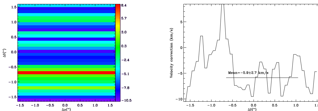
Figure 6.7: Left: Velocity correction, for each slit, measured from a Gaussian fit on a combination of the four OH lines detected around the \text{H}_2\lambda 2.12\mu\text{m} line. Right: A cut in the Y direction of the detector. An average value was used to correct the wavelength calibration in this spectral region.
