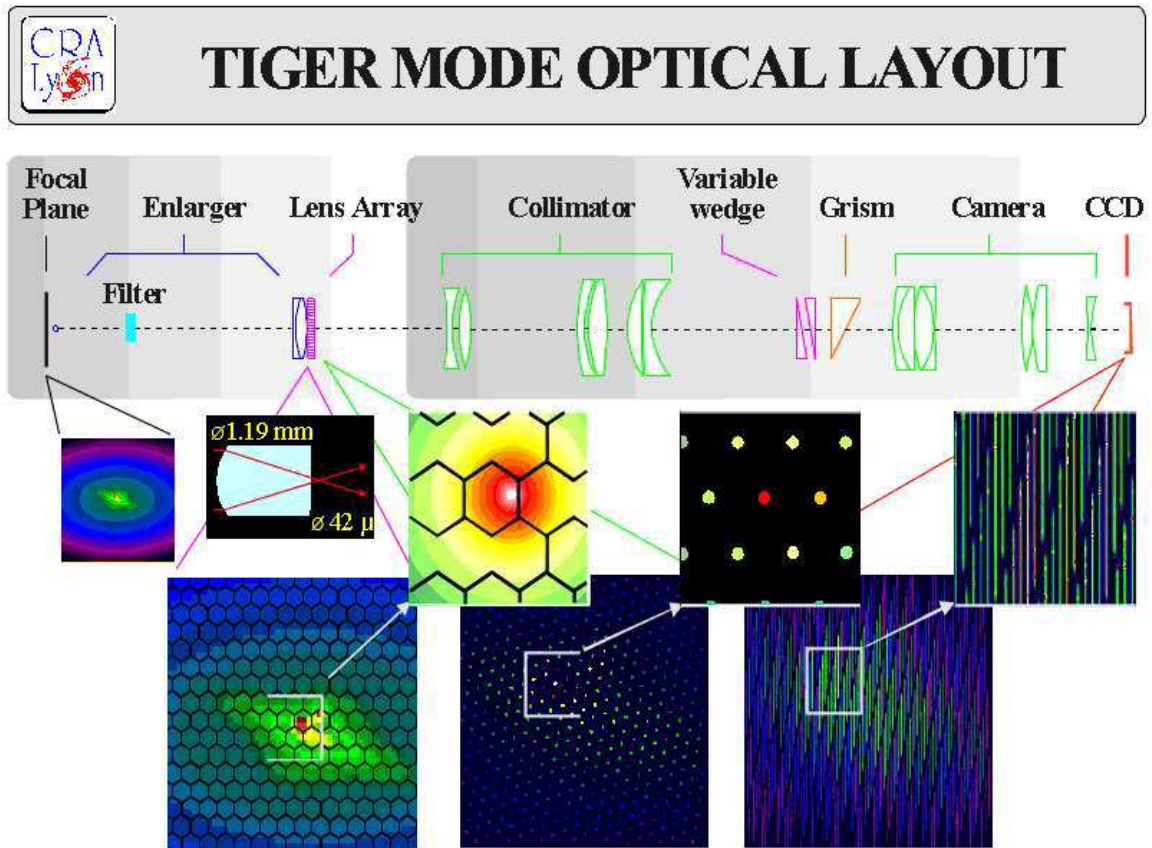
Figure 4.3: Schema of the optical path for the instrument OASIS.
