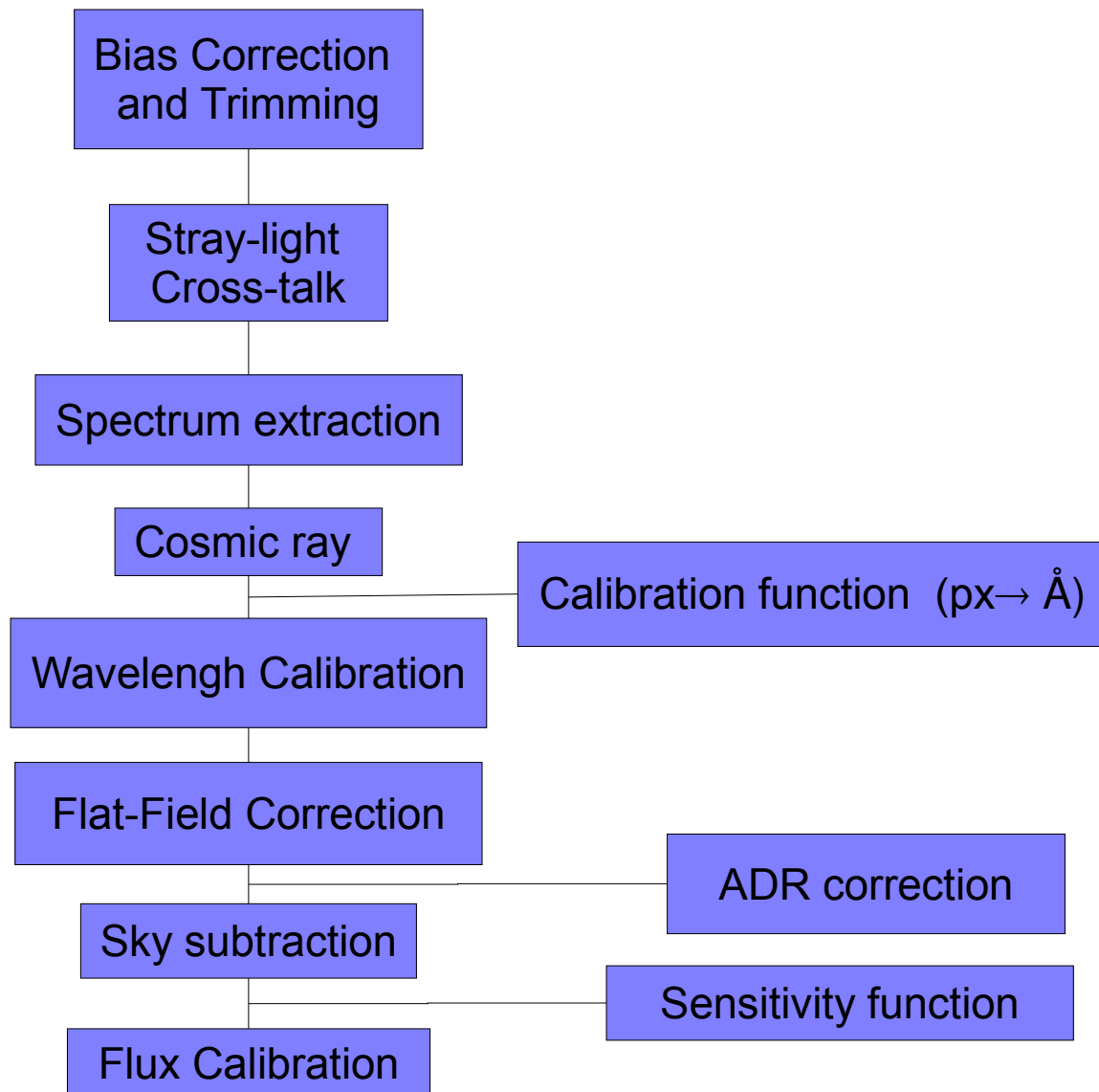
Figure 4.5: General steps for a data reduction of IFS.
