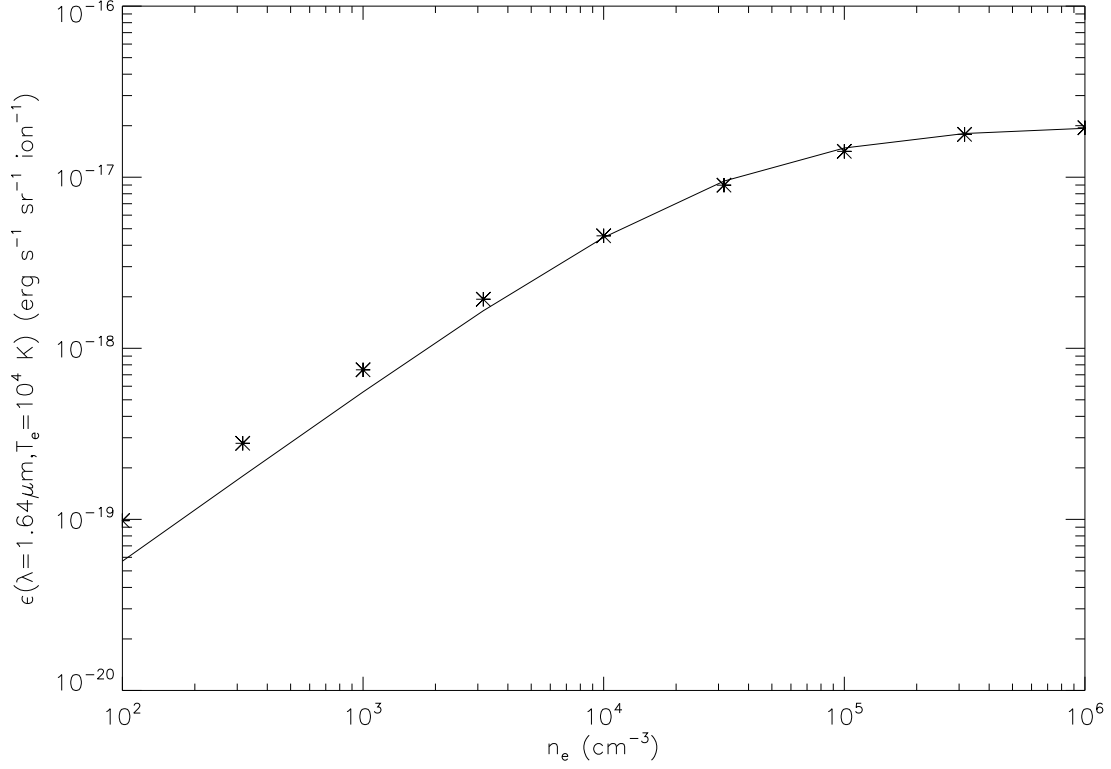
Figure 3.10: Computed emissivity by Pesenti et al. (2003) for [FeII] \lambda 1.64\mu\text{m} line at an electron temperature T_e , of 10^4 K, as a function of the electron density, n_e . Points are the computed values and the line over-plotted is the fit used in our estimations of mass flux (see text).
