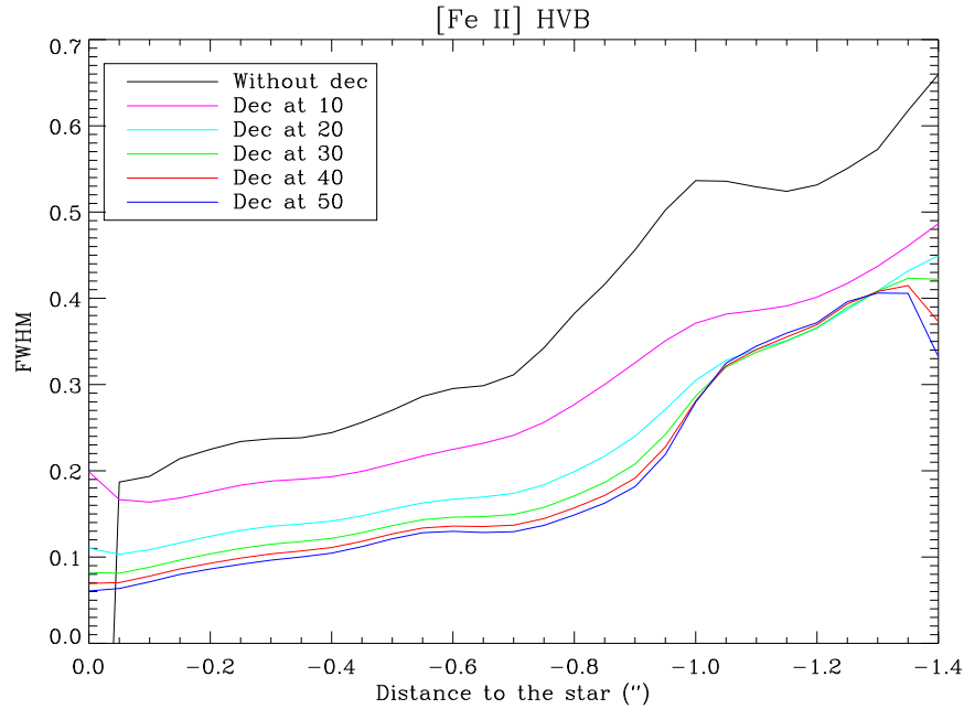
Figure 6.14: Measured FWHM of the jet on the different HVB [FeII] images resulting from different numbers of iterations in the deconvolution process. The maximum number was fixed at 40 iterations in the following.
