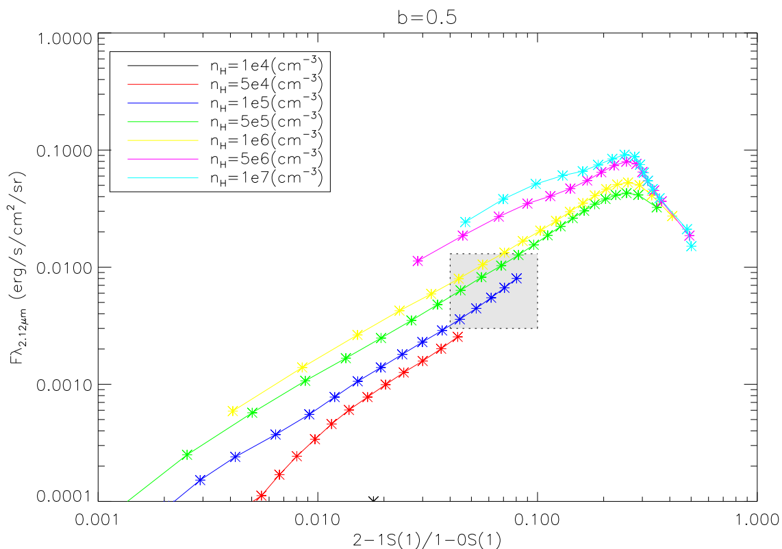
Figure 6.35: Computed brightness in the \text{H}_2\lambda_{2.12\mu\text{m}} line against the computed 2-1 S(1)/1-0 S(1) ratio from models by Kristensen et al. (2008). Different colors correspond to different values of hydrogen density, n_H=1\times 10^4 \text{cm}^{-3} , 5\times 10^4 \text{cm}^{-3} , 1\times 10^5 \text{cm}^{-3} , 5\times 10^5 \text{cm}^{-3} , 1\times 10^6 \text{cm}^{-3} , 5\times 10^6 \text{cm}^{-3} and 1\times 10^7 \text{cm}^{-3} , and the small gray cube shows the observational values. This model is for a C-shock with b=0.5 .
