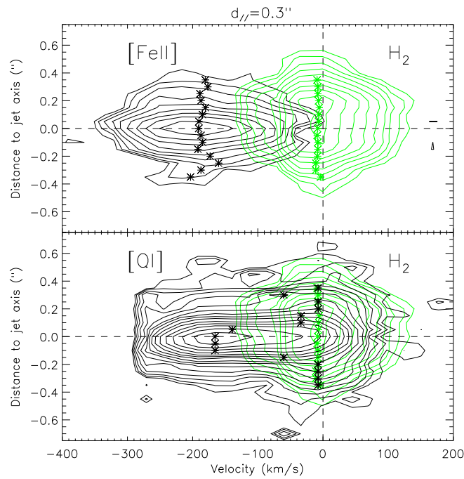
Figure 6.24: Top panel: Transverse PV diagram for the [FeII] \lambda 1.64\mu\text{m} in black, H 2 \lambda 2.12\mu\text{m} in green contours. Bottom panel: [OI] \lambda 3600 (data from Coffey et al. (2008), provided by Dr. Coffey) in black contours and H 2 \lambda 2.12\mu\text{m} in green contours. Centroid velocities from an one-component Gaussian fit are shown with asterisks (black for the iron and the [OI], green for the H 2 ).
