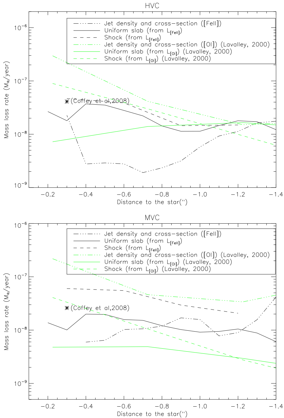
Figure 6.33: Same as Fig. 6.32 (models depending on the luminosity were corrected by iron depletion) but values obtained by Lavalley (2000), using the optical line [O I] \lambda 6300 \text{ \AA} and the same methods, are showed for comparison.
