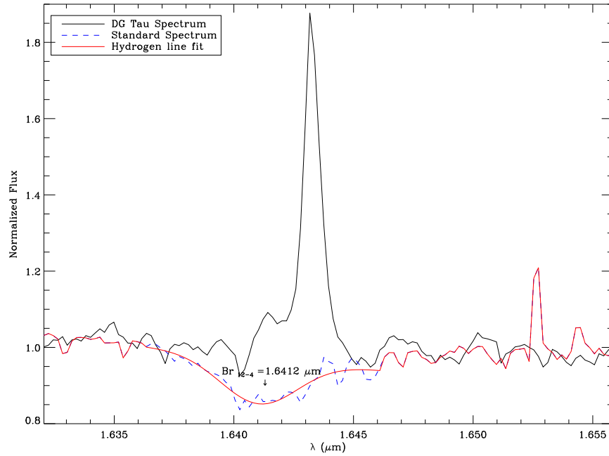
Figure 6.8: Spectrum at \alpha \sim 0'' and \delta \sim 0.5'' showing clear jet emission in the [\text{FeII}]\lambda 1.64\mu\text{m} line. The telluric standard star spectrum is over-plotted, in dashed line, and in red solid line the fit to the Brackett Hydrogen line at 1.6412\mu\text{m} is also included. Both spectra are normalized to the continuum. Telluric absorption lines contribute less than 7% to the emission.
