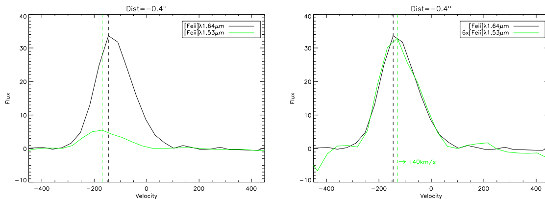
Figure 6.2: Velocity calibration problem: line profiles for \lambda 1.53\mu\text{m} (green) and \lambda 1.64\mu\text{m} (black) lines at a distance of 0.4'' from the star in the blue jet. Two lines show a shift of almost 50 km/s. Left: profiles after continuum subtraction. Right: same profiles but the \lambda 1.53\mu\text{m} profile was multiplied by 6 and shifted of 40 km/s to show the similarity between the two profiles.
