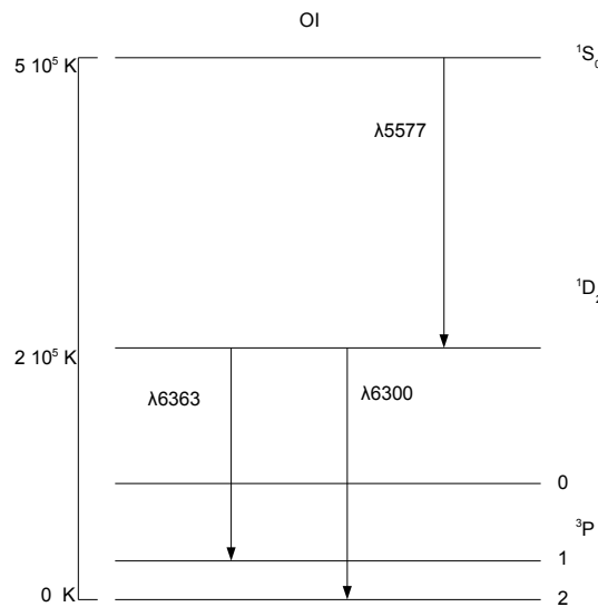
Figure 3.3: Energy level diagram of the neutral oxygen, [OI], with the main optical forbidden emission lines (wavelengths in \text{\AA} ), adapted from Lavalley (2000).
