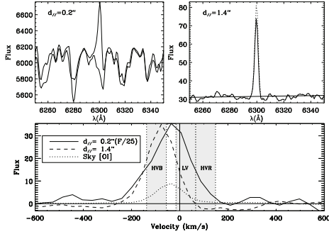
Fig. 2. Top panels: solid curves show the observed OASIS [O I] 6300 Å spectra (thick lines) and the fitted continuum (thin lines) towards the blueshifted jet, offset by 0.2'' ( top-left ) and 1.4'' ( top-right ) from the star. Profiles before subtraction of the [O I] atmospheric line are shown with a dotted line (same as solid thick curve at 0.2'' ). Bottom panel: residual continuum-subtracted [O I] line profiles at 0.2'' and 1.4'' from the star. The subtracted [O I] atmospheric line is shown as a dotted curve. The profile at 0.2'' is divided by 25 for clarity. Velocity intervals contributing to the HVB, LV and HVR channel maps of Fig. 3 are shaded.
