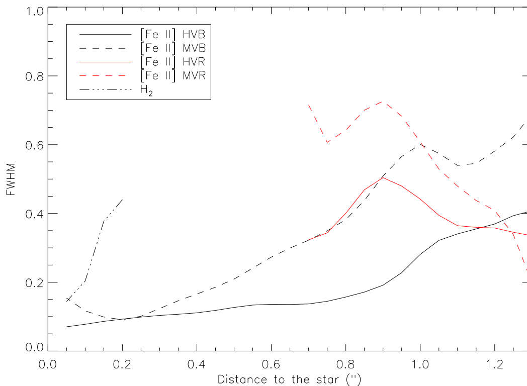
Figure 6.16: Jet width for both the [FeII] and the H_2 emission, respect to the projected distance from the star, derived from deconvolved channels maps of Fig. 6.12. Atomic HVC is in solid line and the MVC is in dashed line (black for the blue jet and red for the red one). H_2 width is in dashed double-dotted line.
