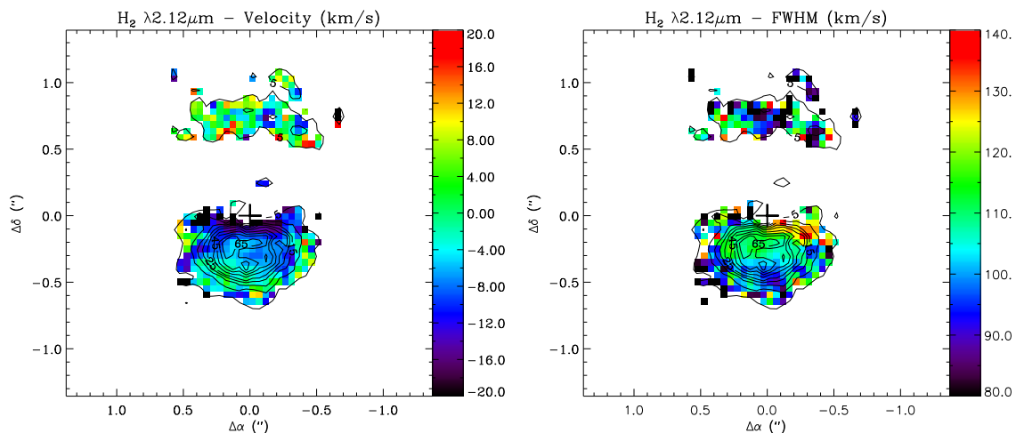
Figure 6.19: Same as Fig. 6.18 but for the \text{H}_2\lambda 2.12\mu\text{m} emission line.
