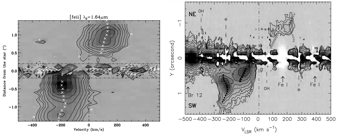
Figure 6.21: Left: Position-velocity map in the [FeII] \lambda 1.64\mu\text{m} line, after continuum subtraction, for a 1'' wide pseudo-slit and sampled every 0.1'' . Contours start at 2.43 \times 10^{-15} \text{ W m}^{-2} \mu\text{m}^{-1} (")^{-2} and increase by factors of \sqrt{2} . Negative contours are shown with dashed lines. The white contour shows the SNR=3 level calculated on each average profile and crosses show the centroid velocity derived from a Gaussian fit. At distances \pm 0.2'' , the PV are very affected by continuum subtraction residuals. Right: PV diagram shown by Pyo et al. (2003) for comparison, see text.
