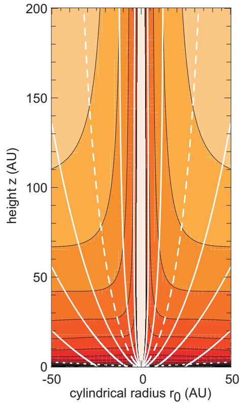
Figure 6.38: Overall geometry of the MHD disc wind solution of Casse & Ferreira (2000) used in the predictions by Panoglou et al. (2009). Solid curves show flow lines and the color scale shows the density. The white line denotes the slow magneto-sonic wind surface at z \simeq 0.05r .
