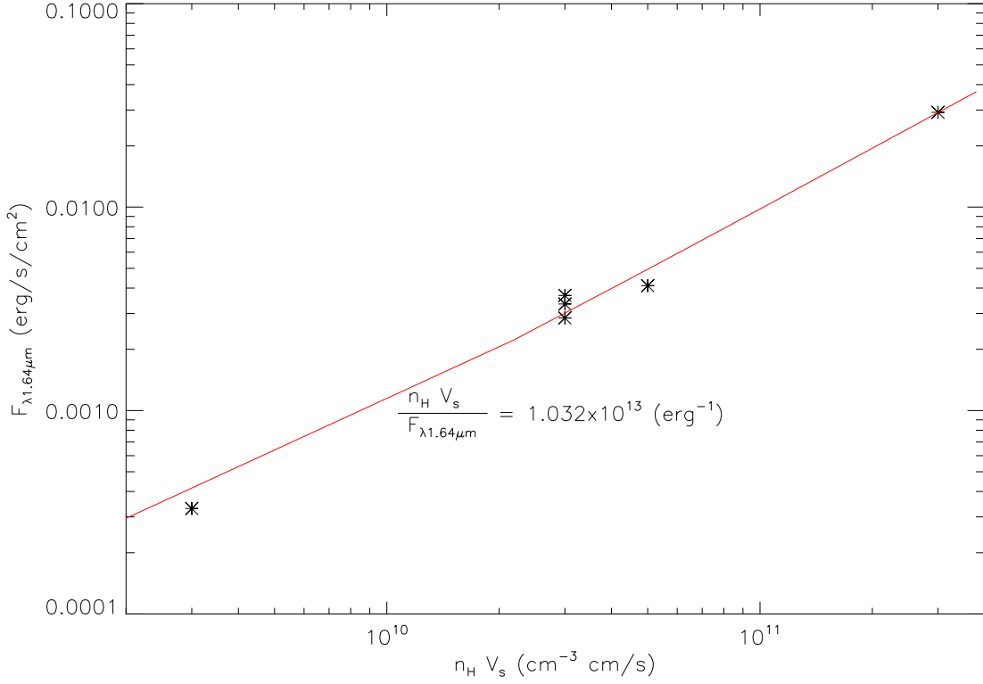
Figure 3.11: Flux in the [FeII] \lambda 1.64\mu\text{m} line predicted by shock models computed by Hartigan et al. (2004) against the product of n_H V_s (input parameters). The flux given is what emerges out the front of shock. We find a good agreement with a linear fit, also over-plotted. We use this proportionality to estimate the mass-loss rate in the shock (see Eq. 3.40 and the text).
