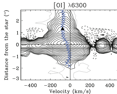
Fig. 6. Position-velocity map along the RY Tau jet in [O I] \lambda 6300 Å after continuum subtraction, for a 1'' wide pseudo-slit sampled every 0''2 along the jet. Centroid velocities derived from a single Gaussian fit are also plotted (blue crosses). Intensity contours start at 3\sigma ( 1.32 \times 10^{-19} W m ^{-2} Å ^{-1} (") ^{-2} ) and increase by factors of \sqrt{2} . Negative contours are shown with dashed lines. The dotted line shows the 5\sigma level, based on the spectral noise in each spectrum. Close to the star, the far wings of the line ( |v| \geq 250 km s ^{-1} ) are affected by continuum subtraction residuals. The location of the jet knot identified in the deconvolved HVB map is indicated by a filled triangle.
