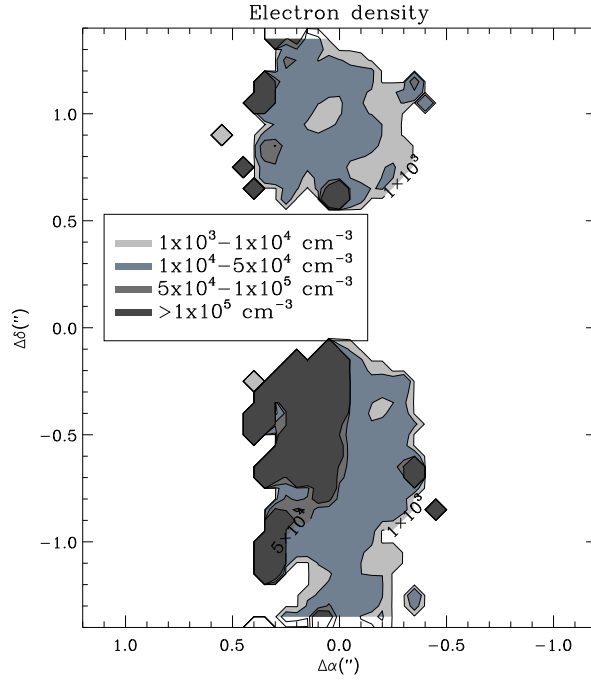
Figure 6.26: Electron density distribution in both the blue and red jet, obtained from the [FeII] \lambda 1.53\mu\text{m}/\lambda 1.64\mu\text{m} ratio and using the calculations of Pesenti et al. (2003). Close to the star, at the East we do not plot contours higher than 1 \times 10^5 \text{ cm}^{-3} because electron density in this region reach the high density limit of 5 \times 10^5 \text{ cm}^{-3} .
