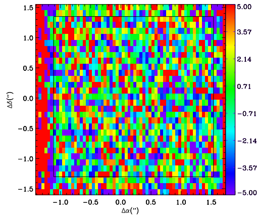
Figure 6.6: Difference between the velocity corrections derived from a linear fit, finally applied to the data, and the velocity corrections measured for each point on the detector. The standard deviation gives a lower limit to the error on the wavelength calibration. It is calculated inside the box because the outer parts of the detector are more noisy.
