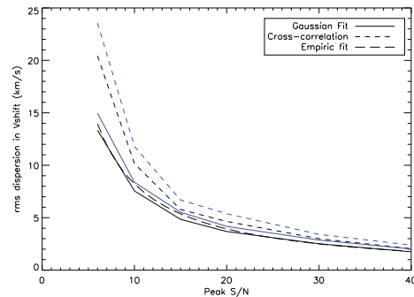
Fig. A.1. 1\sigma error on the velocity shift between two spectra as a function of the signal-to-noise ratio ( SNR ) at the line peak, as modelled from Monte-Carlo simulations. Two measurement methods are presented: cross-correlation of spectra (short-dashed curves) and centroid difference of Gaussian fits (solid curves). The input velocity shift is 10 \text{ km s}^{-1} , and the input profile FWHM is 135 \text{ km s}^{-1} (black curves) and 175 \text{ km s}^{-1} (blue curves). The long dashed curve plots \sigma_{\Delta V} = 90/SNR \text{ km s}^{-1} , the expected theoretical error for infinite sampling (see text).
