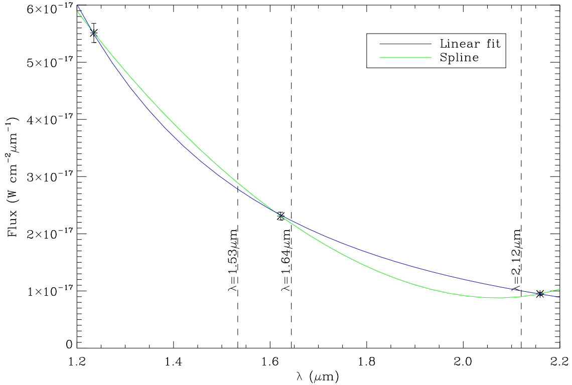
Figure 6.10: Interpolation between the flux calculated from the magnitudes in H, K and J bands from the 2MASS catalogue, for the star HIP 26686 (observed in the H band). Two methods were tested, a spline fit (green) and a linear fit (blue). Finally, the linear fit (in logarithmic scale), expected for a black body emission at this wavelength domain in the Rayleigh-Jeans approximation, was kept.
