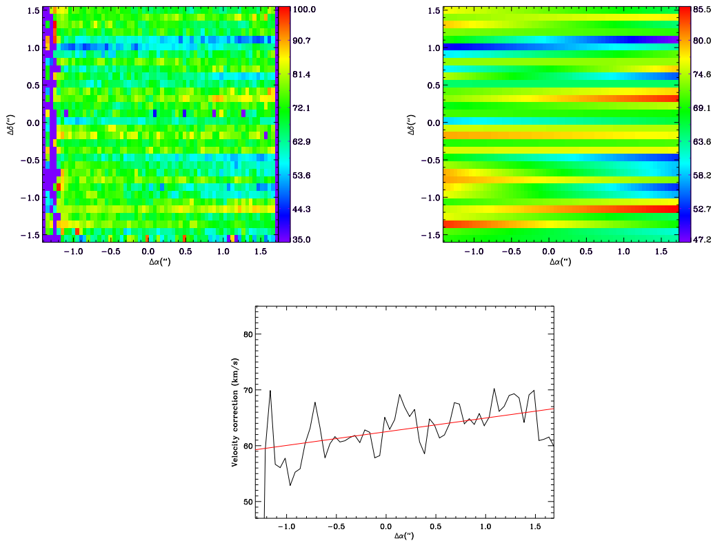
Figure 6.4: Upper-Left: Velocity correction to the previous wavelength calibration to the sky \lambda 1.6692\mu\text{m} line at each spatial position on the detector. Upper-Right: Velocity correction ( \Delta v ) in km/s derived as a linear fit carried out on the X direction of the detector on the previous image. Lower: Example of the fit achieved in one of the central slits.
