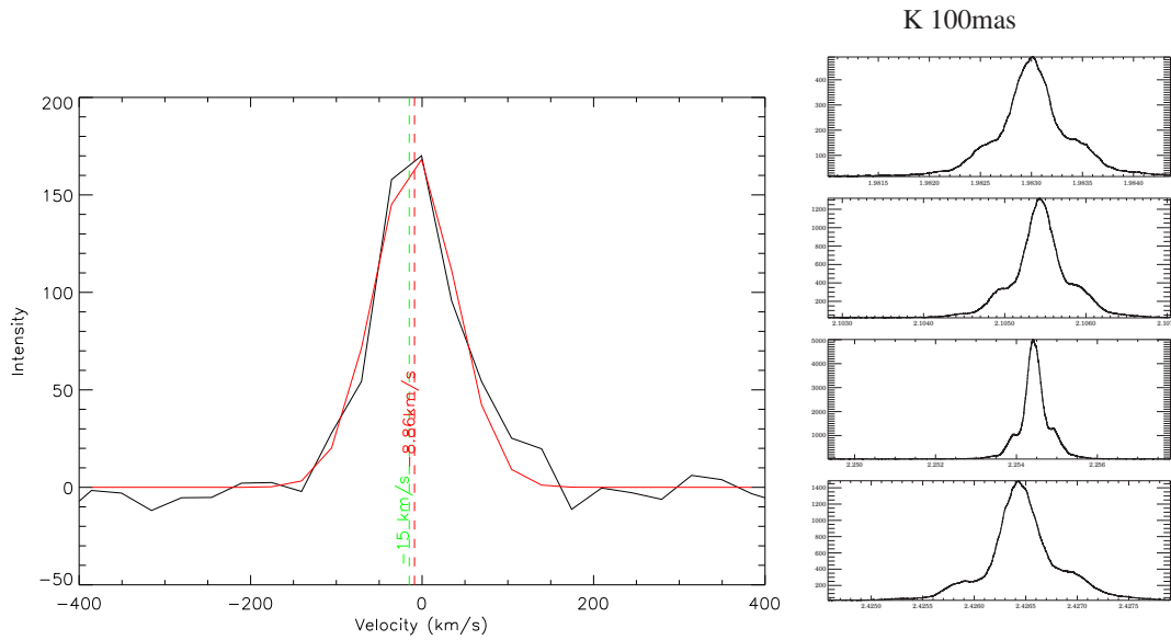
Figure 6.20: Left: Average profile of the H 2 emission, simulating the long-slit observations by Takami et al. (2004). The Gaussian fit to the profile is over-plotted in red. The radial velocity of -15 km/s observed by Takami et al. (2004) and the centroid velocity from the Gaussian fit ( -9 \pm 3 km/s) are also shown. Right: SINFONI spectral PSF in the K band for the plate-scale used in our observations and for different regions on the detector.
