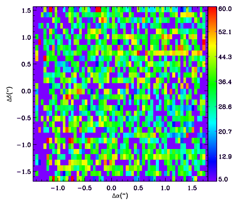
Figure 6.5: Velocity correction to apply in the region of the [\text{FeII}]\lambda 1.533\mu\text{m} line, measured from the OH sky line at \lambda 1.53327\mu\text{m} . The wavelength calibration in this spectral region was not finally corrected because it would introduce more noise to the corrected image.
