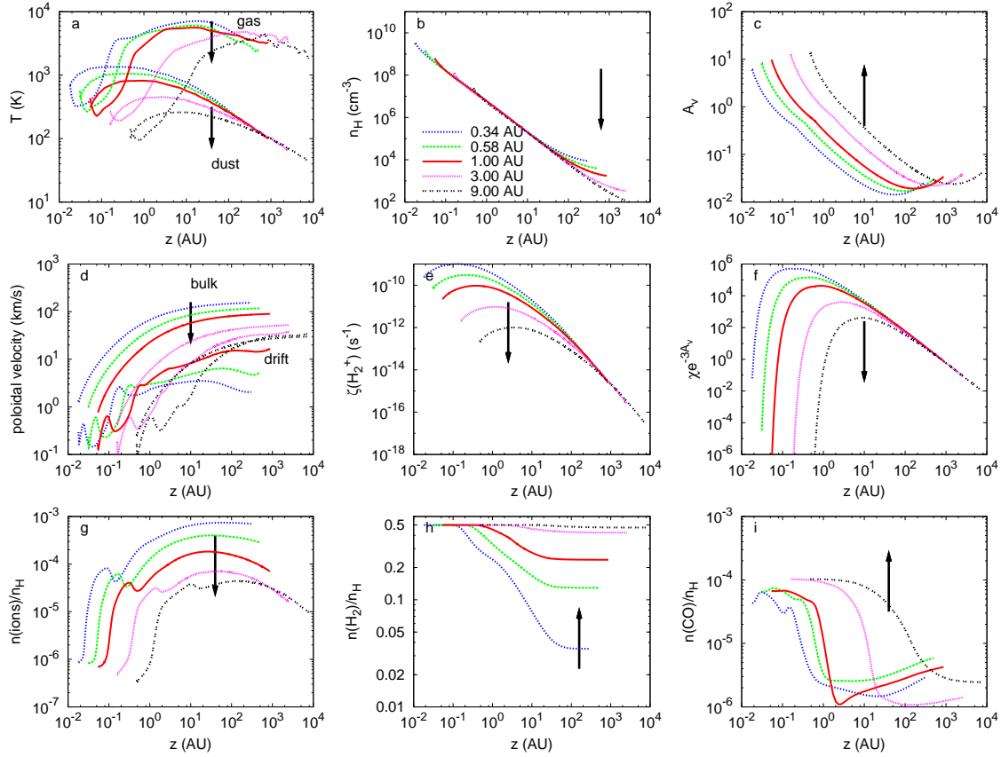
Figure 6.39: Model predictions for a Class II object, \dot{M}_{acc} \sim 10^{-6} M_{\odot}/\text{yr} , and different streamlines launched from 0.34, 0.58, 1.00, 3.00 and 9.00 AU, obtained by Panoglou et al. (2009) (private communication). (a) the gas temperature and dust temperature (lower curves); (b) the number density of hydrogen nuclei; (c) the visual extinction A_v to the star, in magnitudes; (d) the poloidal components of the bulk flow speed (top curves) and the calculated drift speed (lower curves); (e) the X-ray \text{H}_2 ionization rate; (f) the effective radiation field in Draine units (attenuation factor appropriate for carbon photoionisation); (g) the fractional abundance of ions; (h) the fractional abundance of \text{H}_2 ; (i) the fractional abundance of CO.
