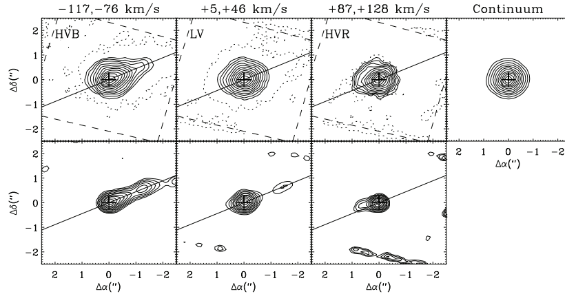
Fig. 3. Continuum-subtracted [O I] 16300 Å emission maps of the RY Tau microjet, both raw ( top panels ) and deconvolved ( bottom panels ). Emission is integrated over three velocity intervals, with the centers of the corresponding velocity channels (each 41 \text{ km s}^{-1} wide) indicated on top. The derived blueshifted jet position angle is plotted as a solid line. The continuum map is displayed in the top-right panel . In the top row , contours start at 2% of the maximum and increase by factors of \sqrt{2} . In the bottom row they start at 0.1% of the maximum and increase by factors of 2. Dotted contours correspond to a signal to noise ratio of 5 for the HVB and LV maps, 3 for the HVR map. The dashed line shows the OASIS field of view. Spatial offsets are relative to the continuum centroid (located with a cross). The spatial sampling used is 0''.1 .
