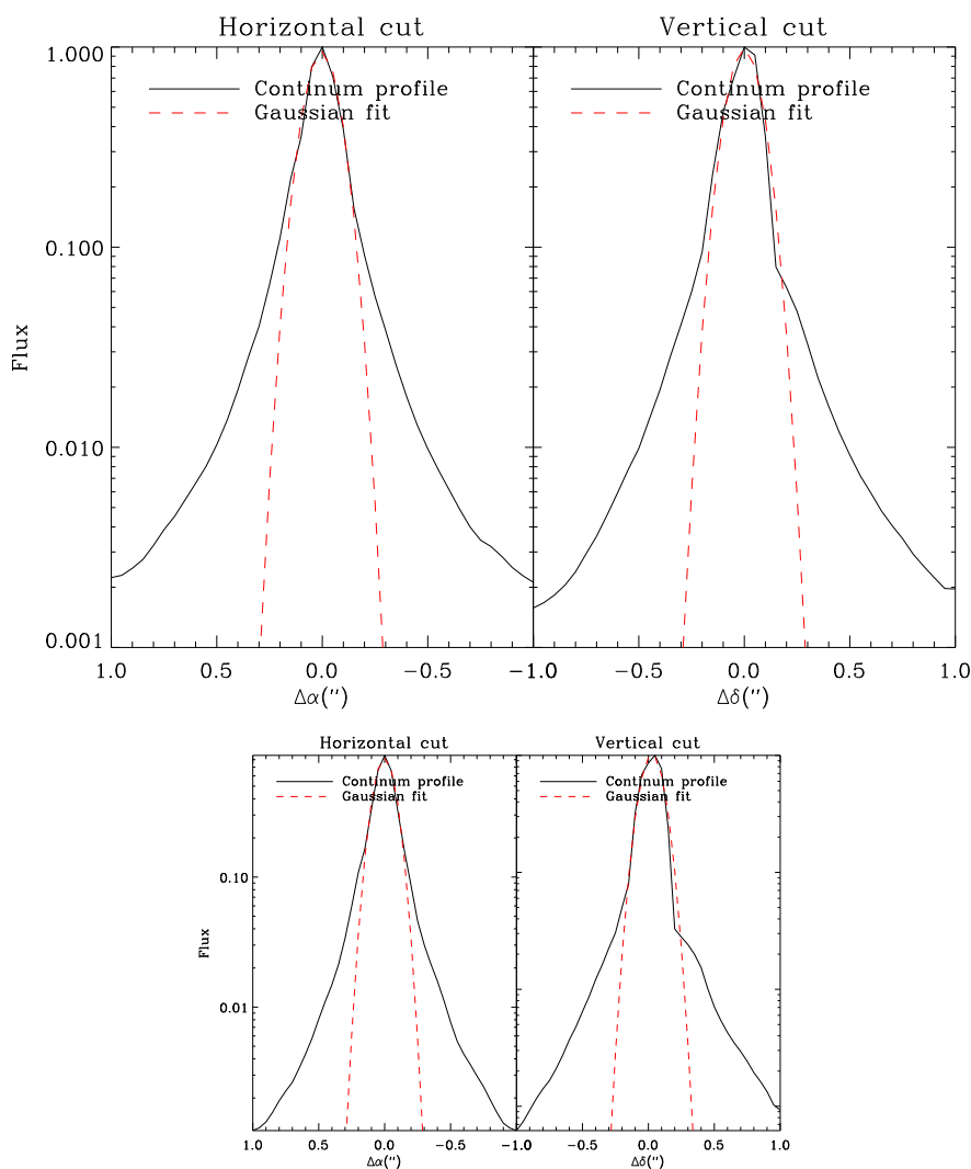
Figure 6.13: Cut, in both spatial directions, of the continuum image used as an estimate of the PSF to deconvolve the [FeII] velocity channel maps. In the \alpha direction the FWHM=0.18'' and FWHM=0.15'' in the \delta direction.
