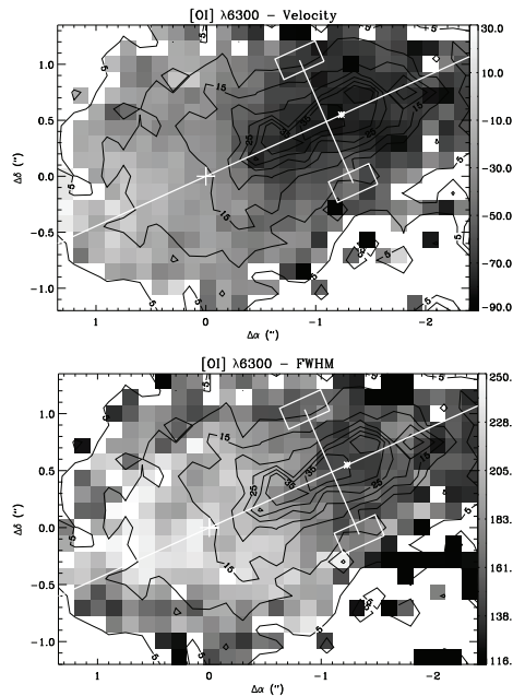
Fig. 5. Maps of the centroid radial velocity ( top ) and velocity width ( bottom ) of a one-component Gaussian fit to the [O I] \lambda 6300 Å line profiles. Contours show the signal to noise ratio (SNR) at the line peak (from 5 to 35 by step of 5). Only lenslets with SNR > 5 are shown. The cross shows the continuum position, the asterisk denotes the HVB knot, and the straight line the blue jet PA. The two white boxes indicate the two regions that contribute to the transverse velocity shift detected at 1''2 from the star and 0''6 to the jet axis in Fig. 8.
