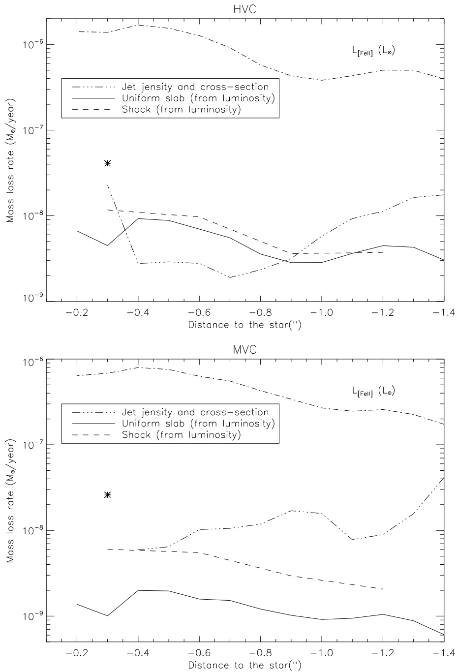
Figure 6.32: Mass-loss rate for the atomic jet in [\text{FeII}]\lambda 1.64\mu\text{m} for the three methods described in the text as indicating in the legend and for the two velocity components identified, HVC on the top and MVC on the bottom. The line luminosity for each velocity component, used in the two methods based in the luminosity, is also represented. Stars indicate the value found by Coffey et al. (2008) for optical observations.
