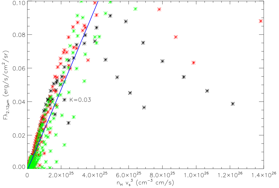
Figure 3.12: Computed H_2 brightness in the 1-0 S(1) ( \lambda = 2.12\mu m ) line against the product n_H V_s^3 to find the factor K in Eq. 3.47 as a linear fit. Different colors refers to models with different magnetic field, b=B/\sqrt{n_H}=0.5 (black), 1.0 (red) and 2.0 (green). In blue we plot the linear fit that gives us a value of K=0.03 .
