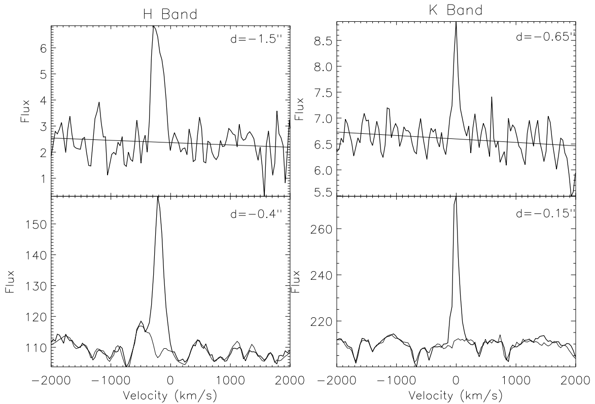
Figure 6.11: Observed spectra in the [\text{FeI}]\lambda 1.64\mu\text{m} line in H band and in the \text{H}_2\lambda 2.12\mu\text{m} line in K band (thick lines) and fitted continuum (thin lines) at two positions along the blueshifted jet. In the H band we used a reference spectrum for distances to the star lower than 1.5'' and a linear fit in the rest. In the K band the limit was fixed at a distance of 0.5'' from the star (see text for more details).
