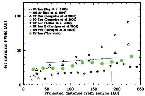
Fig. 4. Large filled circles: PSF-corrected width ( FWHM ) of the RY Tau jet forbidden line emission versus projected distance from the star, as derived from the [O I] HVB deconvolved map (see text). Measurements available on the same spatial scales for other TTS microjets are also plotted with various symbols, after correction for the corresponding PSF. The object-symbol correspondance and references are given at the top left corner of the plot. The position of the knot located at 1''.35 = 190 \text{ AU} in the RY Tau microjet is denoted by the vertical line.
