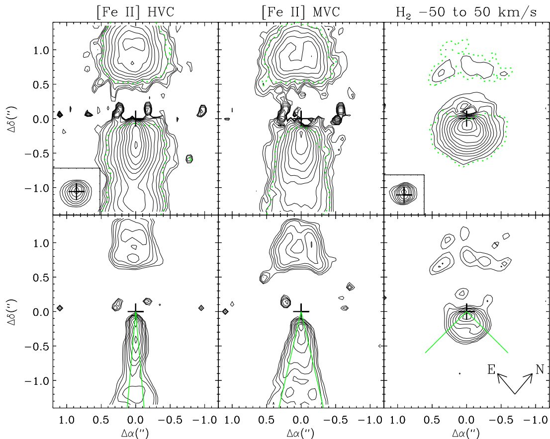
Figure 6.12: Continuum-subtracted maps for [\text{Fe II}]\lambda 1.64\mu\text{m} and \text{H}_2\lambda 2.12\mu\text{m} lines. Atomic emission is centered on -233 km/s for the blue side of the HVC map and on +186 km/s for the red side of the same component, on -111 km/s for the blue MVC and on 29 km/s for the red part. The molecular emission is centered on -0.61 km/s. The cross gives the centroid position of the continuum emission and the dotted contour limits the region with \text{SNR}=5 . Top panels are the raw data and bottom panels shows the same channel maps deconvolved. The opening angles for each blue velocity component are also represented. The notation \Delta\alpha and \Delta\delta are used to mark the spatial coordinates (X,Y) on the detector, the real orientation is given in the last panel. I keep this notation in the following figures. Inserts, in the HVC and \text{H}_2 maps, show continuum images derived from local fits.
