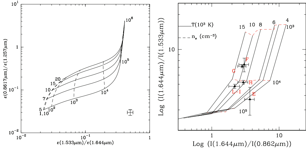
Figure 3.7: Diagnostic diagrams from Pesenti et al. (2003) on the left and Nisini et al. (2005) on the right from [FeII] lines in the IR domain. Left: dashed lines show n_e varying from 1 to 10^6 \text{cm}^{-3} in factors of 10, solid lines show T_e varying from 5000 to 20 000 K. Right: dashed lines show electron densities of 10^3 , 10^4 and 10^5 \text{cm}^{-3} and solid lines show electron temperatures of 4, 5, 6, 8, 10, 15 \times 10^3 K.
