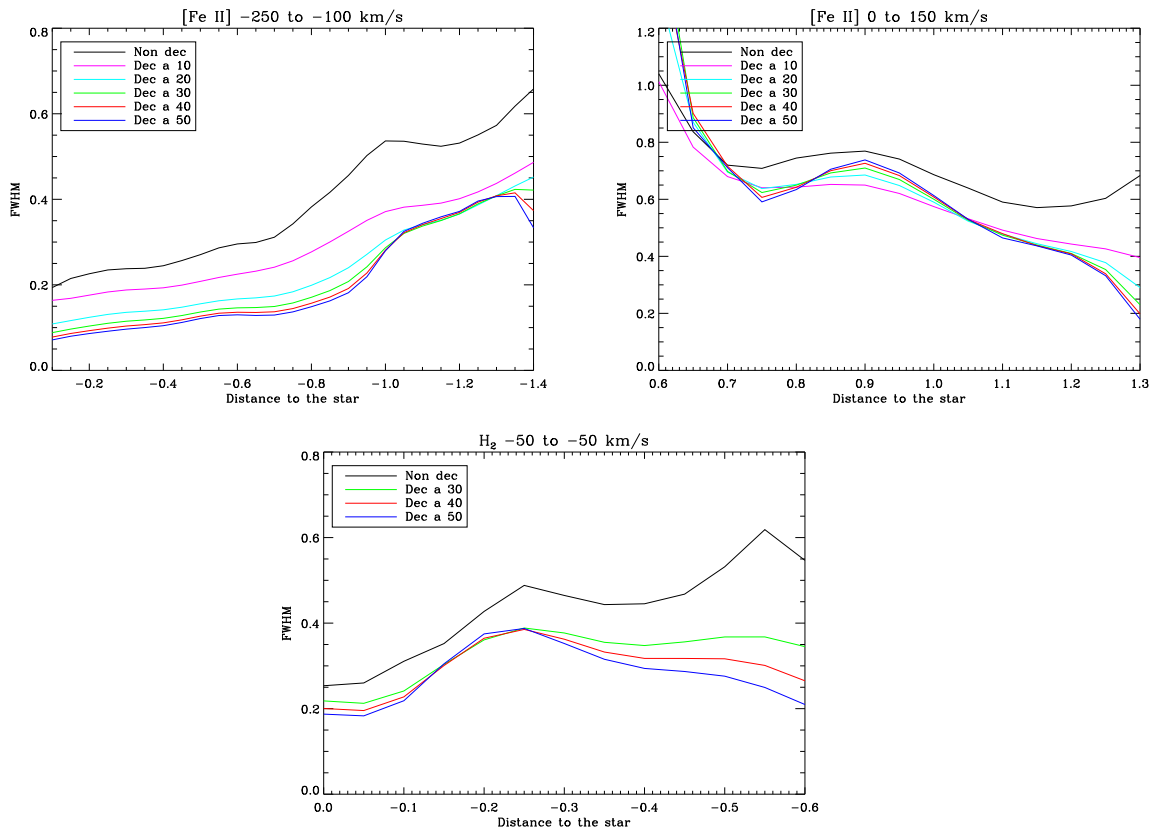
Figure 4.9: Deconvolved DG Tau jet widths measurements as a function of the distance to the star for different number of interactions. The original maps are that shows in top panels of Fig. 6.12 in Ch. 6. The final number of iterations taken to obtain the restored images shown in bottom panels of Fig. 6.12 is 40. The two top graphics correspond to the atomic jet (blue side in the left and red side on the right). The bottom graphics corresponds to the molecular emission.
