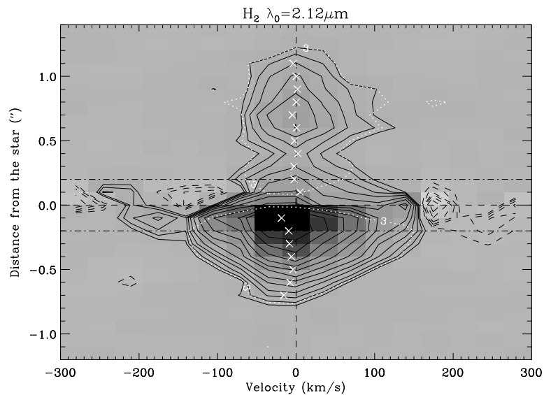
Figure 6.22: Position-velocity map for the H_2 \lambda 2.12 \mu\text{m} line for a pseudo-slit of 1'' width and sampling every 0.1'' . Contours start at 1.72 \times 10^{-15} \text{ W m}^{-2} \mu\text{m}^{-1} (")^{-2} and increase by factors of \sqrt{2} . White contours and crosses are the same as in Fig. 6.21.
