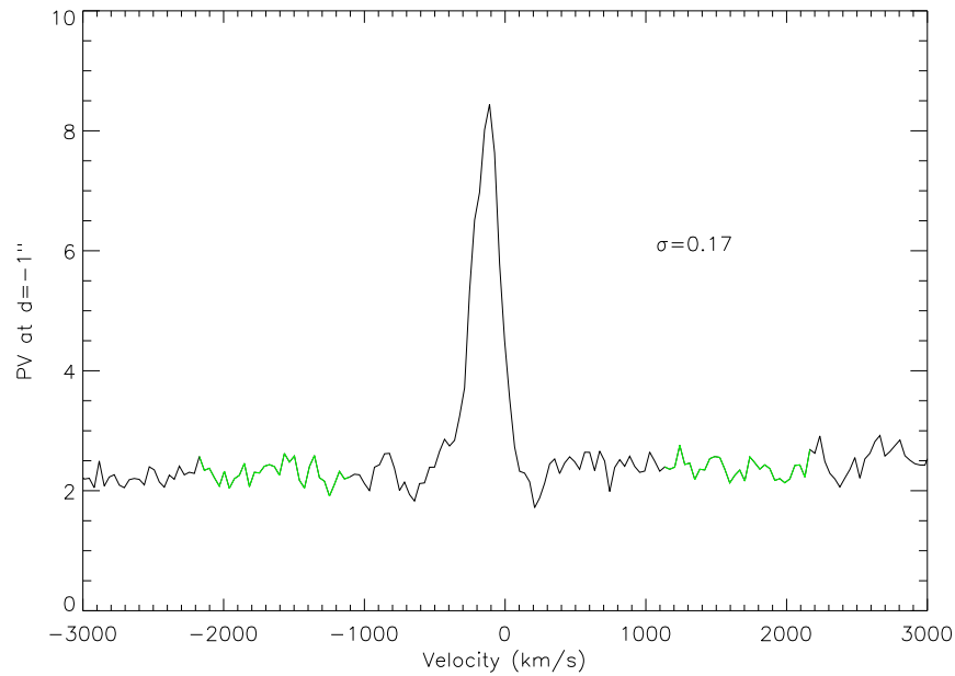
Figure 4.11: Example of the noise estimation in a spectrum of the PV diagram of DG Tau in the blue side of the jet, at a distance of 1'' from the star. The intervals in green are the regions where the standard deviation was computed.
