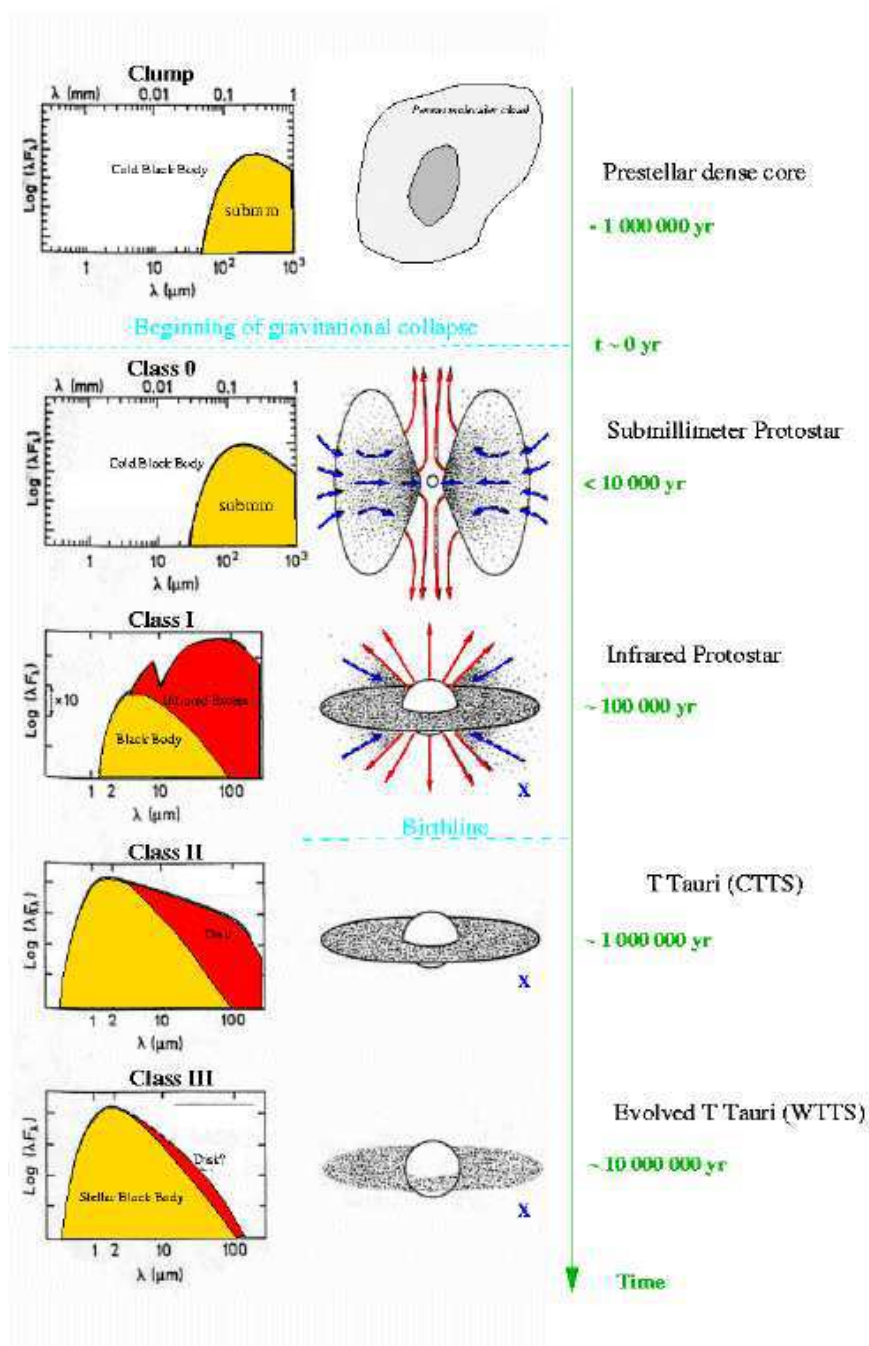
Figure 2.1: Classification of low mass young stellar objects and schema of their evolution.
