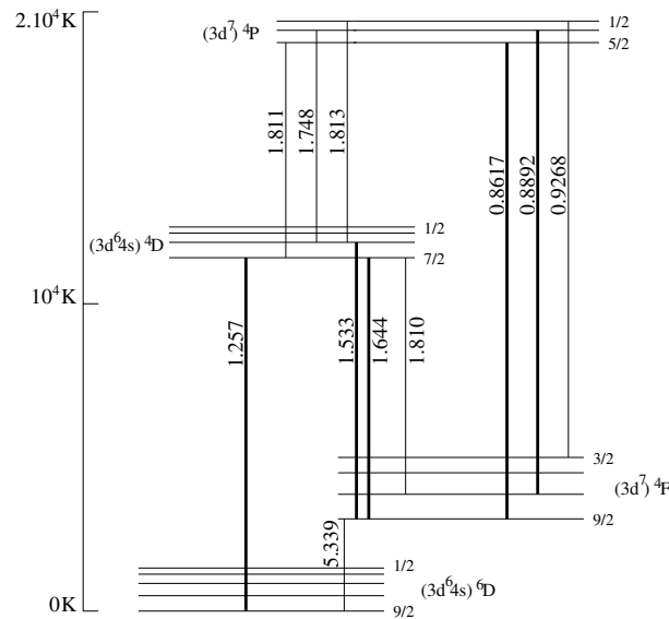
Figure 3.4: Energy level diagram of the more prominent optical and near-infrared [Fe II] emission lines (wavelengths in \mu\text{m} ) originating from the 16 first levels, adapted from Pesenti et al. (2003).
