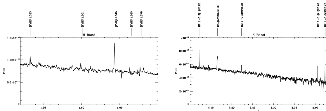
Figure 6.1: Average spectra, both in the H and K band, from a region with strong emission from the DG Tau jet. I label the strongest emission lines identified, most of them iron and molecular hydrogen lines, but also the \text{Br}_\gamma line at 2.16 \mu\text{m} .
