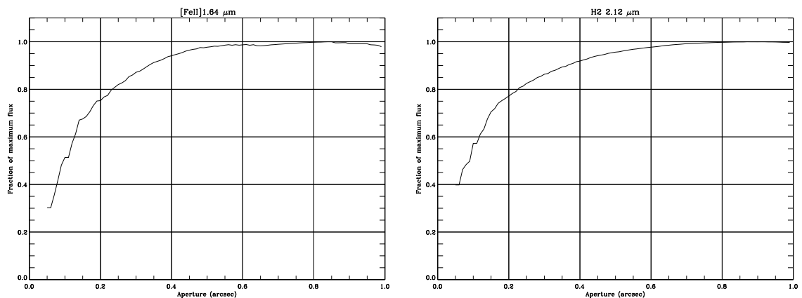
Figure 6.9: Measured flux normalized to the maximum in the telluric standards as a function of the aperture taken for integrating the flux. The H band on the left and the K band on the right.
