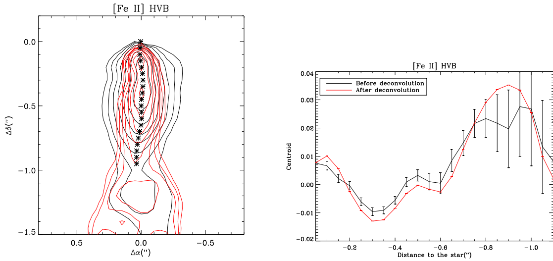
Figure 6.17: Left: HVB channel map, before deconvolution in black and after deconvolution in red. Stars mark the centroid position derived from a Gaussian fit to the transverse profiles. Right: The centroid positions in arcseconds as a function of the distance to the star, marked as stars in the left panel.
