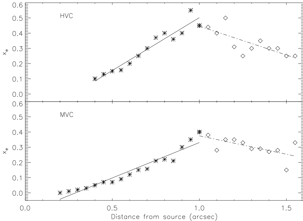
Figure 6.30: Derived ionization fraction values for different distances from the star and for the high and medium velocity components, from Bacciotti (2002). We carried out two linear fits for distances lower and higher than 1'' separately.
