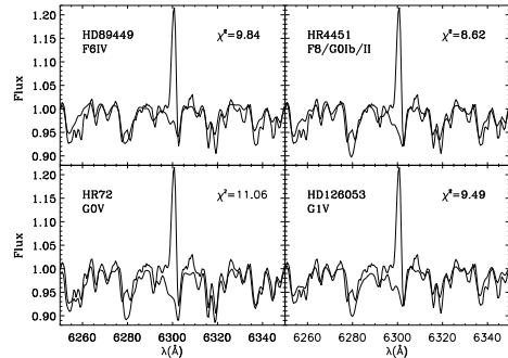
Fig. 1. Comparison between the EXPORT RY Tau spectrum (thick line, from Mora et al. 2001) and rotationally broadened EXPORT spectra of four reference stars (thin lines). The reduced \chi^2 , computed over our 6210–6550 Å wavelength domain (excluding the [O I] line region) is indicated in each panel. The reference star that best fits the photospheric spectrum of RY Tau is HR 4451.
