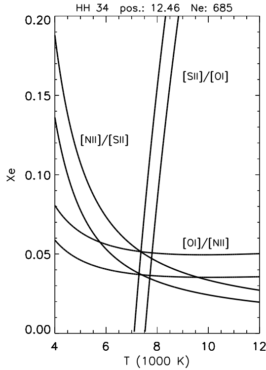
Figure 3.9: Example of the BE technique to derive the electron temperature and the ionization fraction in the jet of the HH 34 object. The values of x_e and T , and their uncertainty, are found from the intersections of the curves. Adapted Bacciotti & Eisloffel (1999).
