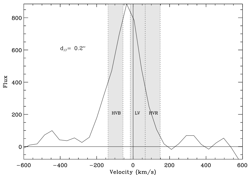
Figure 4.10: For a given emission line, one can choose the velocity intervals where the emission will be integrated to reconstruct each channel map. This is the example of the three velocity components (three channel maps) observed for the RY Tau jet (Ch. 5).
