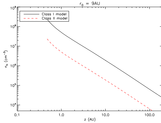
Figure 6.43: Predicted n_H as a function of z for the solution with \lambda = 13 and r_0 = 9 \text{ AU} (Casse & Ferreira, 2000). The class I model corresponds to a mass accretion rate of 10^{-6} M_{\odot}/\text{yr} and the class II model corresponds to 10^{-7} M_{\odot}/\text{yr} .
