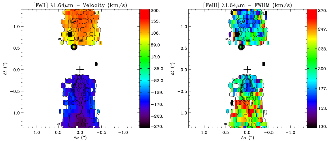
Figure 6.18: Maps of the centroid radial velocity (left) and velocity width (right) resulting of a one-component Gaussian fit to the [FeII] \lambda 1.64\mu\text{m} line on each individual spectra. Contours give SNR at the line peak from 5 to 65 by step of 10. Only the spectra with SNR higher than 5 are shown. The cross marks the position of the star.
