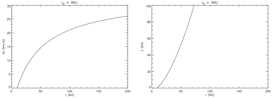
Figure 6.41: Left: Velocity predicted by models by Casse & Ferreira (2000) as a function of the disc radius for the streamline at r_0 = 9 AU. For distances of \sim 50 AU, the predicted velocity is \sim 15 km/s, as observed, and the terminal velocity is reached at higher distances. Right: For the same solution, the morphology of the streamline is in good accord with the observed morphology.
