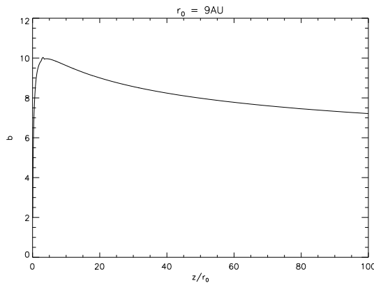
Figure 6.42: Predicted b = B / \sqrt{n_H} as a function of z/r_0 for the solution with \lambda = 13 and r_0 = 9 AU (Casse & Ferreira, 2000).
