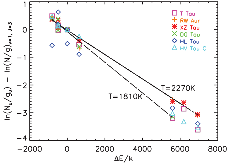
Figure 3.8: Example of a Boltzmann diagram obtained from different H_2 transitions, for several T Tauri stars, from Beck et al. (2008).
