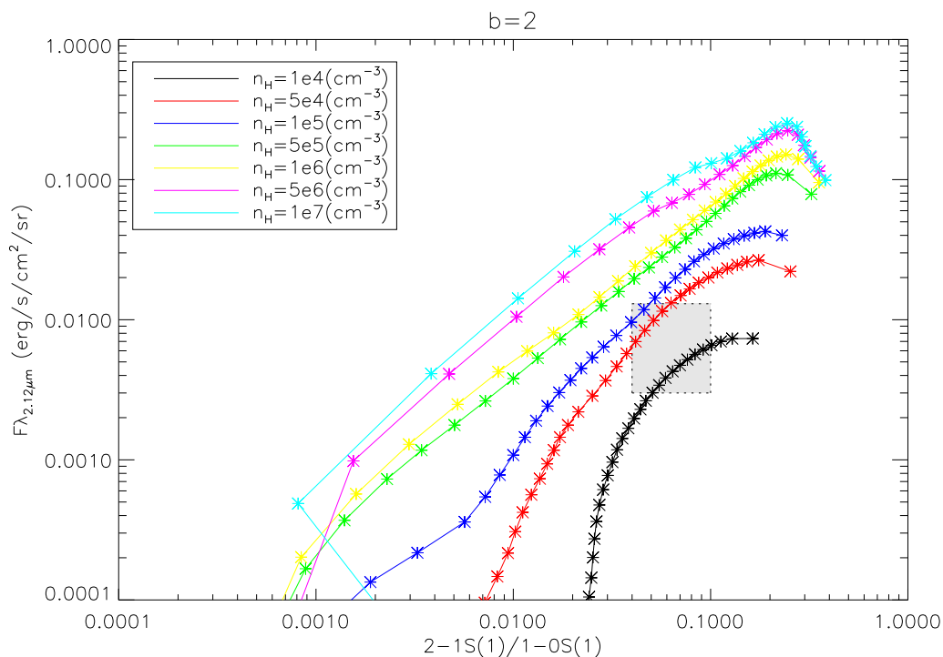
Figure 6.37: Same as Fig. 6.35 but for a C-shock with b=2.0 .
