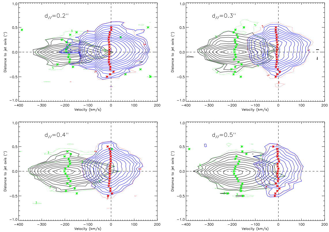
Figure 6.23: Transverse position-velocity diagram for distance to the star of 0.2'' , 0.3'' , 0.4'' and 0.5'' . Iron is plotted in black and H_2 in blue. Centroids velocities from an one-component Gaussian fit are also plotted as green asterisks for the [Fe II] and in red for the molecular emission. The dotted-line contours mark the SNR=3 limit. Emission up to \pm 100 km/s in H_2 are artefacts of spectral PSF of SINFONI.
