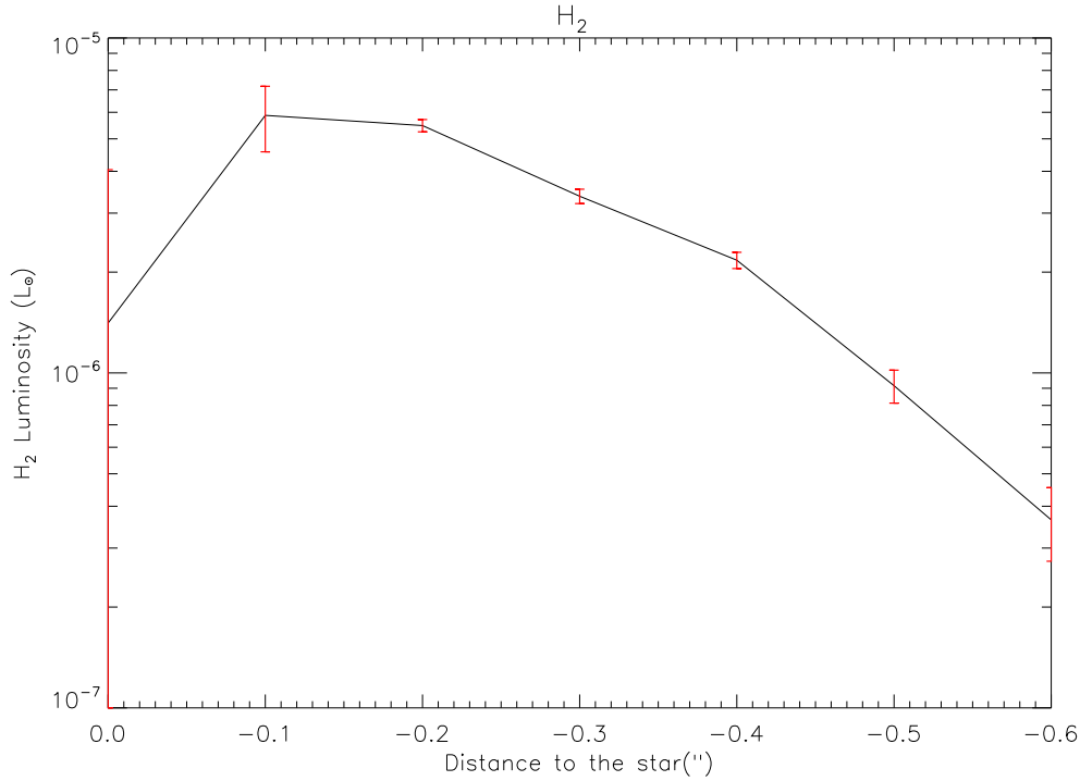
Figure 6.27: H_2 luminosity integrated over a pseudo-slit width of 1'' and sampled every 0.1'' , plotted errors are at 3\sigma . A peak is observed at 0.1'' from the star and then it decreases with distance. The mass of H_2 (Eq. 3.45) and the mass-loss rate, in the case of volume emission, are proportional to the line luminosity.
