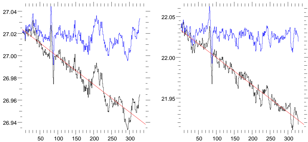
Figure 4.6: Example of the ADR effect from OASIS data (in the X direction of the detector on the left and in the Y direction on the right). The measured displacement as a function of the wavelength are plotted in black. In blue we show the same centroid displacement once the ADR effect has been corrected. The red line is the linear fit used to correct from this effect.
