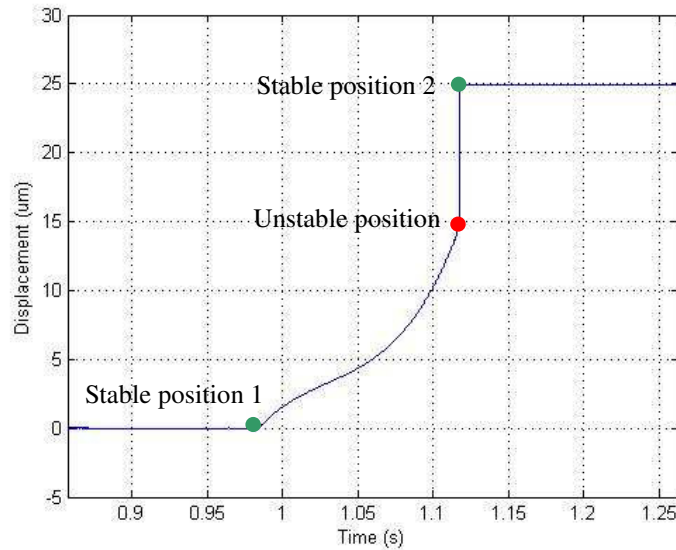
Fig. 5.14. Details of the transition to stable position 2.
