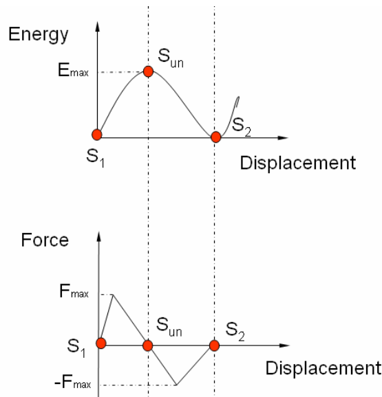
Fig. 3.1. Switching mechanical characteristics.
