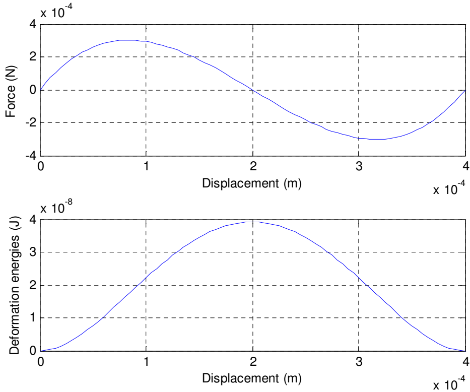
Fig. 3.13. Force –displacement and energy –displacement relations of case 2.
