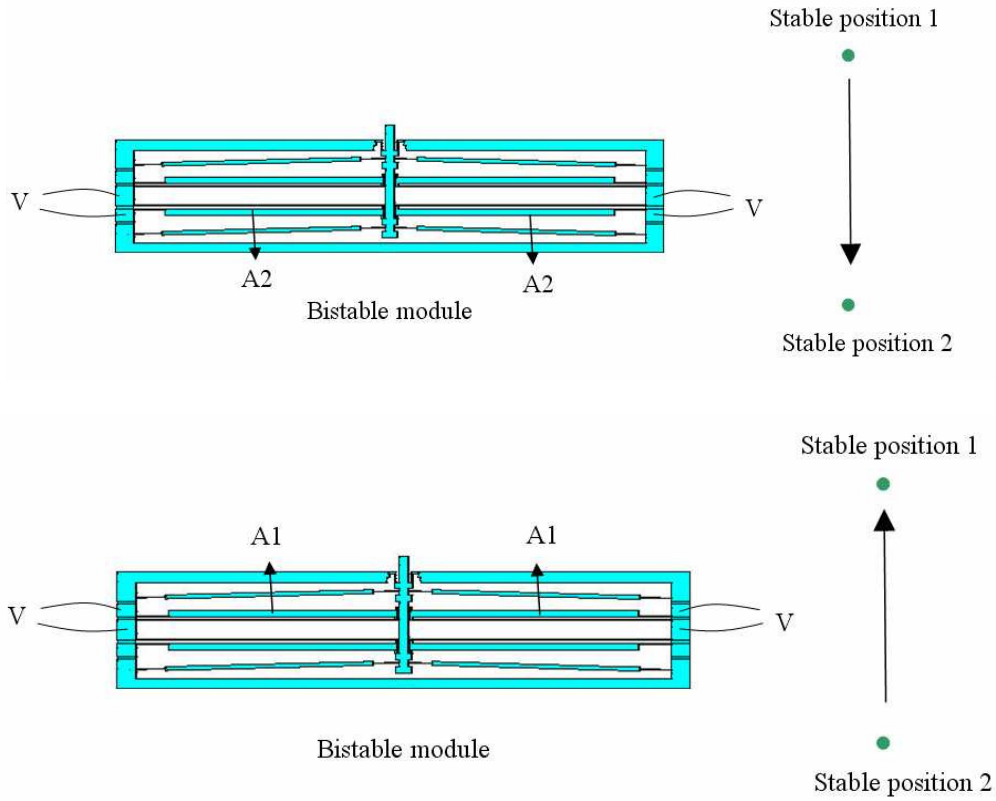
Fig. 3.42. Two pairs of thermal actuators for two stable positions.
