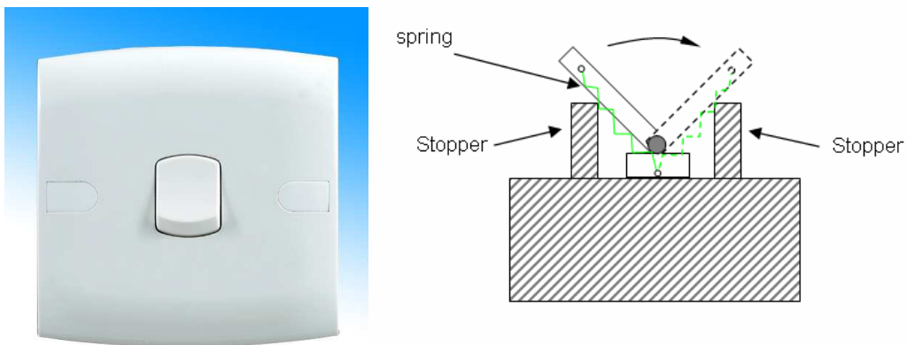
Fig. 2.11. (a) A light switch (b) typical schematic of the light switch.
