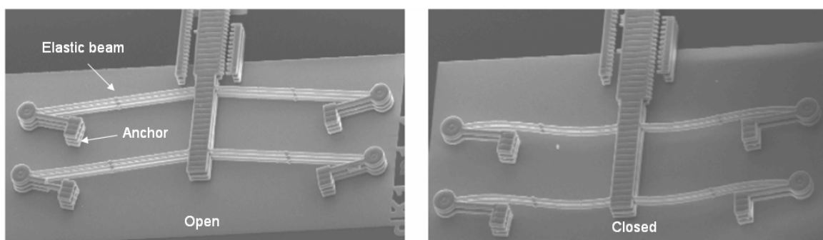
Fig. 2.13. Bistable mechanism in up and down positions [WIL 04].
