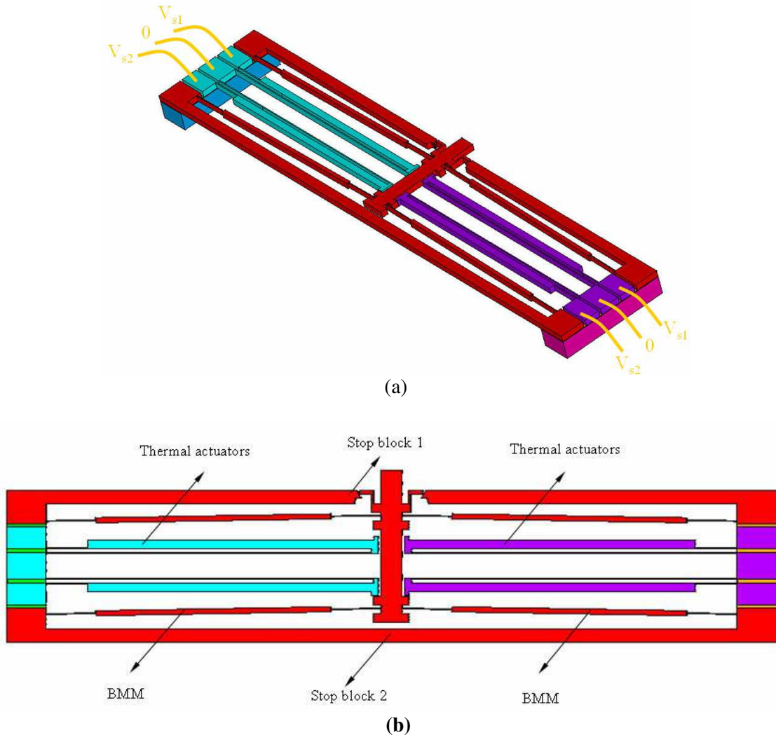
Fig. 4.13. (a) 3D view of the bistable module. (b) plane of the bistable module.
