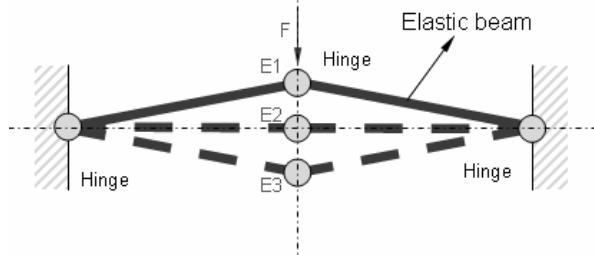
Fig. 3.21. The elastic beam is compressed from first stable position to second stable position.
