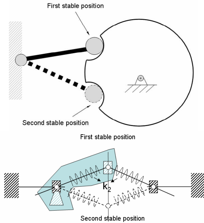
Fig. 3.4. Equivalent model of the cam mechanism.
