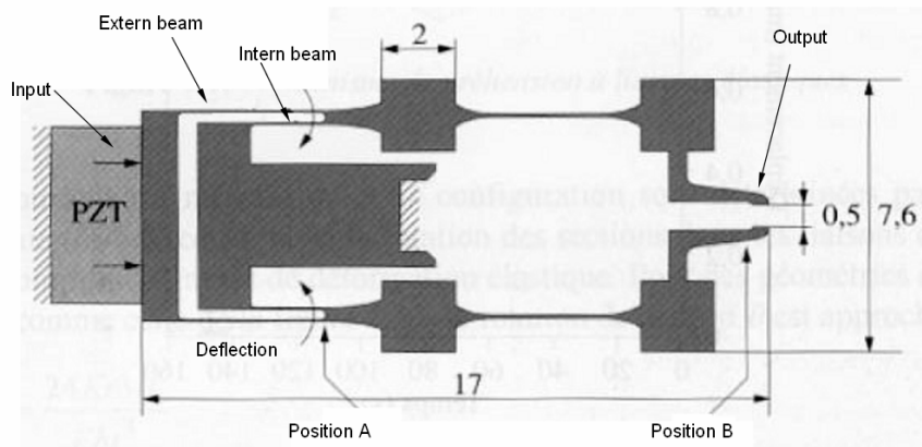
Fig. 1.14. Example of bimorph principle [CAR 98].
