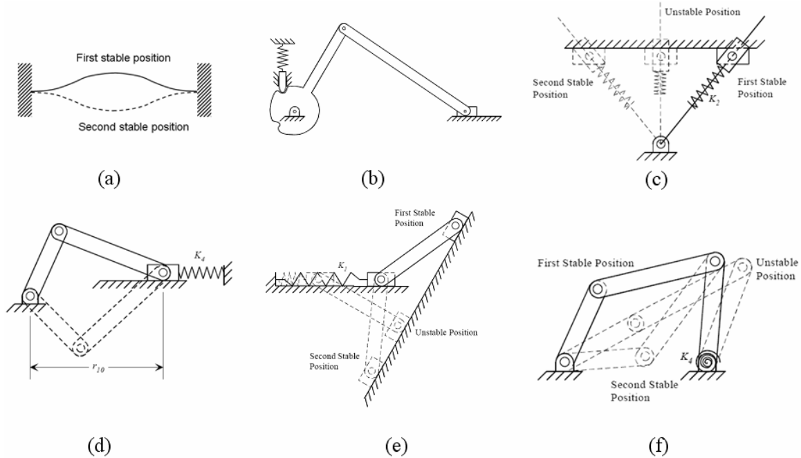
Fig. 3.1. (a) Snap-through buckled beams (b) Bistable cam mechanisms (c) Double-slider mechanisms with a pin joining the sliders (d) Double-slider mechanisms with a link joining the sliders (e) Slider-crank or slider-rocker mechanisms (f) Four-link mechanisms [JEN 98].
