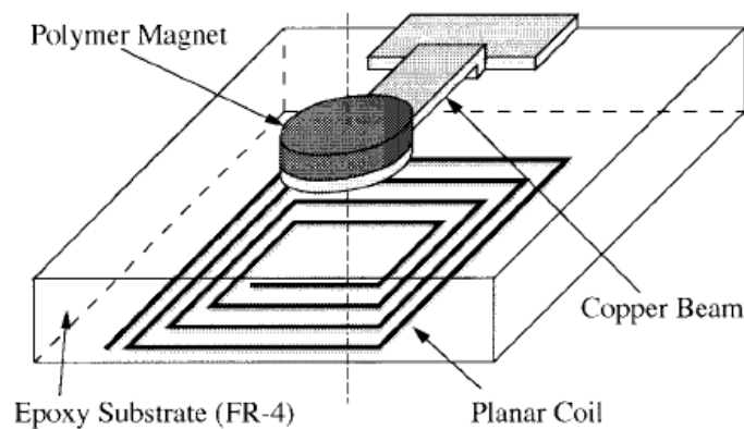
Fig. 1.22. Electromagnetic microactuators based on polymer magnets [LAG 99].
