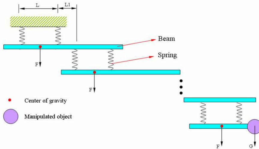
Fig. 3.47. Model of n cascaded bistable modules.
