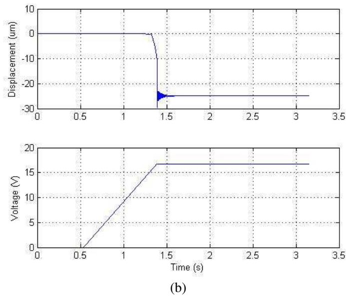
Fig. 5.15. Response from position 2 to position 1.
