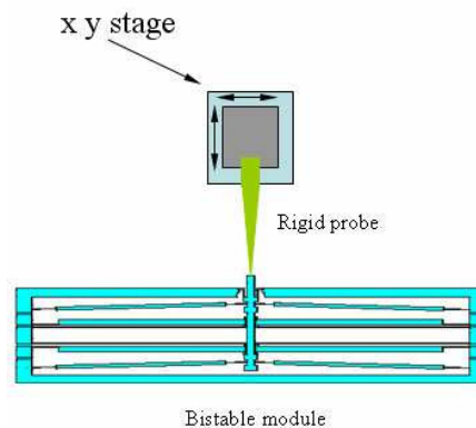
Fig. 5.2. Activation of bistable module using a probe.
