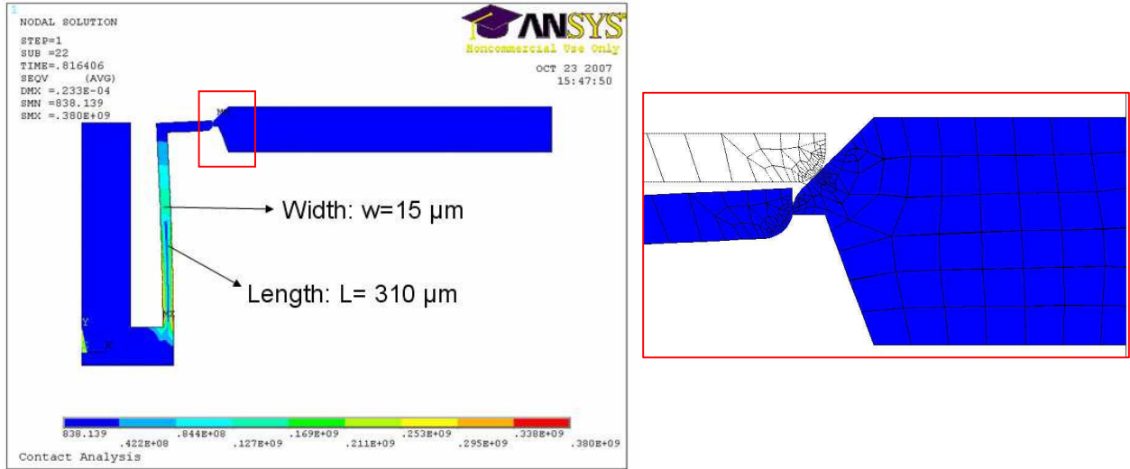
Fig. 3.37. The activation simulation of the stop block.
