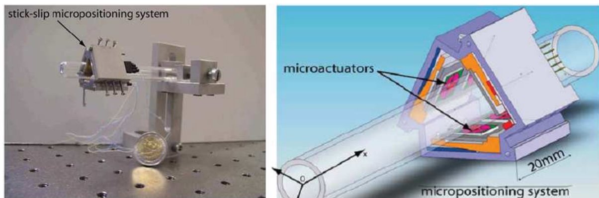
Fig. 1.37. The fabricated stick-slip motor with 2DOFs [RAK 09a].
