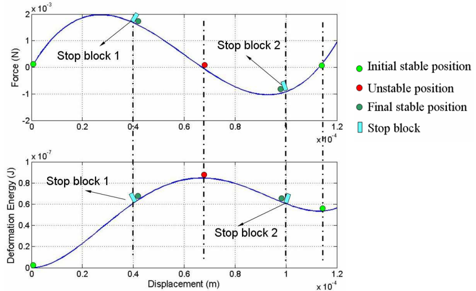
Fig. 3.39. The location of the two stop blocks.
