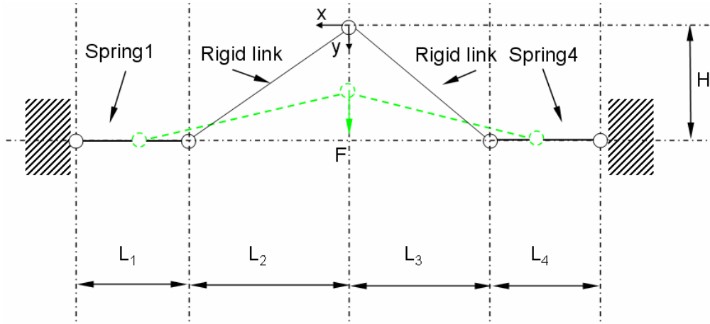
Fig. 3.12. Schematic of bistable mechanism of case 2.
