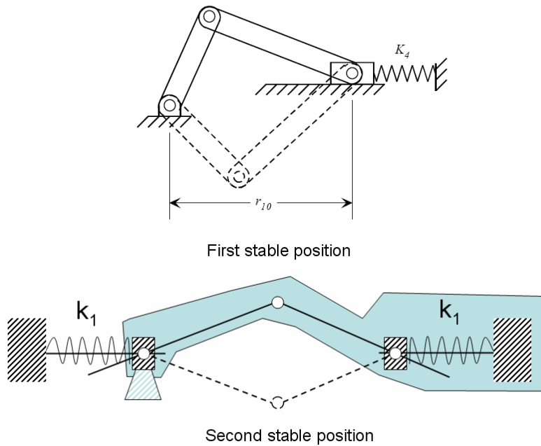
Fig. 3.6. Slider-crank or slider-rocker mechanisms.
