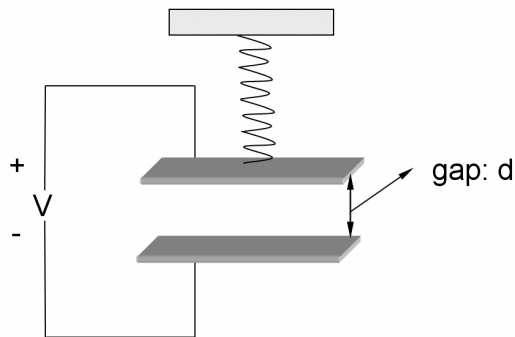
Fig. 1.24. Parallel plate electrostatic actuator.
