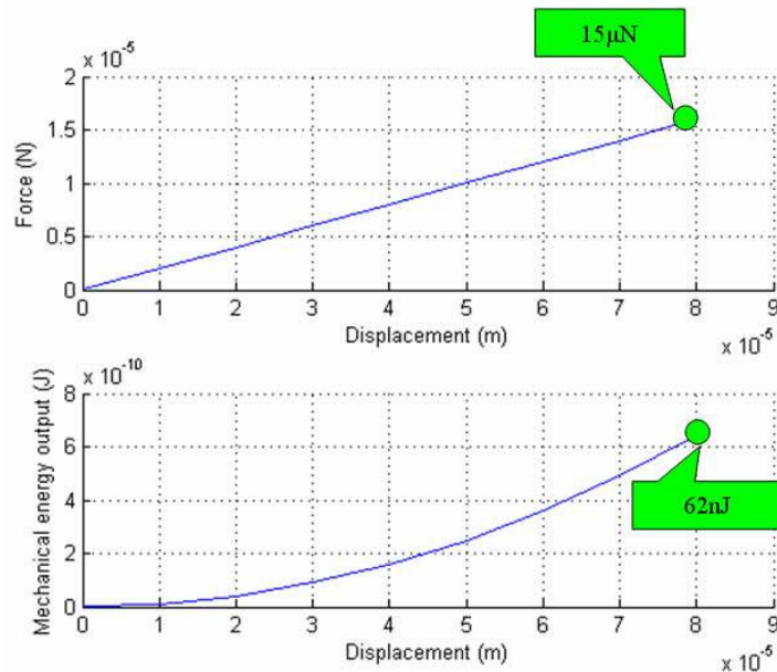
Fig. 4.16. Force and mechanical energy output of thermal actuator.
