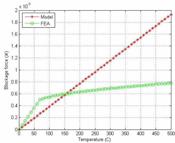
Fig. 3.33. Temperature-blockage force comparison between model and FEA.
