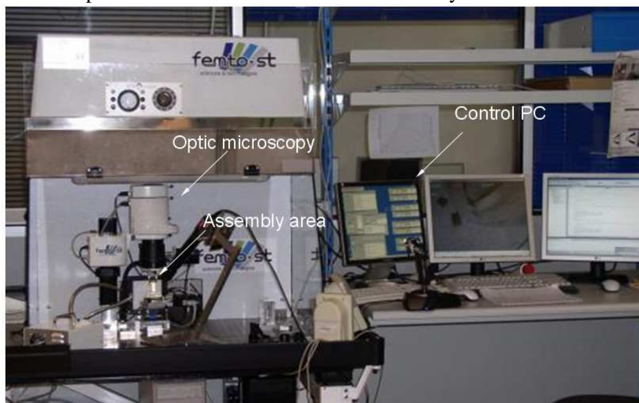
Fig. 1.6. Microassembly station at Femto-st/As2m.
