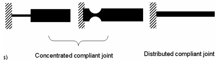
Fig. 3.19. Examples of compliant joints.
