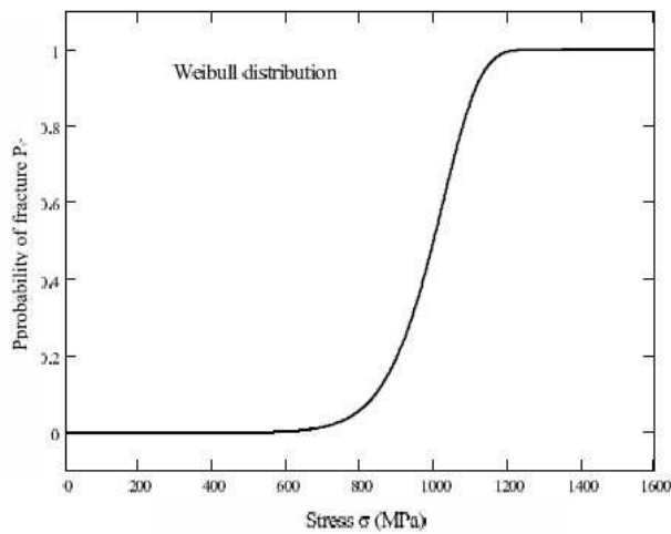
Fig. 4.11. Weibull distribution of the probability of fracture versus stress [WEI].
