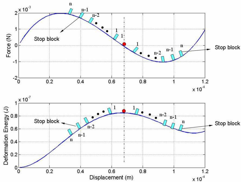
Fig. 3.44. Locations of the stop blocks in the cascaded bistable modules.
