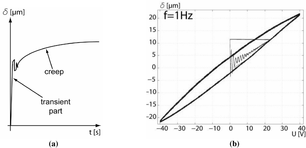
Fig. 1.32. (a) A creep phenomena of piezoelectric bimorph beam [RAK 09a]. (b) Hysteresis of a piezoelectric bimorph beam [RAK 09a].
