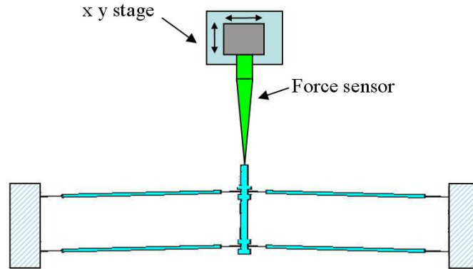
Fig. 5.4. Experimental set-up (a commercial force sensing probe (ST-S270 from FEMTO TOOLS [FEM] with a sensitivity of 899.2 \mu\text{N/V} ).
