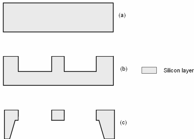
Fig. 4.7. A typical bulk machining.
