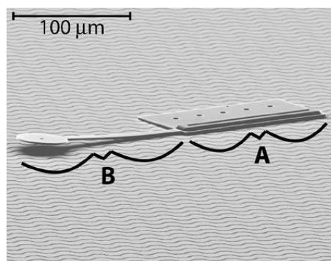
Fig. 1.2. A mobile microrobot. A: scratch drive actuator, B: cantilevered steering arm (B) [DON 06].
