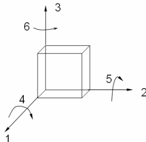
Fig. 1.26. Numbering of the direction for the piezoelectric parameters.
