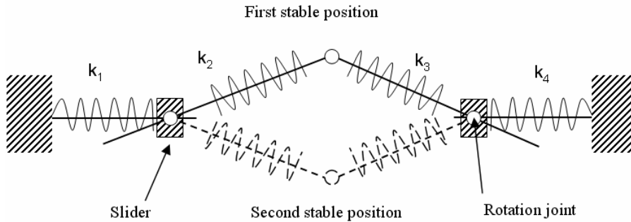
Fig. 3.2. A generic bistable mechanism.
