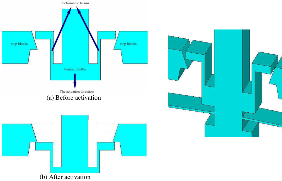
Fig. 3.36. The designed stop block.
