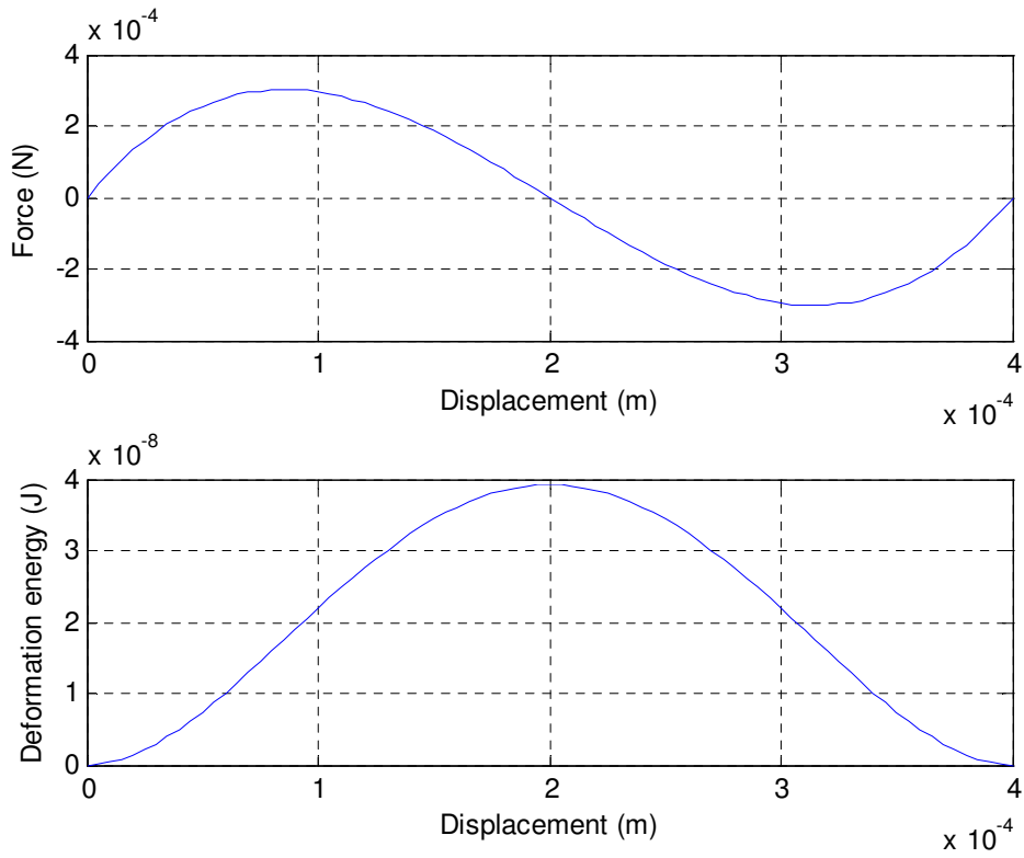
Fig. 3.11. Force –displacement and energy –displacement relations of case 1.
