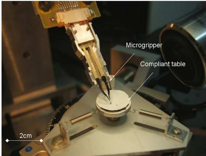
Fig. 1.7. Large view of assembly area.
