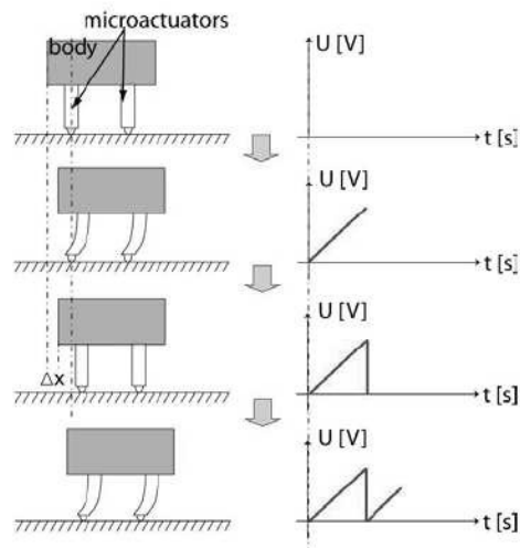
Fig. 1.36. Principle of stick-slip motion [RAK 09a].
