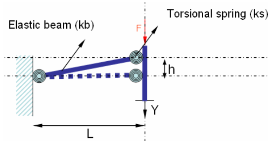
Fig. 3.26. The model of the compressed piezoelectric material.
