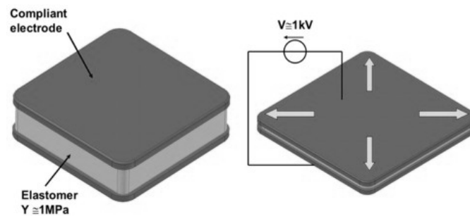
Fig. 1.31 Principle of electroactive polymers [LMTS].
