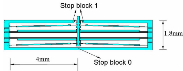
Fig. 4.2. Designed bistable module.
