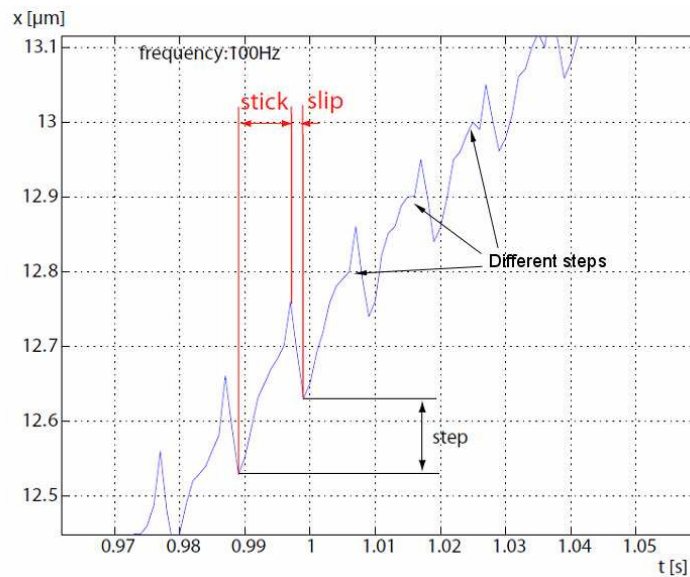
Fig. 1.39. Measurement of steps in linear motion (voltage U = 150V ) [RAK 06b].
