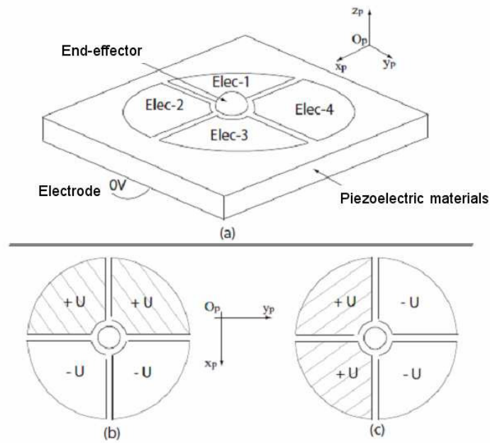
Fig. 1.38. Configuration of 2DOFs piezoelectric actuator, (a) Four used electrodes, (b) motion following O_p x_p , (c) Motion following O_p y_p [RAK 06a].
