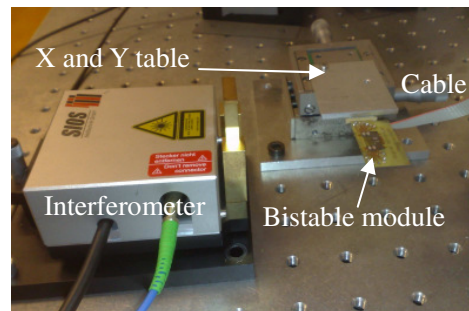
Fig. 5.10. Experimental set-up.
