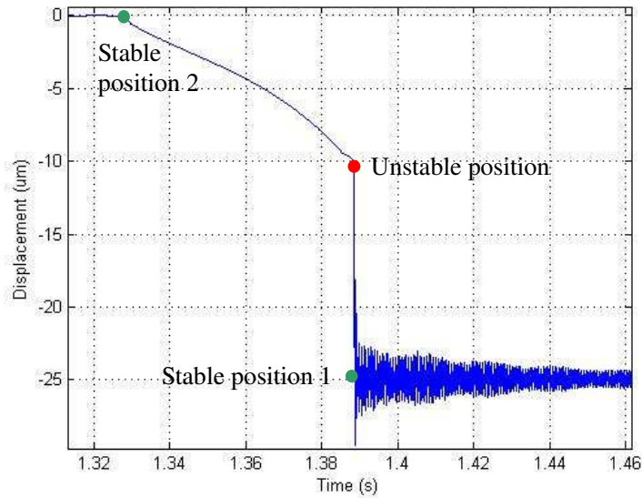
Fig. 5.16. Details of the transition to stable position 1.
