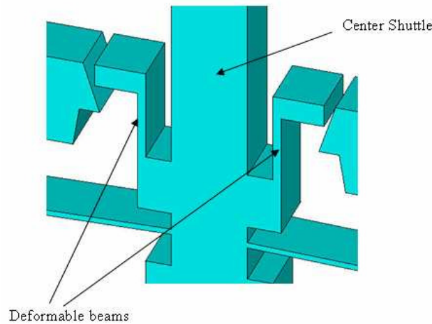
Fig. 5.1. The designed stop block.
