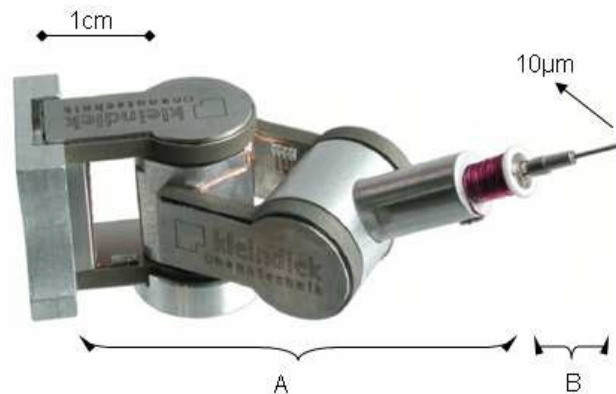
Fig. 1.3. A centimeter robot mounted end-effector. A: Robot mechanism, B: end-effectors [KLE].
