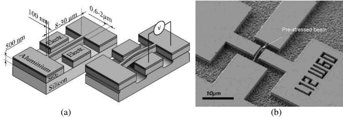
Fig. 2.16. (a) Schematic of a bistable pre-stressed beam (b) photo of the design (using a SEM: Scanning Electron Microscope) [CHA 08].
