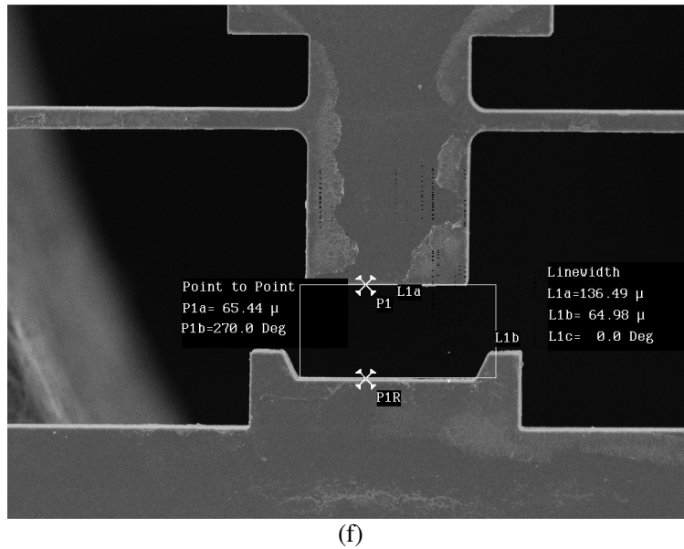
Fig. 4.25. (a,b,c,d) Scanning electron microscope (SEM) pictures of microfabricated module. (e) The width measurement of bistable beam using the SEM picture. (f) Measurement of the distance between the bistable mechanism and the second stop block using the SEM picture.
