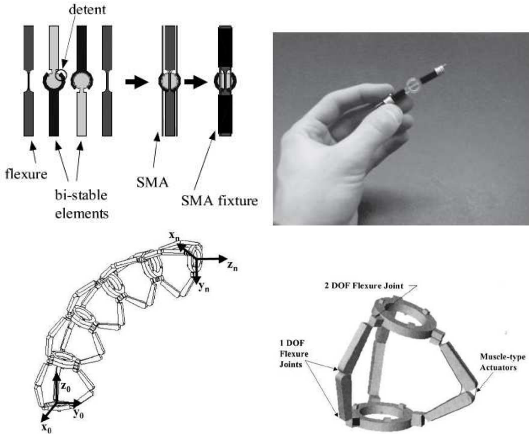
Fig. 2.8. Binary Robotic Articulated Intelligent Device (BRAID) [SUJ 04].
