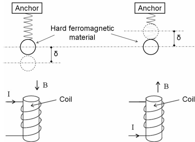
Fig. 1.21. Electromagnetic force.
