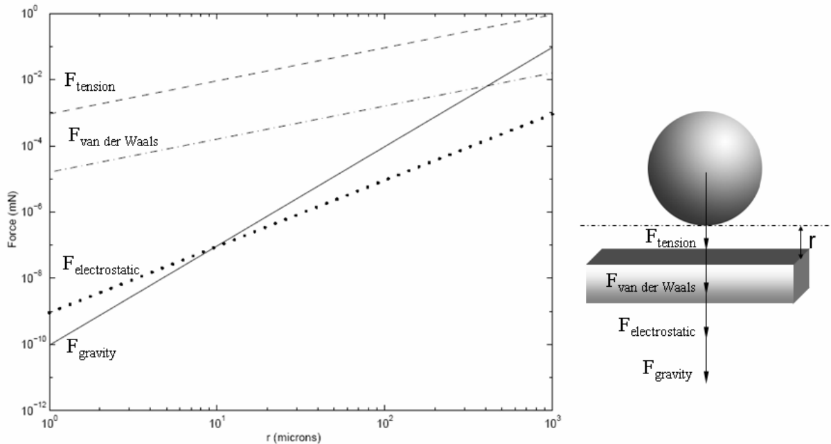
Fig. 1.4. The different forces in the microworld for a sphere/ plane interaction.
