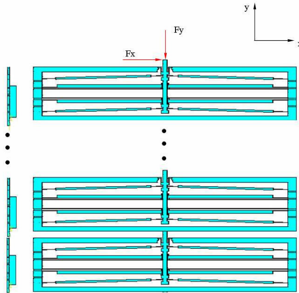
Fig. 3.43. N cascaded bistable modules.
