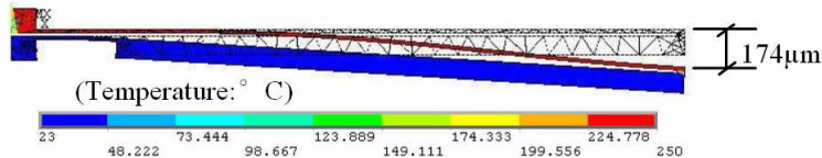
Fig. 3.34. Electro-thermal-mechanical simulation result.
