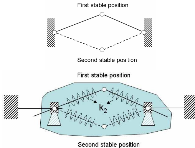
Fig. 3.3. Equivalent model of curved bistable mechanism.
