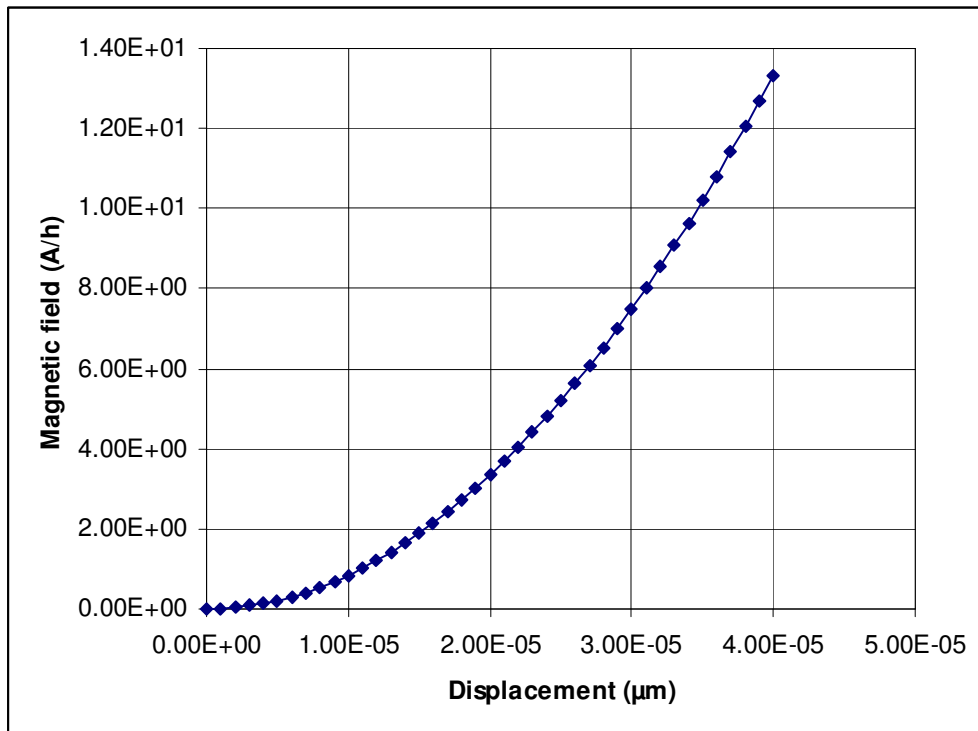
Fig. 3.29. The applied magnetic field Vs the displacement.
