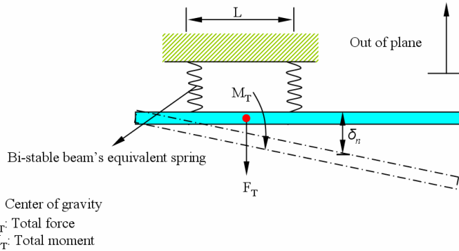
Fig. 3.46. The equivalent out-of plane model of a bistable module.
