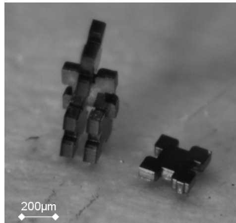
Fig. 1.1. Assembled microobjects [TAM 09].
