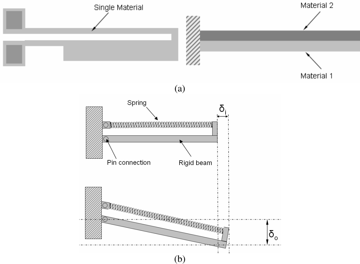
Fig. 1.13. (a) classic bimorph mechanism (b) a model of a bimorph mechanism.
