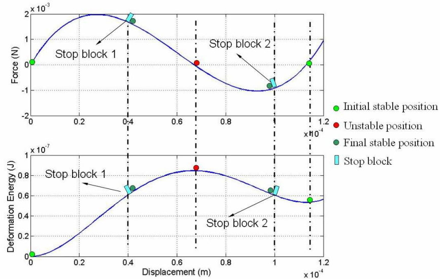
Fig. 5.12. Locations of the stop block.
