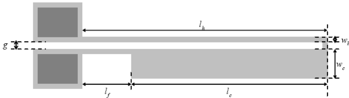
Fig. 4.14. Dimensions of thermal actuator [MUR 05].
