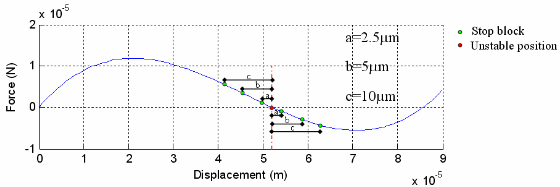
Fig. 5.6. Three locations of the stop blocks.
