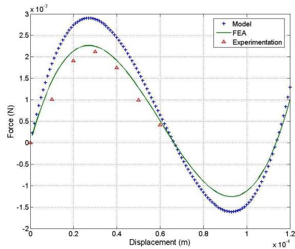
Fig. 5.5. Force (F) Versus displacement (Y) characteristic.
