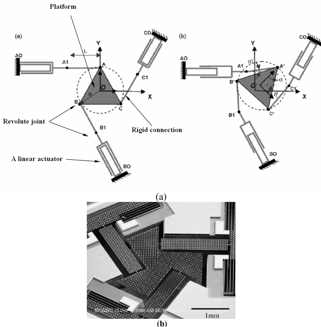
Fig. 1.18. (a) Schematic of a xy\theta positioner (b) Fabricated positioner [MUK 08].
