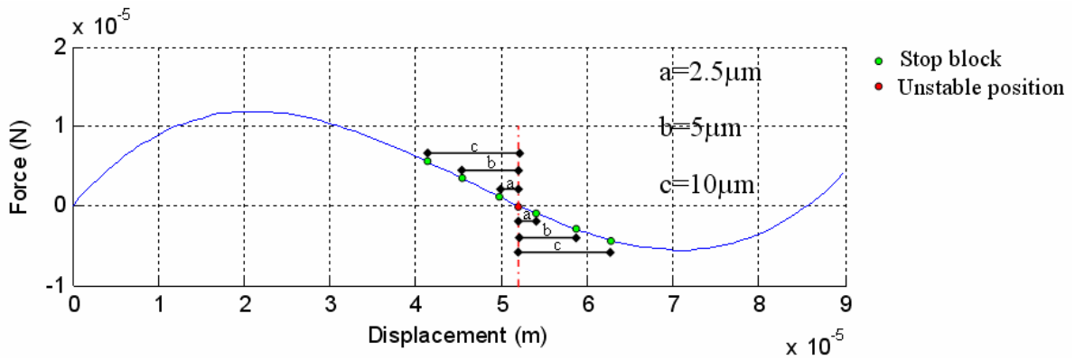
Fig. 3.41. Three locations of the stop blocks.
