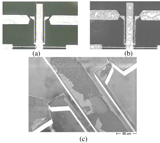
Fig. 5.3. (a) Before activation. (b) After activation. (c) SEM photo of 3D stop block after activation.
