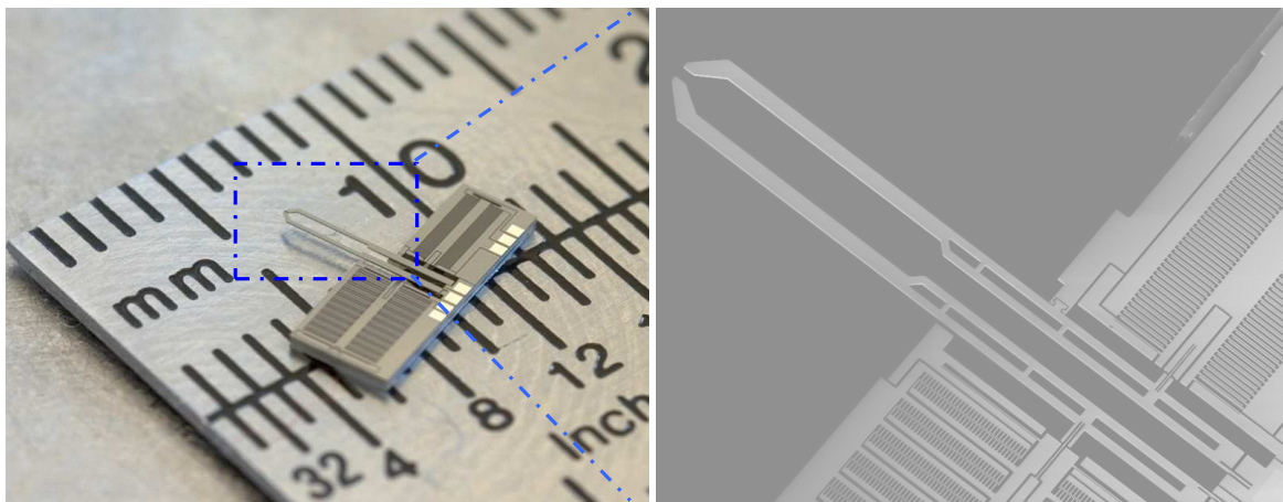
Fig. 4.3. A fabricated microgripper by FEMTO TOOLS [FEM].
