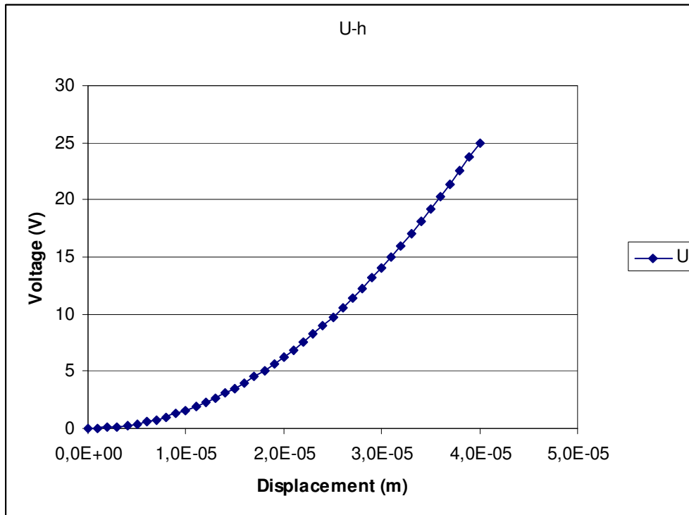
Fig. 3.27. The applied voltage Vs the displacement.
