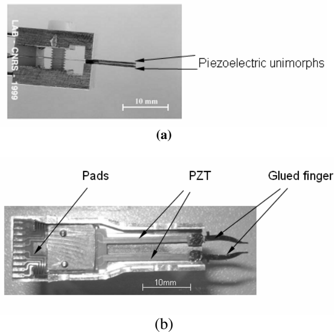
Fig. 1.28 (a) Microgripper including two unimorphs (Y. Haddab of Femto-st institute) [Yas 04](b) Two DOF microgripper (J. Agnes of Femto-st, institute) [AGN 03].
