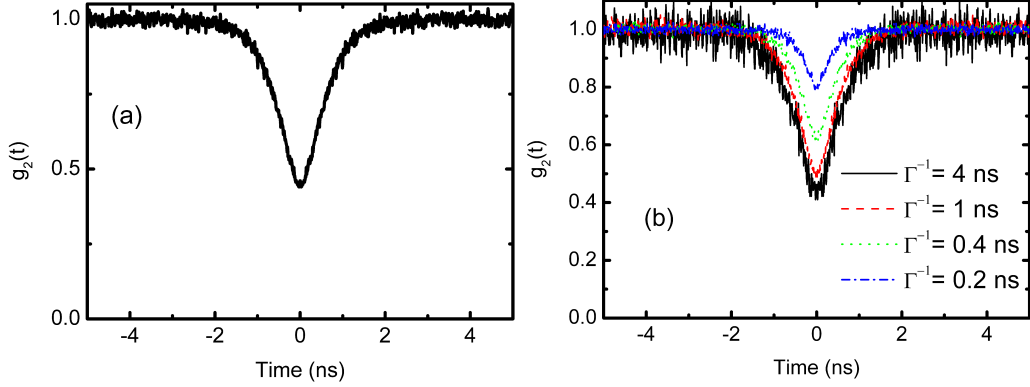
Figure 4.16: (a): simulation of the autocorrelation of the exciton (same parameters than figure 4.13(b)) taking into account a time resolution of 300 ps. (b): effect of the pumping rate on the exciton autocorrelation function.
