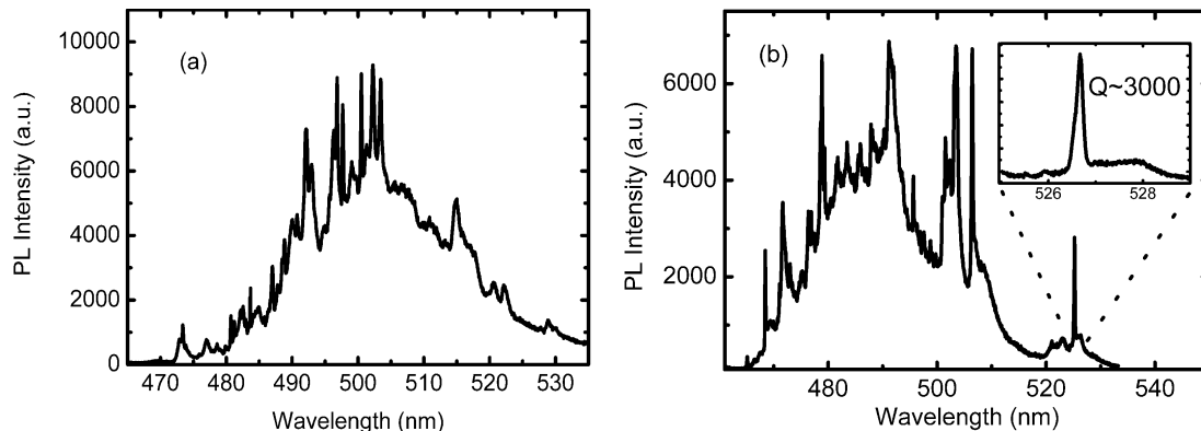
Figure 5.3: (a): Low temperature CW \mu PL on a good 3\mu\text{m} microdisk. Optical modes appear as sharp lines in the spectrum. The linewidths are down to 0.1 nm. (b): Best quality factor at low energy (525 nm) that we could measure. It reaches 3000.
