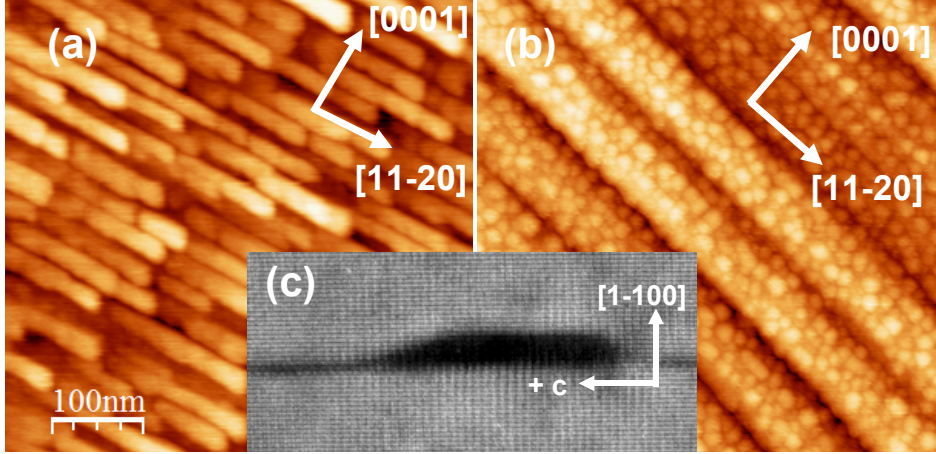
Figure 2.1: Illustration of the wires (a) and dots (b) geometry (AFM image: B. Amstatt). The structures are aligned along the [11\bar{2}0] direction. The inset (c) shows a TEM image (C. Bougerol) of a quantum dot viewed along the [11\bar{2}0] zone axis (scale is given by the spacing in the c -plane : 0.25 nm).
