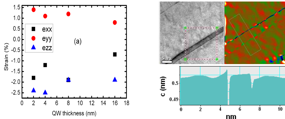
Figure 2.22: (a) : strain extracted from the Raman measurements. We recall that y is the growth axis and z the c -axis. (b) : TEM analysis (area in the dotted square of (a)) of the lattice parameter along the c -axis on the thinner quantum wells (2 nm). One sees that GaN is matched on AlN along this direction. The color plot represents the local lattice parameter and the graph its variation along the growth axis (Note that the sharp features at the interfaces are artifacts [142]). No variation is observed at the GaN/AlN interface.
