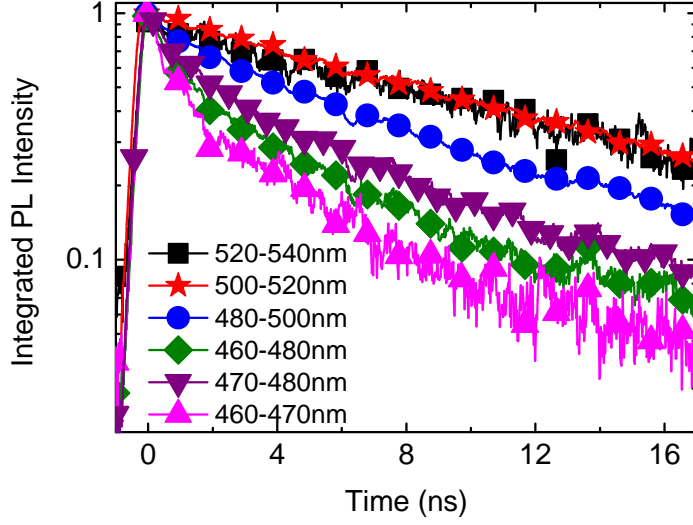
Figure 5.5: TRPL at low temperature on an unprocessed part of the sample in order to characterize the decay times distribution of the active region. The repetition rate is around 1 MHz and the spectrum is taken with a 20 ns window. In this configuration the temporal resolution is in the 400 ps range.
