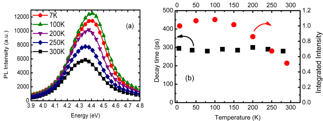
Figure 3.15: (a): temperature dependence of the luminescence of quantum dots embedded in nanowires. (b): temperature dependence of the integrated intensity, extracted from (a), and of the decay time.
