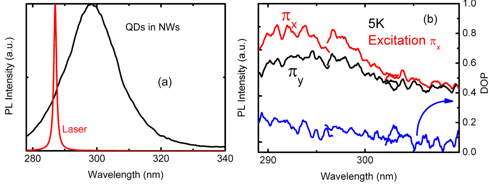
Figure 6.12: (a) : principle of the experiment. The spectrum of luminescence presented is recorded under non resonant excitation. (b) : low temperature photoluminescence spectra under quasi-resonant linearly polarized excitation at 287 nm. The degree of polarization (DOP) and its energy dependence evidence the optical alignment.
