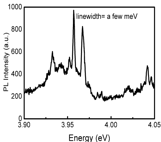
Figure 2.12: CL at low temperature on an unprocessed sample of wires. The linewidths are as narrow as 2 meV.
