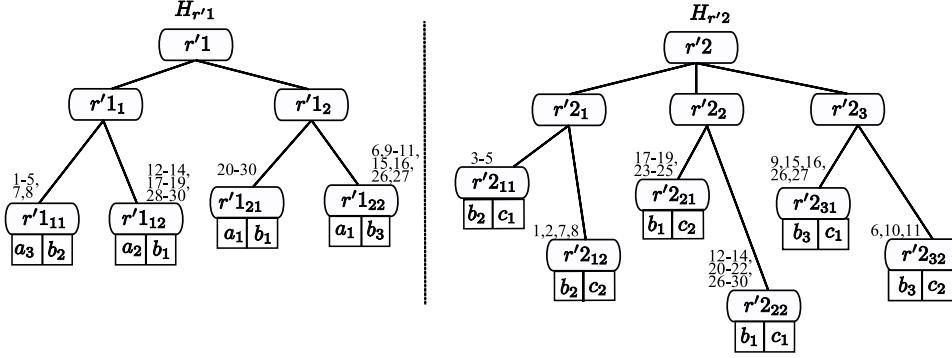
Figure 3.4 – H_{R'_1} and H_{R'_2}
