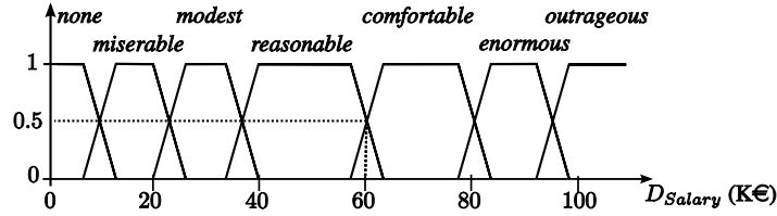
Figure 1.8 – An example of fuzzy partition defined for the attribute Salary
