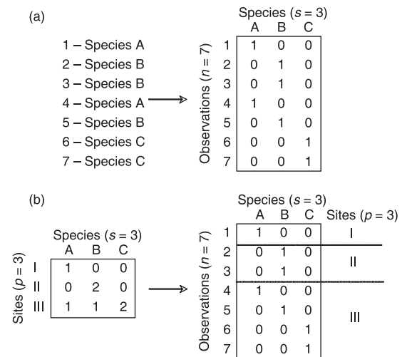
Fig. 1 (a) From a list of n = 7 individual observations of s = 3 species to a n \times s table of species occurrences, \mathbf{Y} . (b) From a table of species abundances of s = 3 species in p = 3 sites that sums to n = 7 observations, to a n \times s table of species occurrences partitioned according to p sites.
