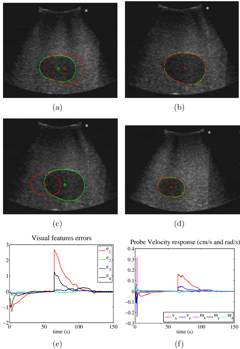
Figure 5.24: Experimental results with an ultrasound phantom using the model-free visual servoing method based on straight line estimation (the current contour is in green and the desired one in red): (a) Initial and first target image - (b) First target reached after visual servoing - (c) A second target image is sent to the robot - (d) The second target image is reached after visual servoing - (e) Visual error time response (cm, cm, rad, cm)- (f) Control velocity applied to the probe.
