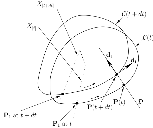
Figure 4.4: Image contour 3D evolution with a corresponding tangent straight line \mathcal{D} . In the 3-D space, the contour lies on the surface of the observed object. Contour \mathcal{C}(t) is extracted from the ultrasound image at time t , while \mathcal{C}(t + dt) is extracted at time t + dt after the probe had performed an out-of-plane motion. Contour's first point \mathbf{P}_1 at time t and that at time t + dt are indicated. They correspond to the intersection of X axis of the centered image frame with the contour, respectively at time t and at time t + dt . The X axis of time t is denoted X_{[t]} , while that of time t + dt is denoted X_{[t+dt]} .
