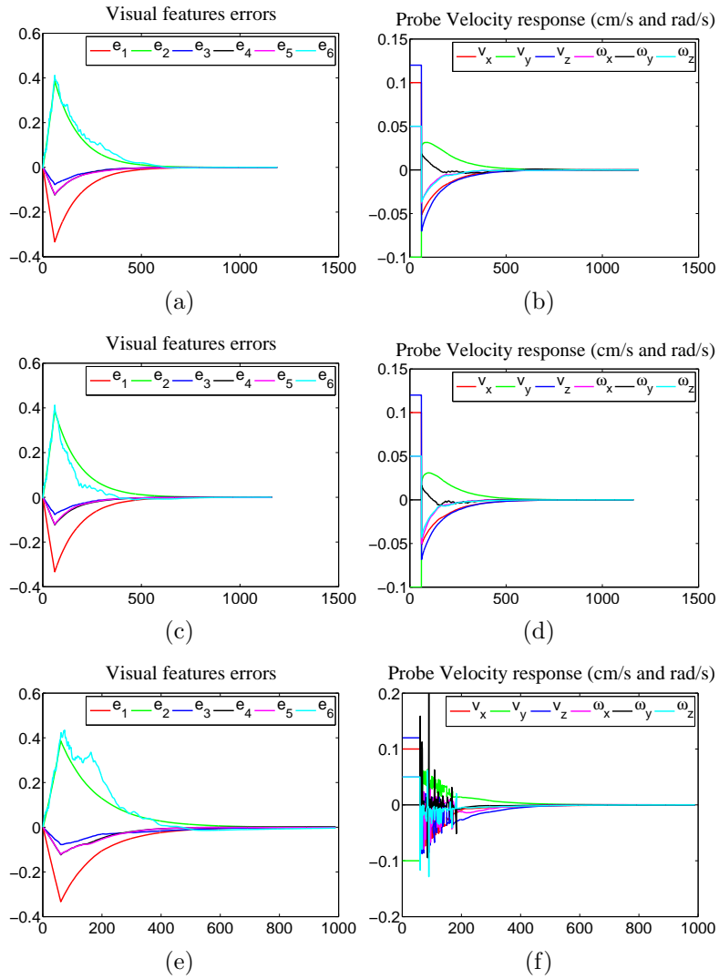
Figure C.19: Comparison of the performances obtained with the model-free servoing method that uses the quadratic surface-based estimation (Fig. C.17, that are also reported here on the two figures at the bottom) to those obtained with the two methods that use respectively the straight line- (top) and the curved line-based estimation (middle).
