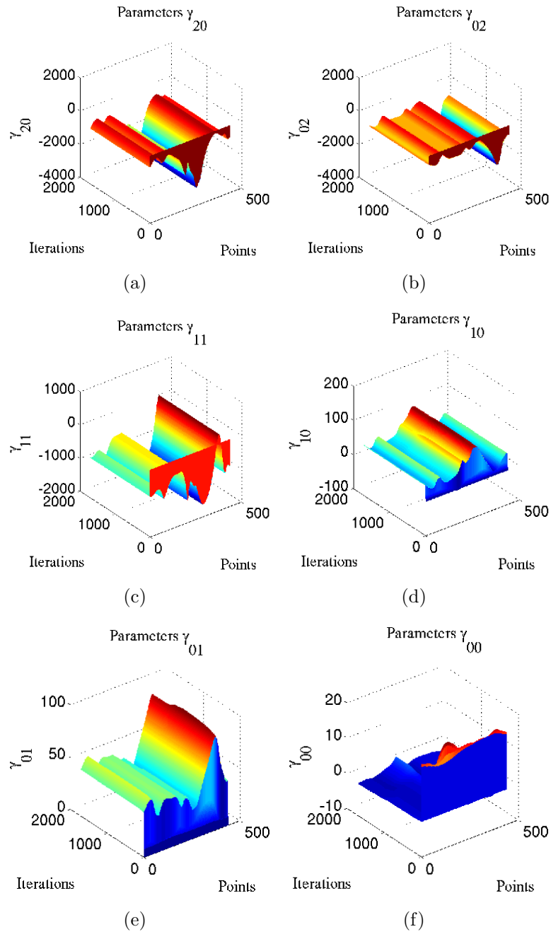
Figure C.14: Estimated Parameters \hat{\Theta} corresponding to the results shown on Fig. C.13.
