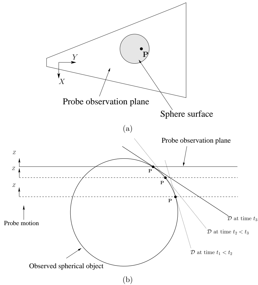
Figure 4.5: Evolution of estimated 3-D straight line for the case a 2D ultrasound probe is interacting with a spherical object. (a) Upper sight showing point P lying on the sphere surface, both being observed by the probe planar beam - (b) Transverse sight: the probe is performing an out-of-plane motion by moving along its Z axis, while at the same time straight line \mathcal{D} continually adjusts its orientation to remain tangent to the sphere surface at P .
