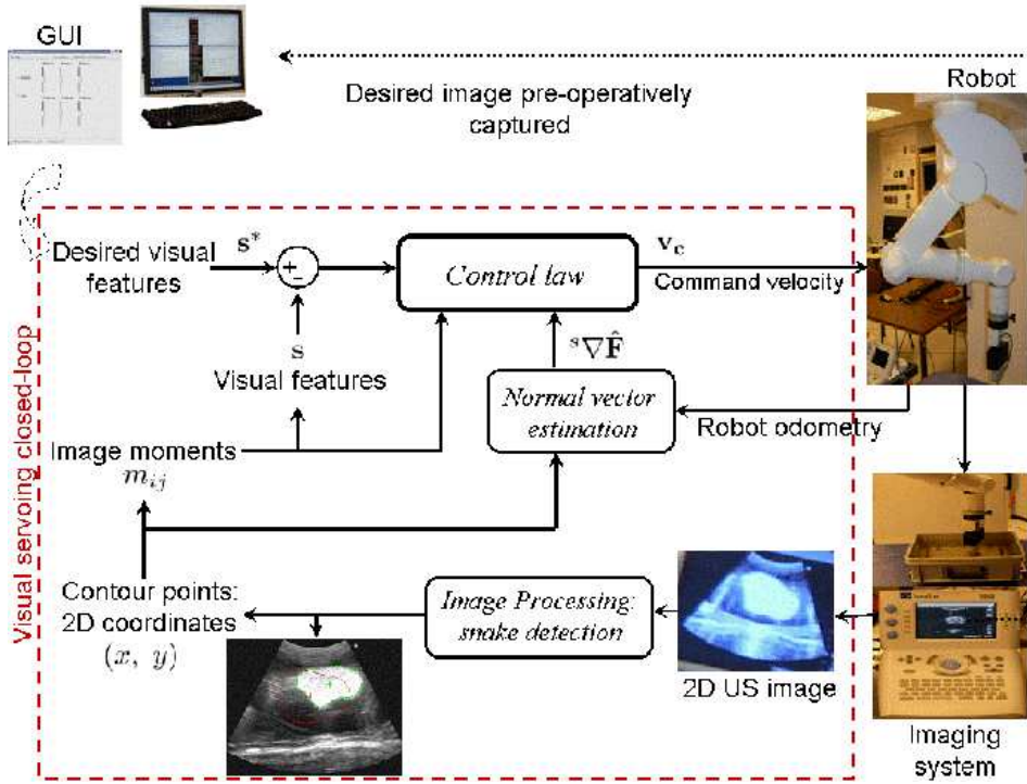
Figure 5.21: Architecture of the model-free servoing method, where the different involved steps along with the corresponding data flow, up to hardware setups, are presented.
