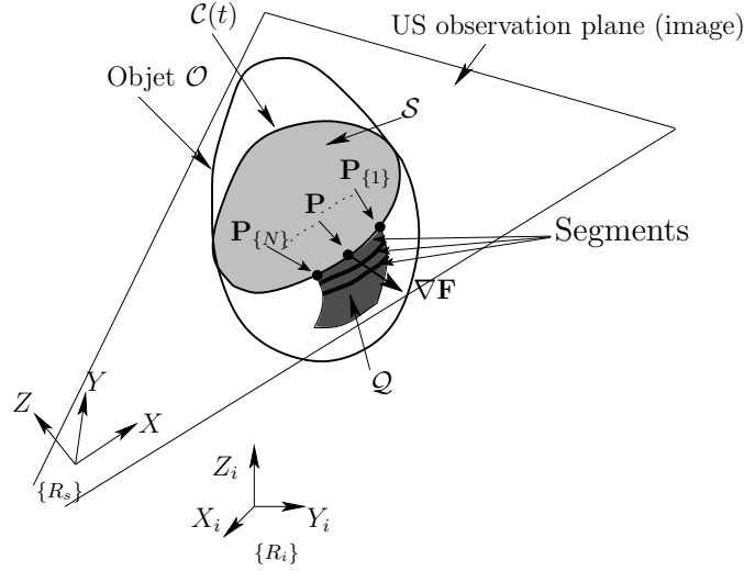
Figure 4.9: Quadric surface \mathcal{Q} that, ideally, should exactly fit the local surface surrounding point \mathbf{P} . The current observed segment is also shown, where its starting point \mathbf{P}_{\{1\}} and ending one \mathbf{P}_{\{N\}} are indicated on it. The segment is centered on \mathbf{P} .
