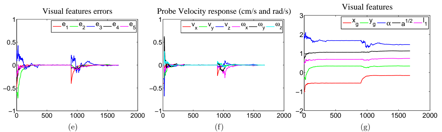
Figure C.11: Model-free visual servoing using the straight line-based estimation method performed on a realistic ultrasound 3D volume - (a) Initial image, whose section is contoured with green, captured right before the servoing is launched. The contour, of the first target image section, is displayed in red and is superimposed on the image - (b) The first target is automatically reached, where the observed (green) and the desired contour (red) now become superimposed - (c) The second target (red) is ordered - (d) The second target is automatically reached. The visual features and their corresponding errors are in (cm, cm, rad, cm, cm).
