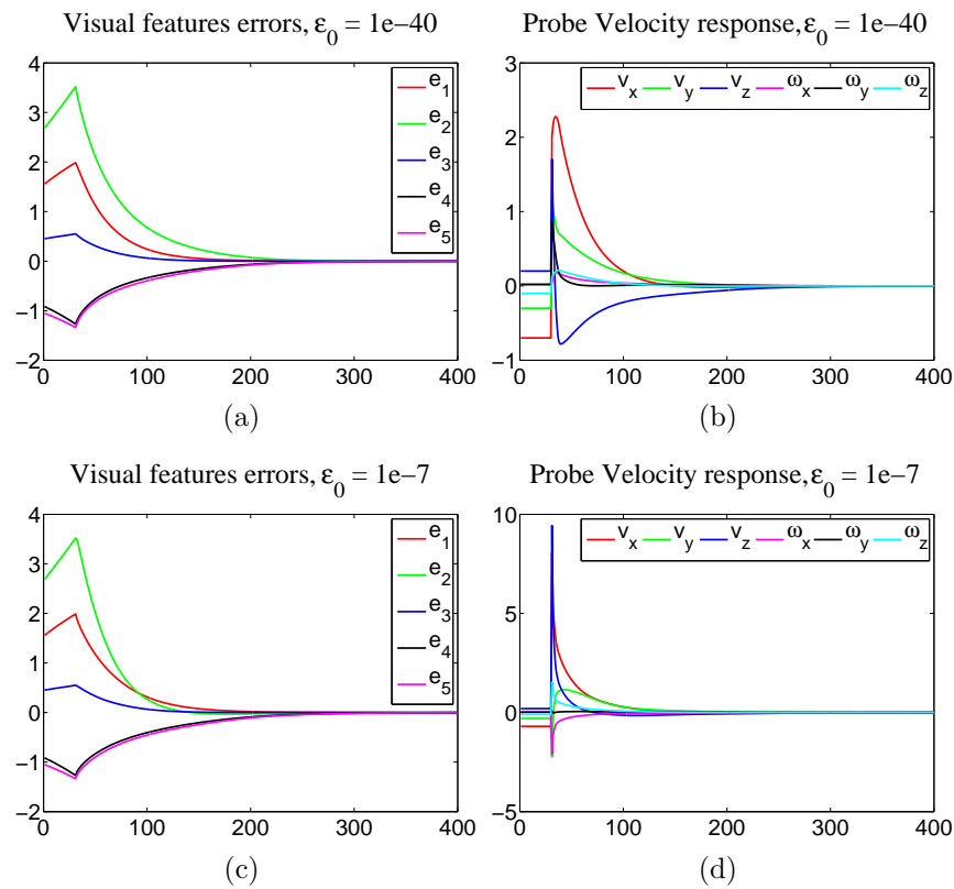
Figure C.6: Results obtained by employing the model-free visual servoing using the straight line -based estimation for different values of the parameter \epsilon_0 . The visual features errors are in (cm, cm, rad, cm, cm), and the probe velocity is in (cm/s and rad/s).
