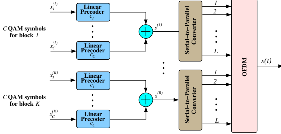
Figure 2.7: LP-OFDM single user transmitter.
