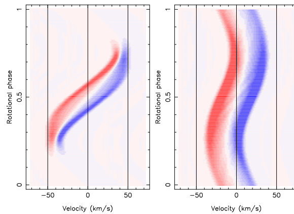
(a) champ radial
