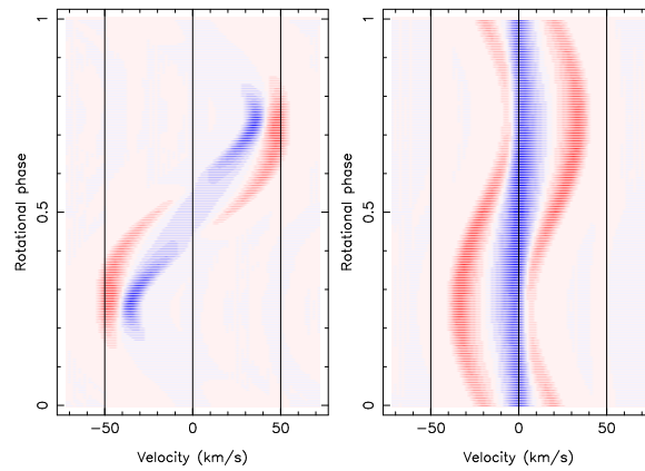
(c) champ azimutal
