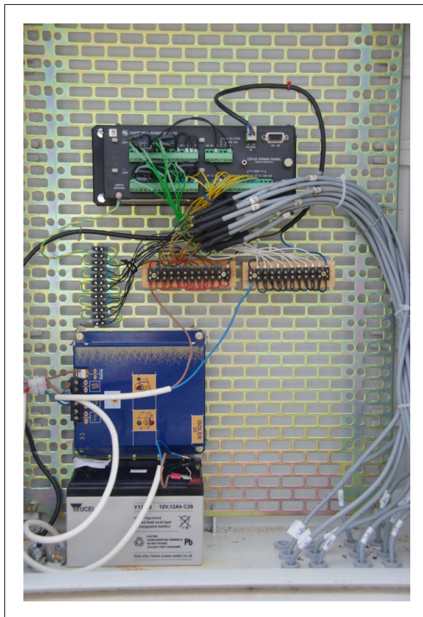
FIGURE 4.2 – Panneau d'acquisition
