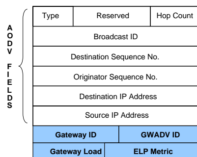
FIGURE 2.16 – Format of the GWADV packet of Gateway Selection Scheme
