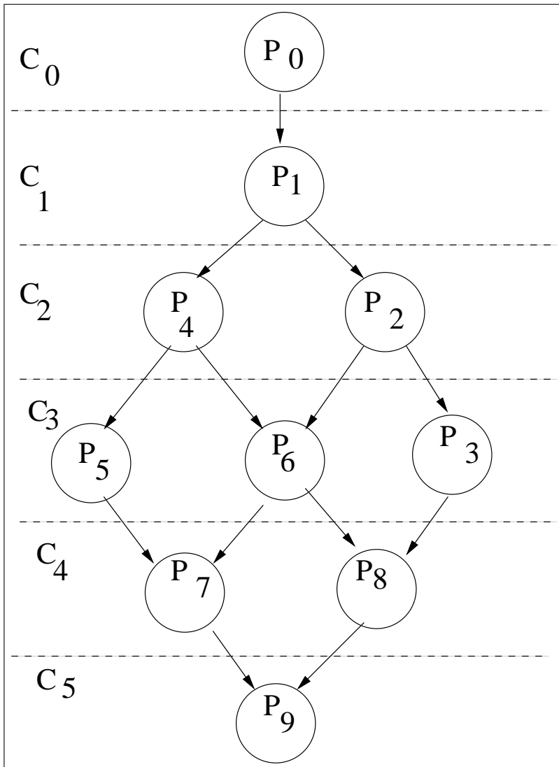
Figure 4.7 – Graphe des partitions
