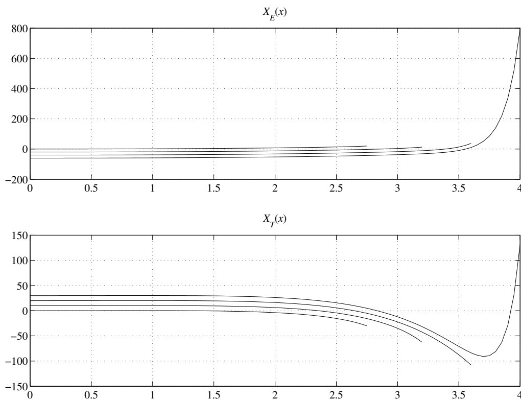
Figure 4.1: The X_E and X_T functions for different values of the upper boundary of integration x_{\max} = v/v_e\sqrt{2}e = 2.8, 3.2, 3.6 and 4.0 , and for an ion charge number Z=1 . The X_E 's are shifted by -20 with each other, the X_T 's are shifted by +10 with each other, the reference curves (i.e. not shifted) are for x_{\max} = 2.8
