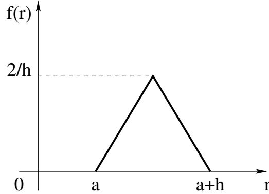
Figure 1.4: The synthetic triangle function with parameters a = 2 and h = 3
