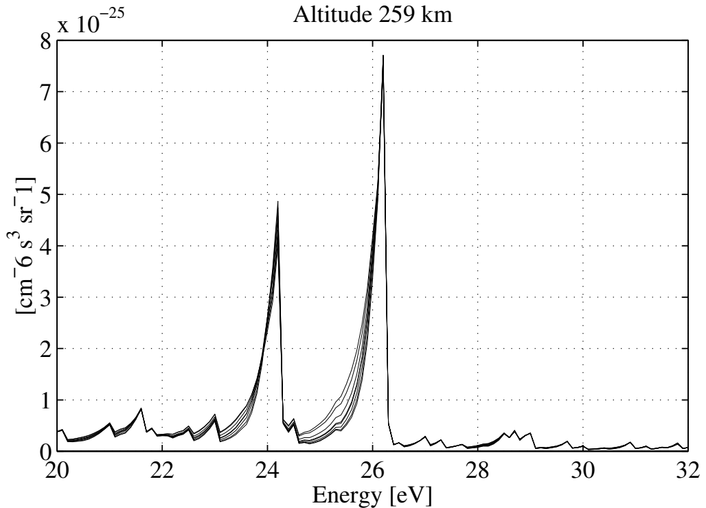
Figure 1.7: The angular supra-thermal distribution, plotted in the energy range 20–32 eV, used to perform the tests shown in Figures 1.8 and 1.9. The distribution was calculated with an eight-stream run over Tromsø in July 1996 at 12:00 UT with a F10.7 index of 80 and an A_p index of 15. The eight curves correspond to the eight angles of the double-Gauss quadrature
