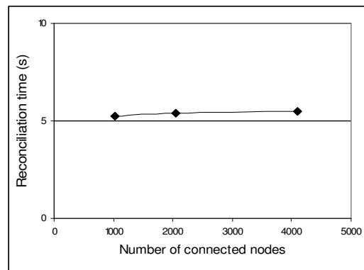
Figure 52. Reconciliation time varying the Nb-Nodes
