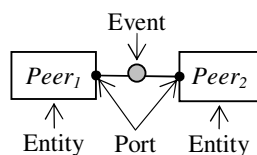
Figure 40. SimJava system
