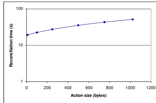
Figure 48. Reconciliation time varying action size
