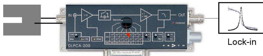
Figure 2.16: Experimental setup for measuring the displacements of the TF's prongs.
