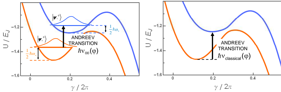
Fig. 6.8. Left: Scheme of the ground-state to ground-state transition \hbar\nu_{00}(\varphi) . The ground eigenstates in each potential |\psi_-^0\rangle and |\psi_+^0\rangle are shown as Gaussian curves in each well. Right: Scheme of the transition in the almost classical case \nu_{\text{classical}}(\varphi) .
