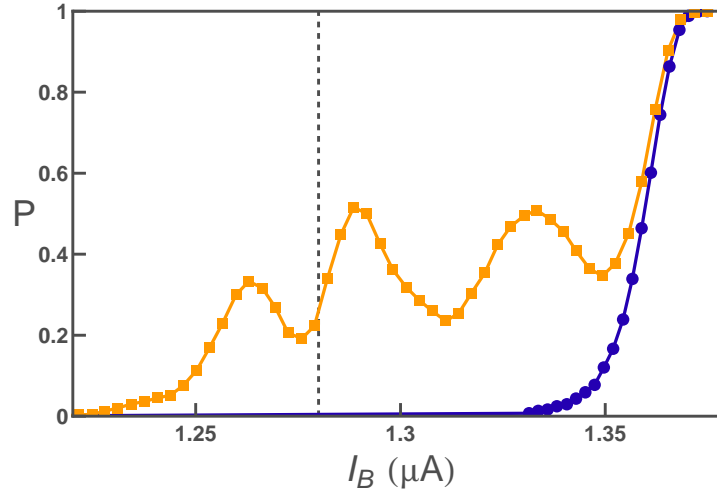
Fig. 6.24. Symbols: Escape probability without (circle) and with (squares) microwave excitation at 24.3 GHz. Close to \varphi = 0 , the curve does not present just a single bump as in Fig. 6.21, but several distinct bumps. Dashed line: Predicted position in bias current where the excitation frequency matches the high-frequency mode, using the parameters extracted from Fig. 6.21.
