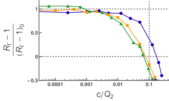
Fig. 3.16. Symbols: Rate asymmetry at s = 0.92 as a function of c/Q_2 for three values of effective quality factor ( Q_{\text{eff}}=2, 5 , and 8 (circles, squares, and triangles)). Dashed vertical line: plasma frequency at this bias current.
