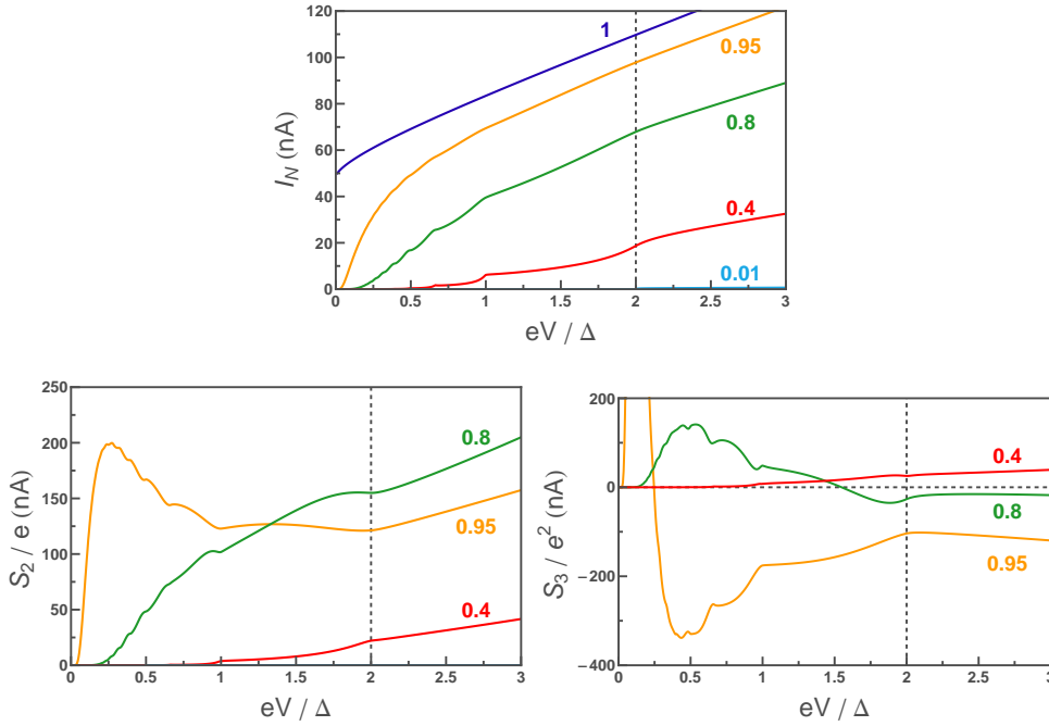
Fig. 4.47. Top: Current-voltage characteristics of a superconducting channel, for various transmissions. Left: Second moment of noise (the curves for the transmissions 0.01 and 1 are not shown, since the result is just very close to 0 everywhere). Right: Third moment of noise. (All curves were presented in [40]. Courtesy of J.C. Cuevas and W. Belzig)
