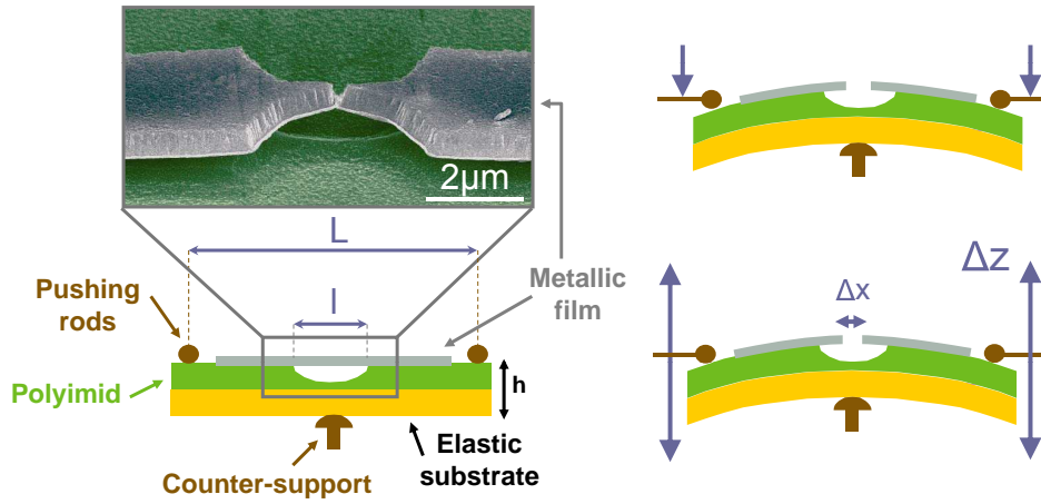
Fig. 5.7. Principle of the microfabricated break-junction technique. A thin microfabricated metallic bridge, suspended over a distance l \simeq 2\mu\text{m} , is broken by bending the elastic substrate (of thickness h \simeq 500\mu\text{m} ) on which it was fabricated. The bending is achieved using a three-points mechanism, with a central counter-support and two pushing rods separated by L \sim 16\text{mm} . A relative vertical displacement \Delta z of the pushing rods, corresponds to a change of the distance between the electrodes \Delta x \simeq r\Delta z where r = 6hl/L^2 is of the order of 10^{-4} in typical experiments. \Delta z can be easily adjusted at the micron level, and the displacement between electrodes \Delta x is therefore controlled at the level of 100 pm or better [19, 44].
