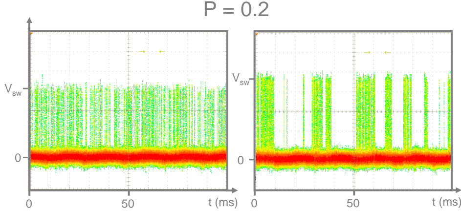
Fig. 5.21. Voltage across the Atomic SQUID as a function of time during a sequence of bias-current pulses ( 50 \mu\text{s} period). Each voltage pulse corresponds to a switching event. Left: at a flux value for which the P(s) curve is normal. Right: Similar measurement, at a flux value for which it displays a step, showing intermittency attributed to the dynamics of quasiparticle trapping and untrapping in the upper Andreev state.
