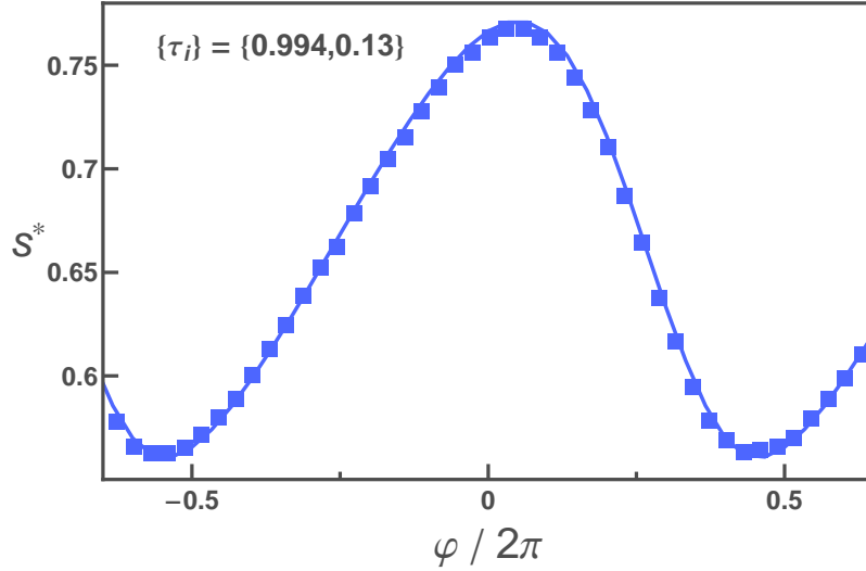
Fig. 5.18. Symbols: Measured modulation curve s^* at T = 350 mK, for the same contact as in Fig. 5.15. Solid line: Modulation curve calculated with the effective potential \langle U \rangle^I using T_{\text{eff}} = 378 mK (adjusted to fit the average switching current) and T_A = T_{\text{eff}} .
