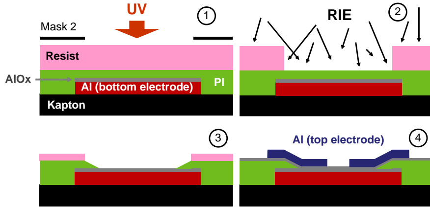
Fig. 7.6. Scheme for the fabrication of capacitor C_e for the SQUID sample. Red: bottom electrode (Al); grey: dielectric (AlOx); green: polyimide layer to protect the edges; blue: top electrodes (see text for details).
