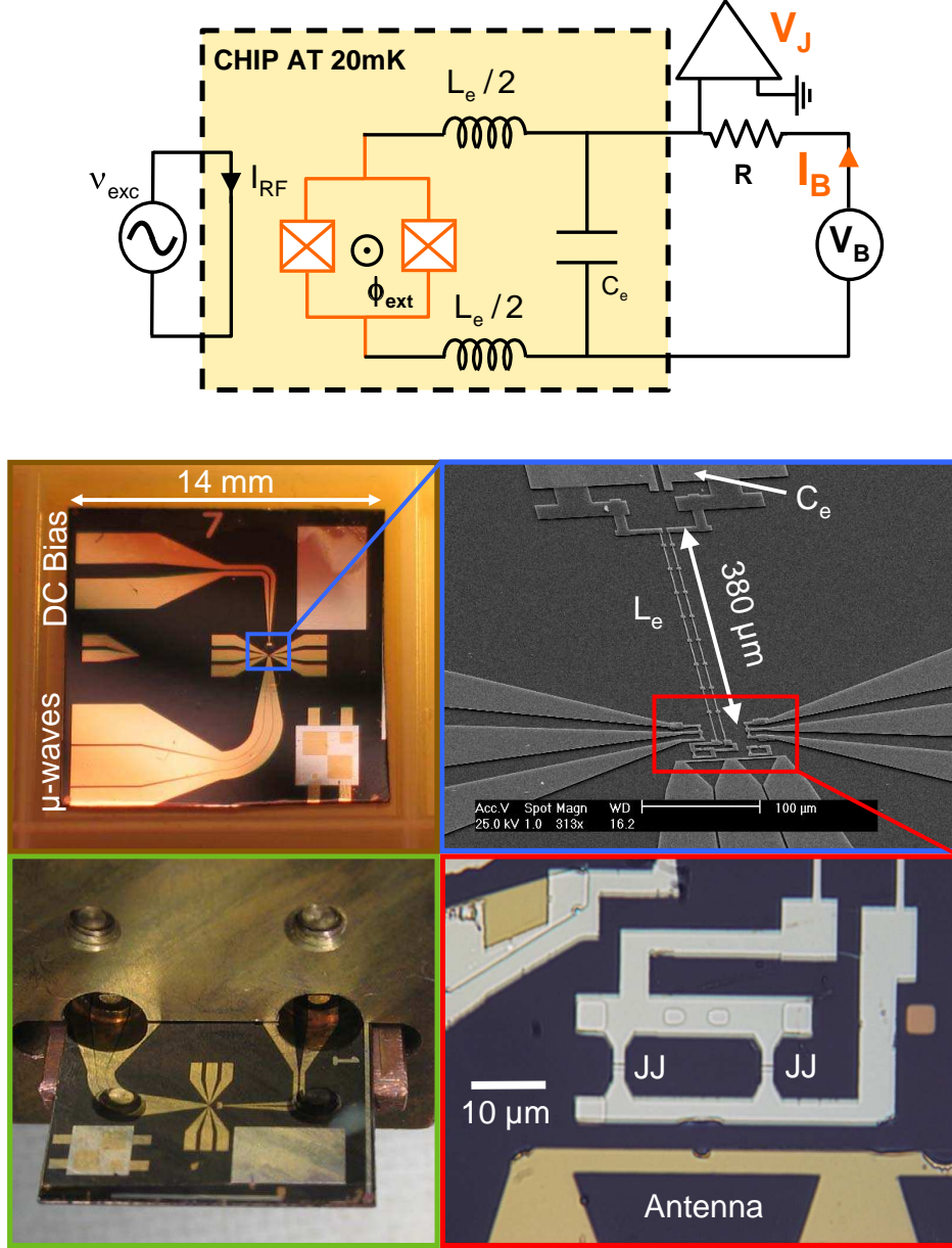
Fig. 6.15. Top: Schematic of the setup. A SQUID of two Josephson junctions of critical current I_0 \simeq 0.75 \mu\text{A} each is connected to an inductive environment made of L_e and C_e . An on-chip antenna is realized with a wire placed close to the loop, which is able to induce a flux at high frequencies. Bottom: Pictures of Sample SQUID, taken at large scale with a binocular (top left) and at smaller scale with an optical microscope (bottom right) or a SEM (top right). The bottom left panel shows the sample holder.
