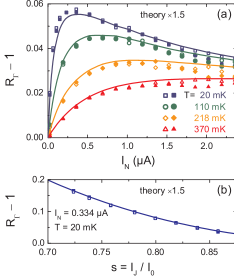
FIG. 3 (color online). (a) Rate asymmetry R_T - 1 as a function of current in noise source I_N for various temperatures T . Filled (open) symbols correspond to measurements with positive (negative) current through the JJ detector. Solid lines are theoretical predictions scaled by a factor 1.5. (b) Dependence of R_T - 1 on s = I_J / I_0 , at I_N = 0.334 \mu\text{A} , obtained with measurement pulses of various lengths. Solid line is theoretical prediction scaled by 1.5.
