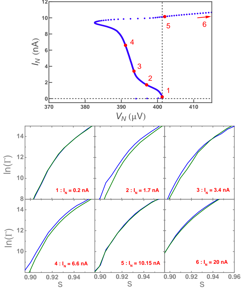
Fig. 4.42. Top: I(V) curve of the noise source around V_N = 400 \mu\text{V} , presenting strong non-linearities. The rate asymmetry was measured when biasing the noise source on this branch, for five different currents. Bottom: Evolution of the escape rate \Gamma as a function of the reduced bias current for the two signs of I_N , when the noise source is biased on the back-bending branch (the five first panels on top figure) and well above the superconducting gap, at a larger current, where the asymmetry is already sizeable, typically R_\Gamma - 1 \simeq 0.03 (panel 6, for comparison).
