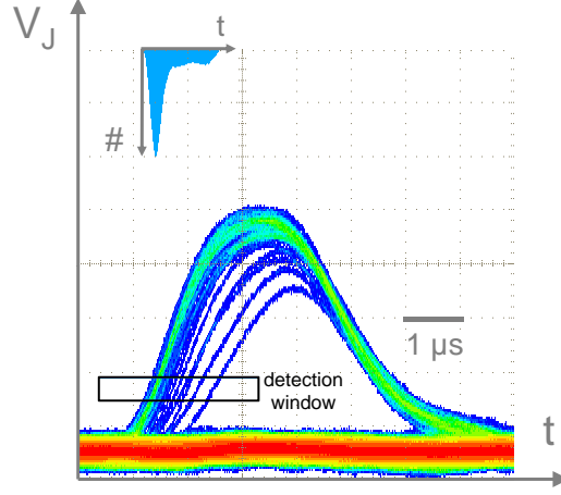
Fig. 4.44. Screen capture of the switching measurement when the noise source is biased on the supercurrent branch. On the top part, an histogram is shown as in Fig. 4.16 (beware that it is pointing downward). The pulse has been tuned to ensure that this histogram is flat when the noise source is not on the supercurrent branch (at low P ). Surprisingly, this is not the case anymore here.
