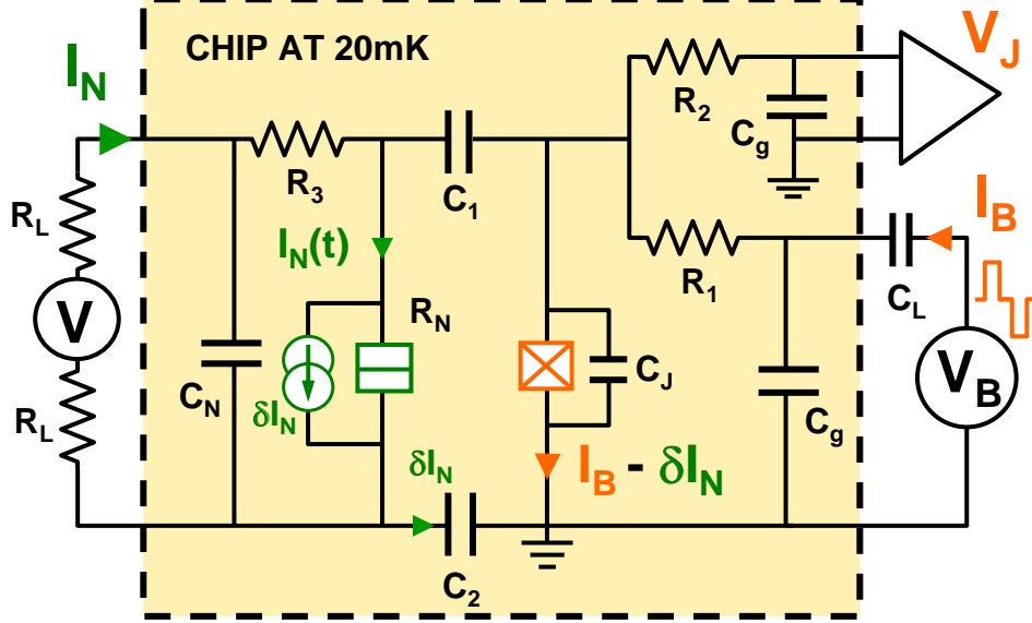
Fig. 4.7. Detailed setup of the experiment presented in this chapter and in [38]. Compared to the setup presented in Fig. 4.6, two coupling capacitors C_1 and C_2 are used. The voltage V_J across the junction monitors the switching to the dissipative state, through the resistor R_2 . Capacitor C_J lowers the JJ plasma frequency \frac{\omega_{p0}}{2\pi} close to 1.5 GHz at zero bias. Capacitors C_N and C_g shunt the impedance of the external connections lines at \omega_{p0} , therefore the admittance shunting the JJ is determined only by on-chip elements. Two large resistors R_L allow to fix the average value of I_N . C_L is a capacitor placed on the bias line at room temperature whose role is to avoid spurious offsets arising from thermoelectric voltages (see text for more details).
