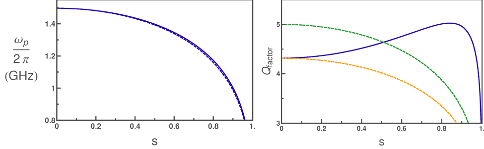
Fig. 4.29. Left: Plasma frequency of the junction obtained from the microwave simulation software at all reduced bias currents (solid line) compared to the approximation for the dependence in s of Eq. (4.27) (dashed line). Right: Quality factor of the junction obtained from the microwave simulation (solid line) compared to the approximate expressions Q_0 (1 - s^2)^{1/4} (bottom dashed line) and 5 (1 - s^2)^{1/4} (top in dashed line)
