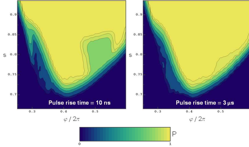
Fig. 5.24. Escape probability as a function of the external flux and the bias current measured on Sample AC2 for an atomic contact with transmissions \{0.999, 0.696, 0.275, 0.26\} . The escape probability is shown for two different rise times of the measurement pulse. The out-of-equilibrium effects tend to disappear for longer rise times.
