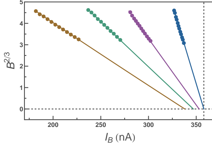
Fig. 4.19. Dots: B^{2/3} functions obtained from escape rate measurements performed for I_N = 0.011, 0.21, 0.52, and 1.15 \mu\text{A} from right to left. Solid lines: Fits using Eq. (4.19) and the exact expression of the barrier height from Eq. (2.14). The effective temperature is obtained from the slope, and the critical current is read from the intersection between the fit and the current axis. When I_N is increased, the absolute value of the slope diminishes, denoting the increase in effective temperature. But, unexpectedly, the extrapolated critical current also decreases, since all the lines do not cross at a single point on the current axis.
