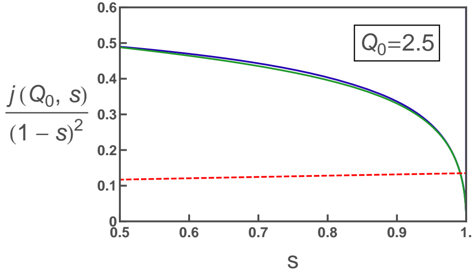
Fig. 2.14. Predictions for j(Q_0, s) at Q_0 = 2.5 , which corresponds to the experimental value in [37]. Solid line: Predictions of H. Grabert j_{\text{FullQ}}(2.5, s) (blue) and K. Glaum j_{\text{FP2}}(2.5, s) (green). Dashed line: Prediction j_{\text{Ad}}(s) from the adiabatic model presented in [65] used to perform a comparison with the experiment in [37], with r=1 .
