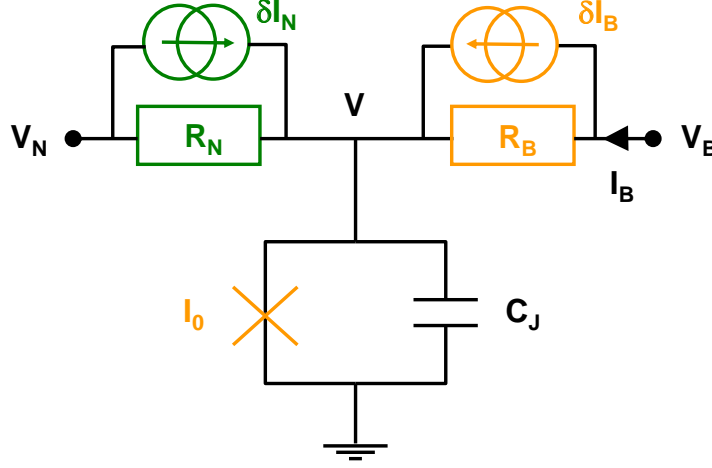
Fig. 2.9. Electrical setup considered in the theories addressing the effect of an asymmetric noise on the escape rate of a JJ out of the zero-voltage state. The junction is biased by a current I_B through a resistor R_B , which is a source of thermal noise \delta I_B . A noise source of impedance R_N produces additional, non-Gaussian fluctuations \delta I_N .
