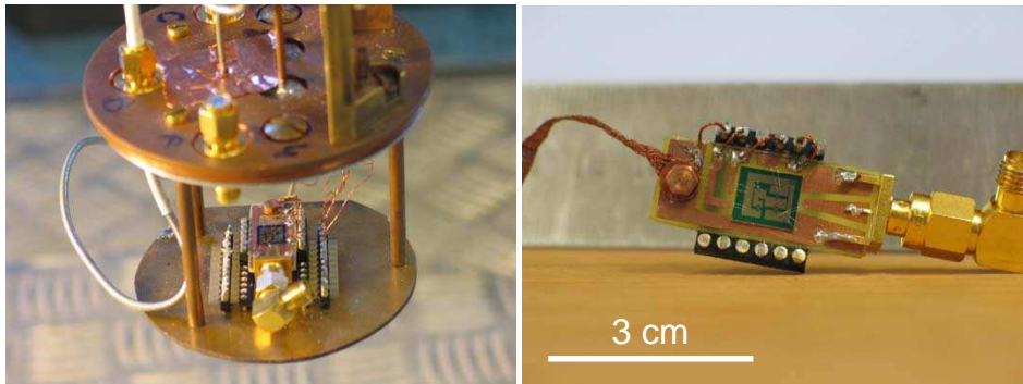
Fig. 8.1. Sample holder for the Samples JJD1 and JJD2.
