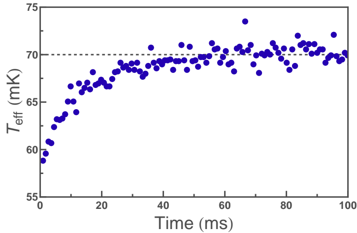
Fig. A.6. Rise of the effective escape temperature with the measurement time. Temperature is calculated from a local escape probability (obtained from the density of escape events in a period of time corresponding to 100 measurement pulses).
