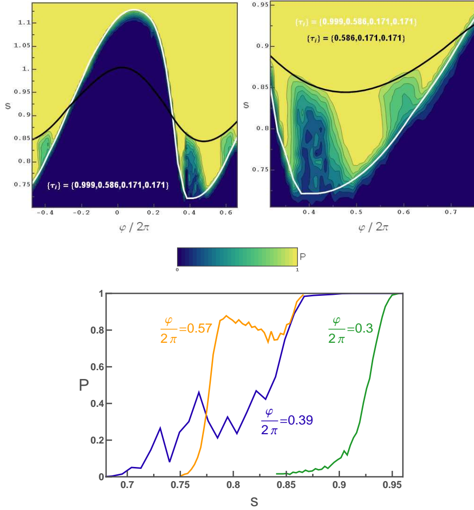
Fig. 5.19. Top: Escape probability as a function of the external flux and the bias current for Sample AC2, with an atomic contact of transmissions \{0.999, 0.586, 0.171, 0.171\} . The white line corresponds to the modulation curve calculated taking into account the contribution of the Andreev ground state of all the channels. The black line corresponds to the modulation curve calculated for \{0.586, 0.171, 0.171\} , i.e. excluding the contribution of the most transmitted channel. Bottom: Escape probability as a function of the reduced bias current for three different values of the applied flux.
