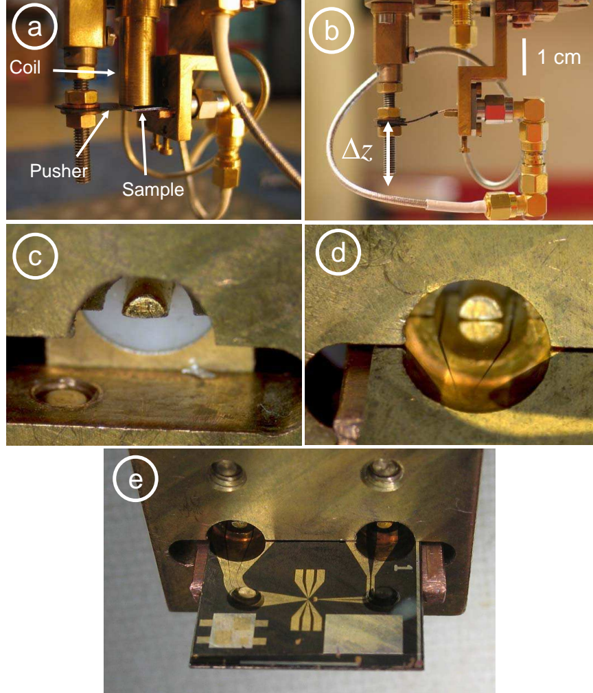
Fig. 8.3. Sample holder designed for Andreev states spectroscopy and used for the measurements on sample SQUID. (a,b) The sample (14 mm \times 14mm, 500 \mu m-thick Kapton substrate) is held tightly against two SMA launchers, by pushing with two screws a small piece of copper, also visible in (d) and (e) , on the back of the substrate. A small superconducting coil is placed in a copper electrostatic shield placed immediately above the sample (the coil is absent in (b) ). In (a) , the sample is not yet bent, in (b) it is noticeably strained. (c) SMA Launcher, without sample; one of the pushing screws shows out on the bottom left; (d) SMA launcher with sample: the pin contacts the central line of the coplanar waveguide on the sample; (e) sample in position (coil and pusher removed) The right launcher connects to the current bias line. The left to the microwave antenna.
