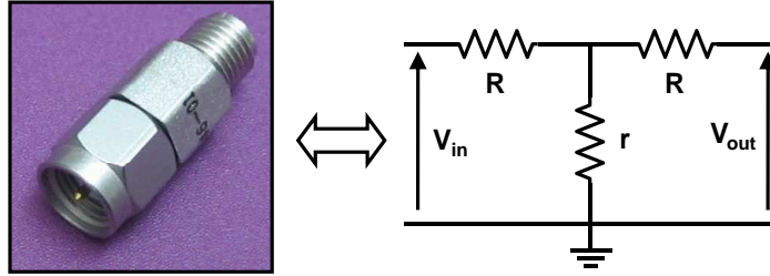
Fig. B.5. Model for an attenuator, with three resistances placed on a T.
