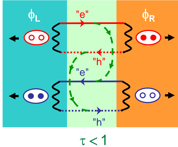
Fig. 5.4. Schematic representation of the scattering mechanisms in a short reflective channel. In addition to the Andreev reflection processes (black wiggly lines), a normal reflection process (green dashed lines) connects electron (hole) states traveling in different directions, thus mixing the two reflectionless states of Fig. 5.1. This gives rise to the "adiabatic Andreev states".
