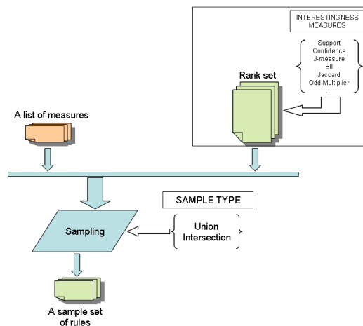
Figure 5.19: A process to compute a sample.
