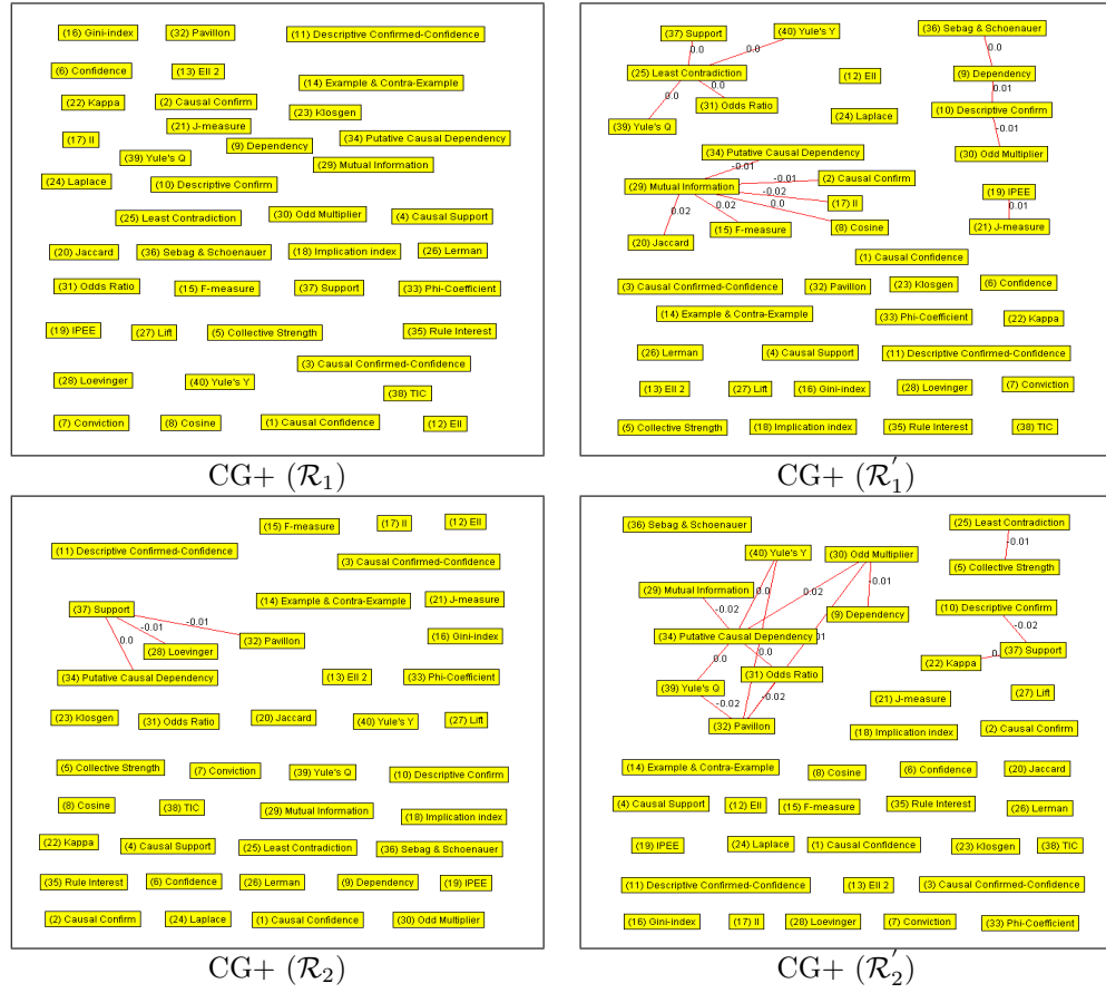
Figure 7.10: \overline{CG}^+ graphs with Spearman's coefficient.
