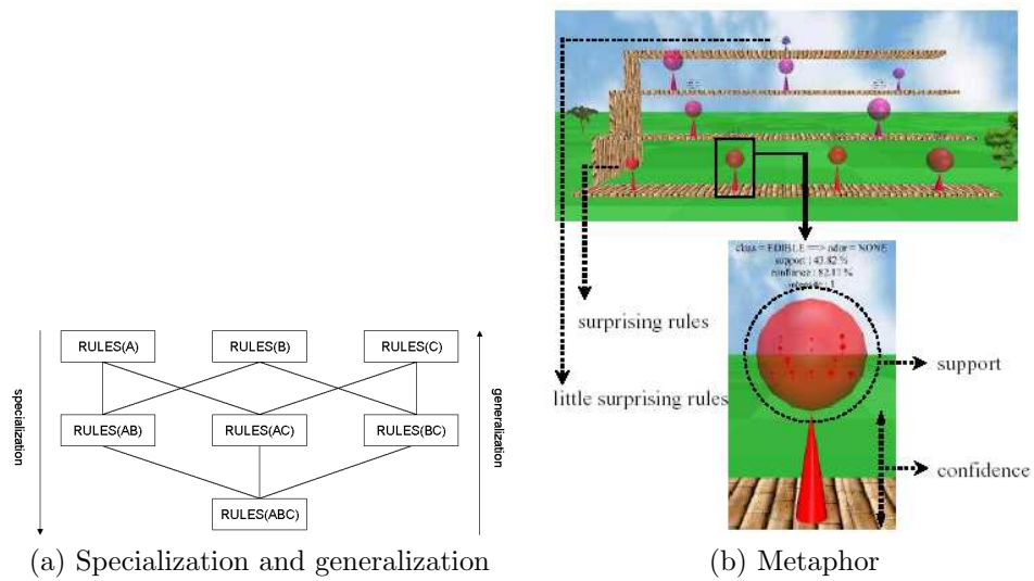
Figure 4.16: Visualization with the ARVis platform.
