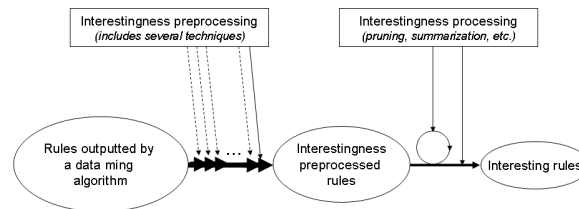
Figure 4.4: IPS in the interestingness process.
