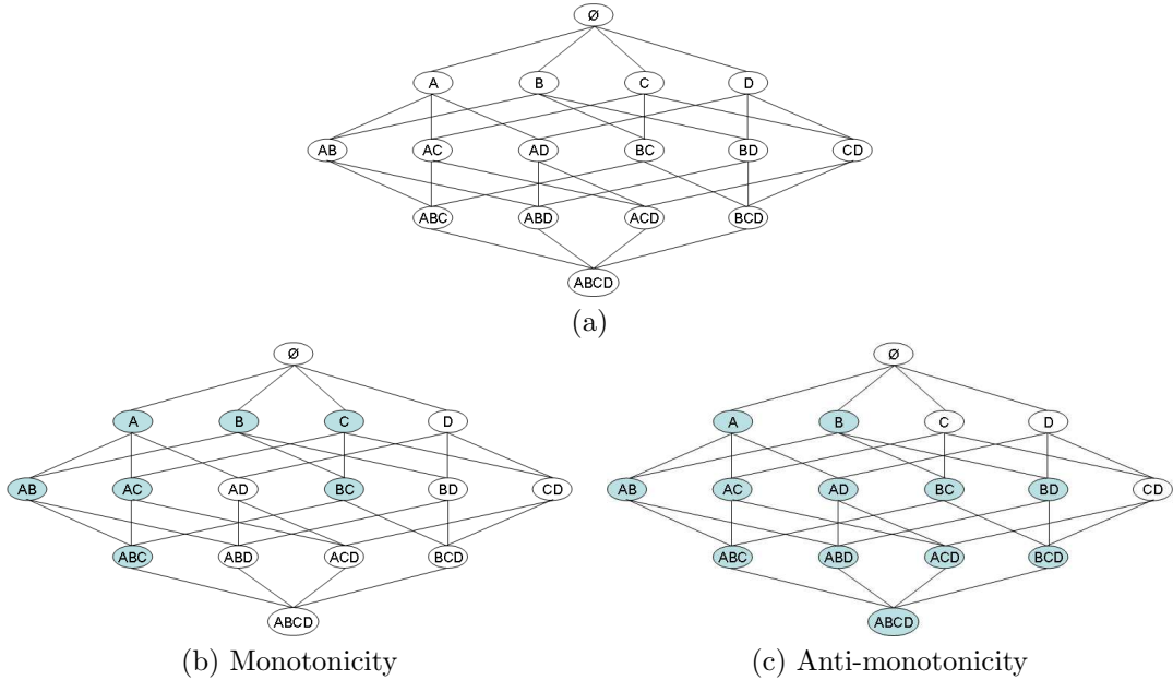
Figure 2.1: Lattice structure.
