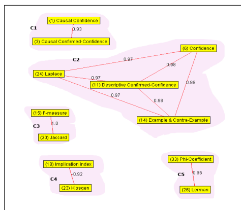
Figure 7.18: CG+ graph with Kendall's coefficient.
