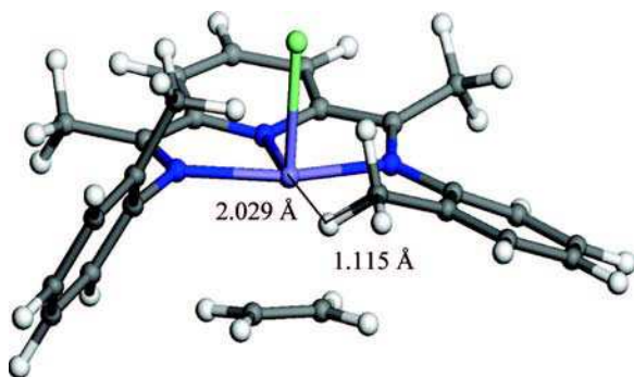
Figure 3. Octahedral structure of the singlet conformer [1(\text{II})\text{Cl-ax}]^{\dagger}\dots\text{anti}\perp .
