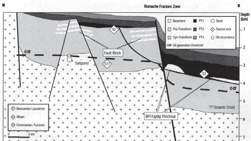
Fig. 18. Schematic cross-section: eastern Ghana play types. Deep-water plays are largely limited to Late Cretaceous basin floor fans.
