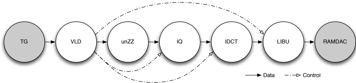
Figure 5.7: Original MJPEG algorithm.
