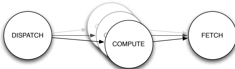
Figure 5.8: Modified MJPEG algorithm.
