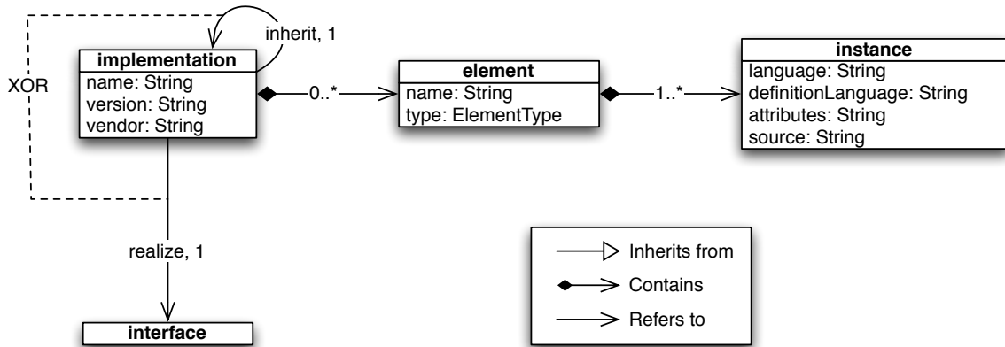
Figure 3.11: Class diagram of a component's implementation meta-model.
