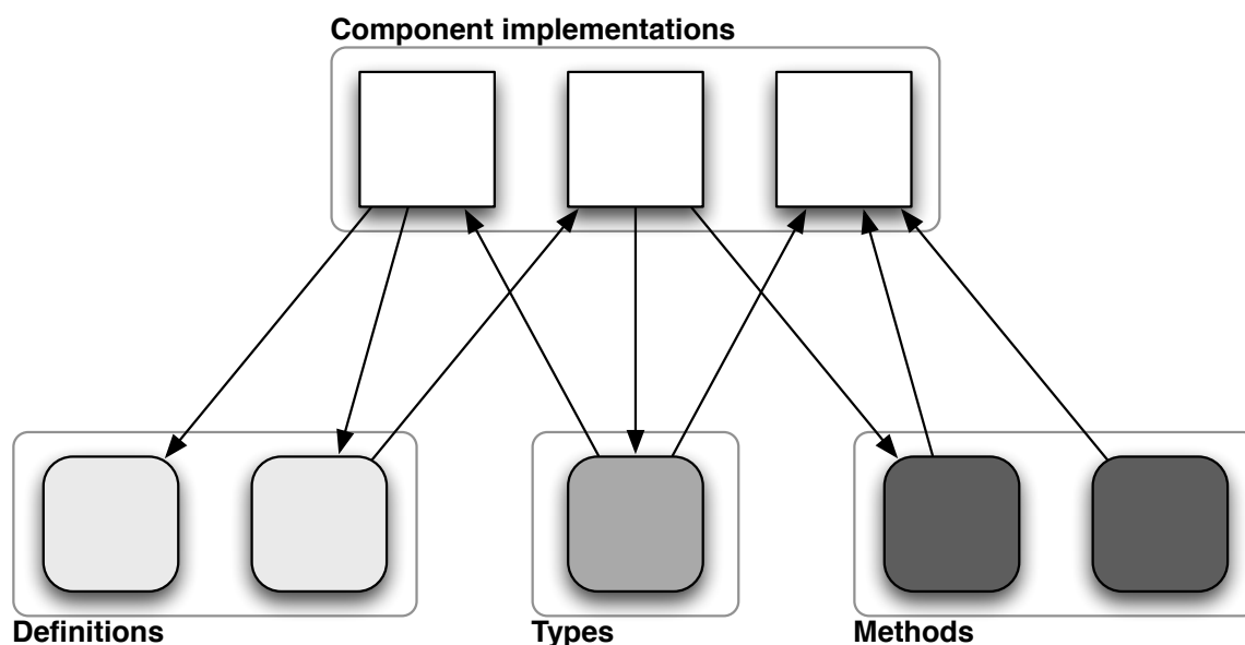
Figure 3.12: 4-partite digraph of the complete component set.
