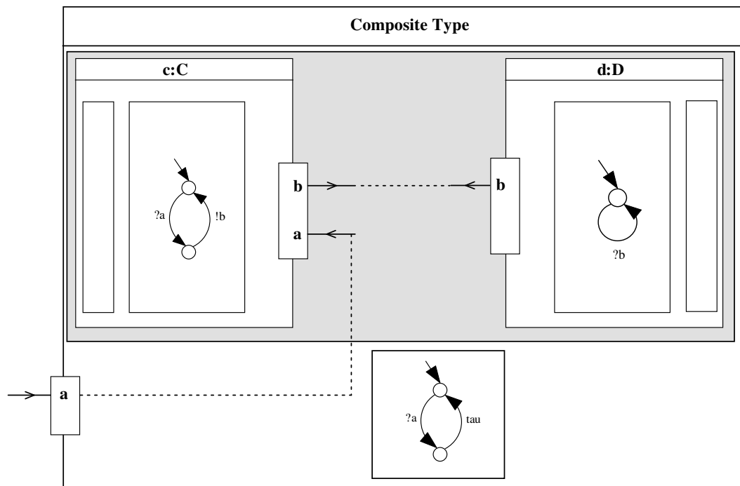
Figure 5.4: Composite Component Example.
