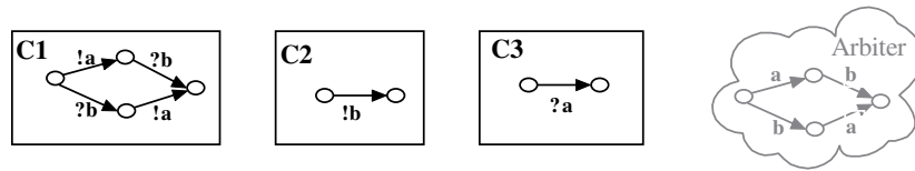
Figure 6.14: Component Protocols.
