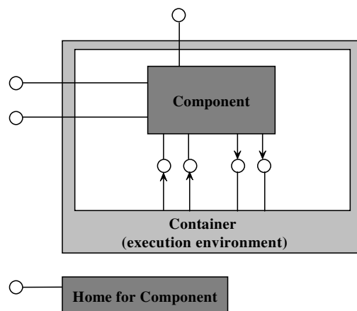
Figure 3.4: CORBA Component Model Execution Environment.
