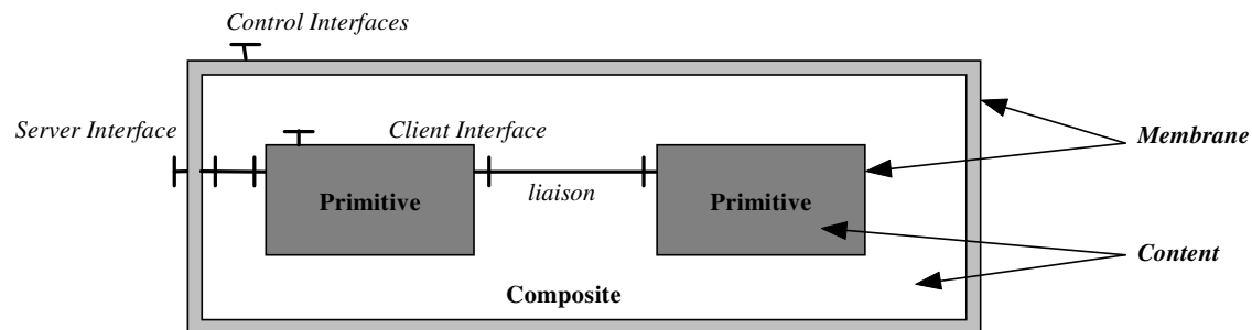
Figure 3.2: Fractal Architecture.
