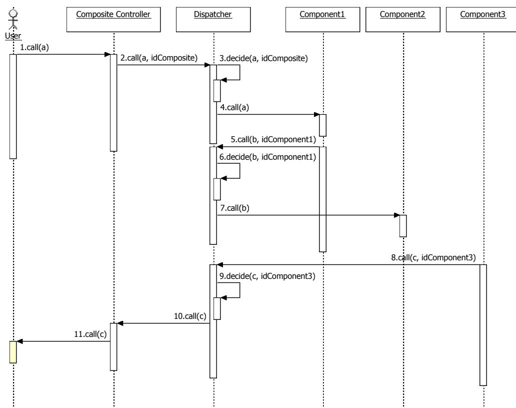
Figure 6.10: Composite Execution.
